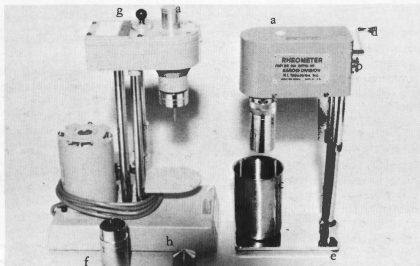
Figure 1. — Viscometers. A-C motor operated (left-side) and manually generated. (a) dial gauge, (b) low speed crank, (c) mud cup, (d) high speed crank, (e) stand, (f) outer sleeve, (g) speed control lever, and (h) inner bob.
