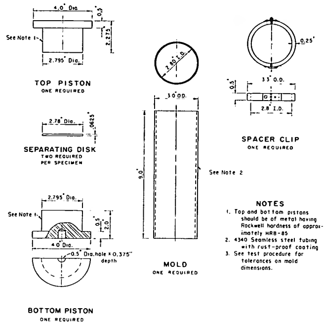
Figure 2. – Soil-cement compressive strength mold assembly.
