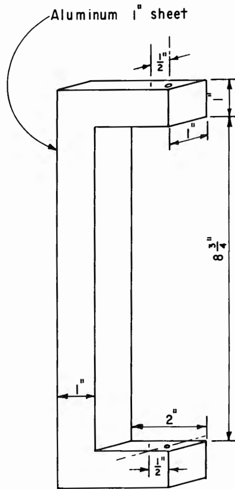
X1.4 - A dial gauge reference bracket for 8-inch permeability test.
