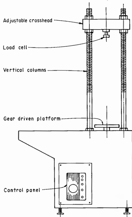
Figure 2. - Compression test machine.
