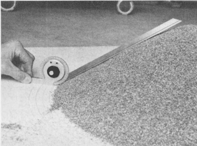
Figure 5. – Measuring the angle of repose of sand using a mechanic's vernier protractor.
