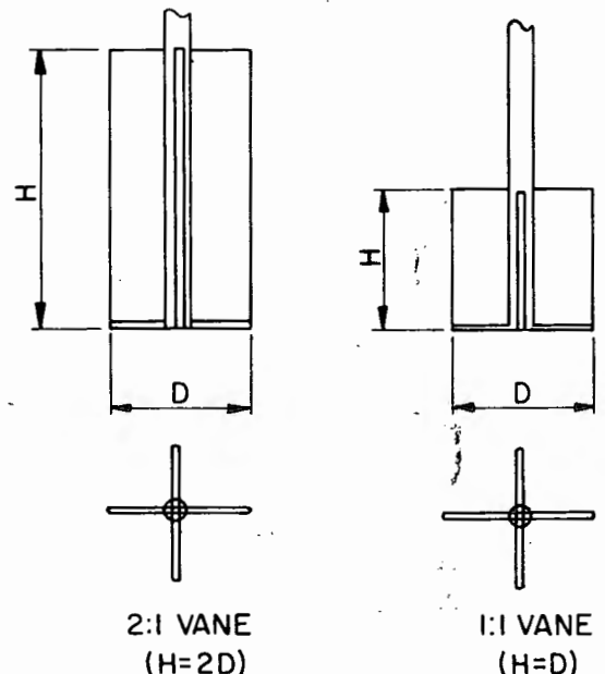
Figure 2. — Rectangular four-bladed vane.
