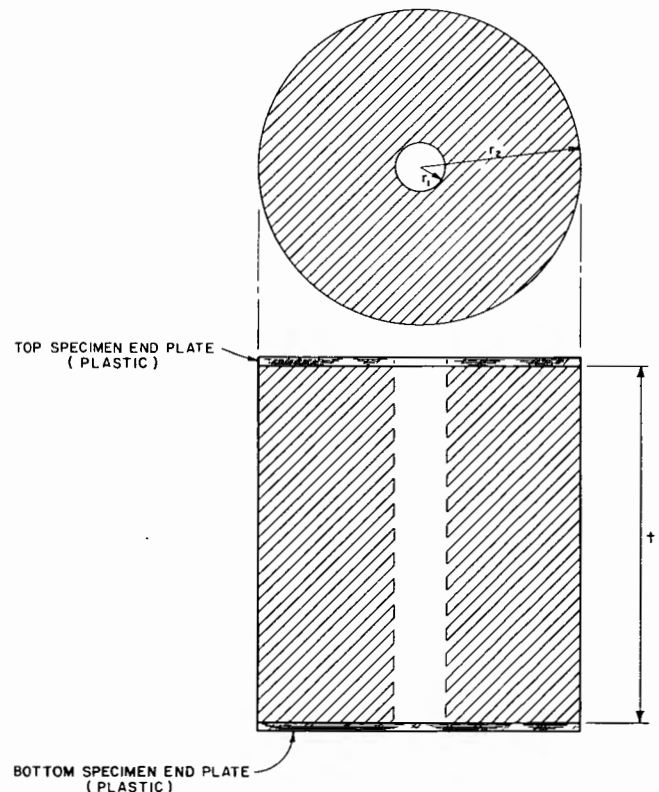
Figure 4. – Schematic showing specimen variables.
