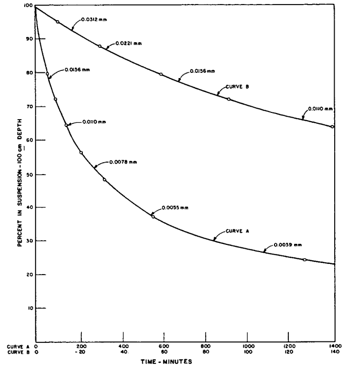
Figure X3.2 - Odén curve construction — Continued.
