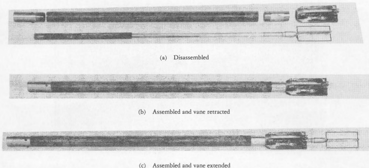
Figure 5. – Rotary cutting bit for use with the vane shear test apparatus
