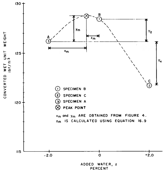
Figure 3. - Determining peak point of compaction curve, Y_2/Y_4 method.
