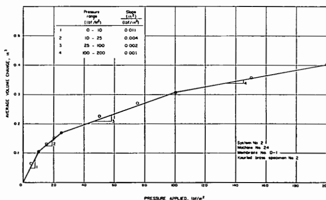
Figure 3. — Average volume change versus pressure applied — plot.
