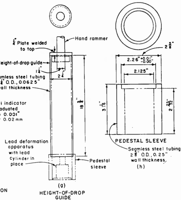
PEDESTAL SLEEVE AND HEIGHT-OF-DROP GUIDE FOR HAND TAMPER
