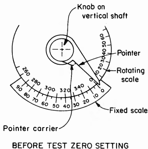
(b) Scales on laboratory vane shear device.
