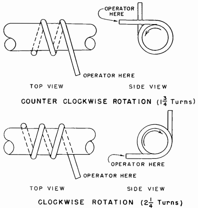
Figure 1. — Number of rope turns on cathead.
