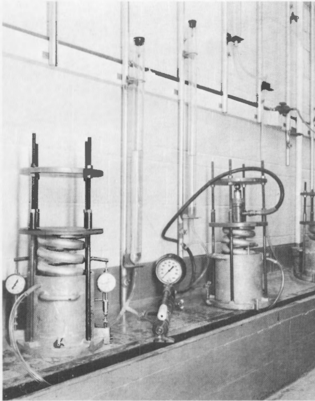
Figure 2. – An 8-inch-inside diameter permeability apparatus with hydraulic cylinder for applying normal pressure.
