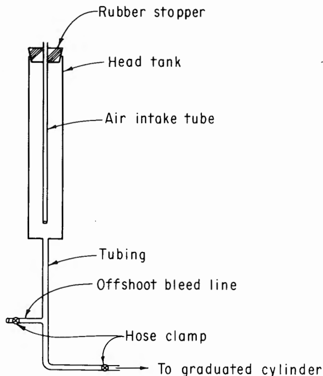
Figure 1. – Head tank calibration schematic.
