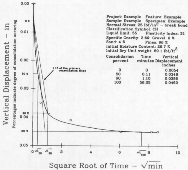
Figure 11. - Vertical displacement versus square root of time plot - example.
