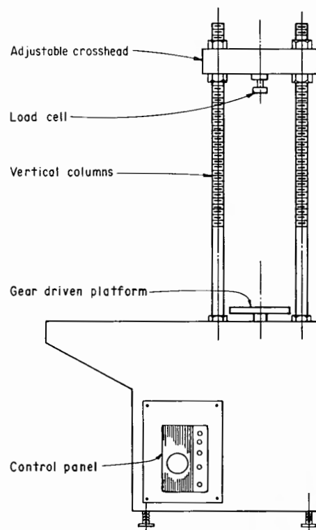
Figure 2. — Compression test machine.
