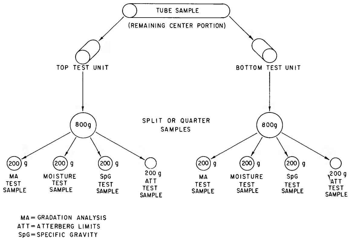
Figure 2. - Schematic of tube processing (dissimilar materials — minus No. 4).
