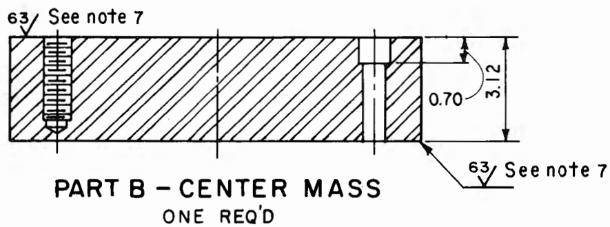
Figure X2.2. - Vibratory table calibration equipment — Continued. 101-D-647
