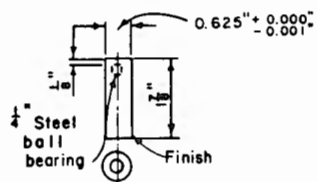
STRIKING PIN (a)
