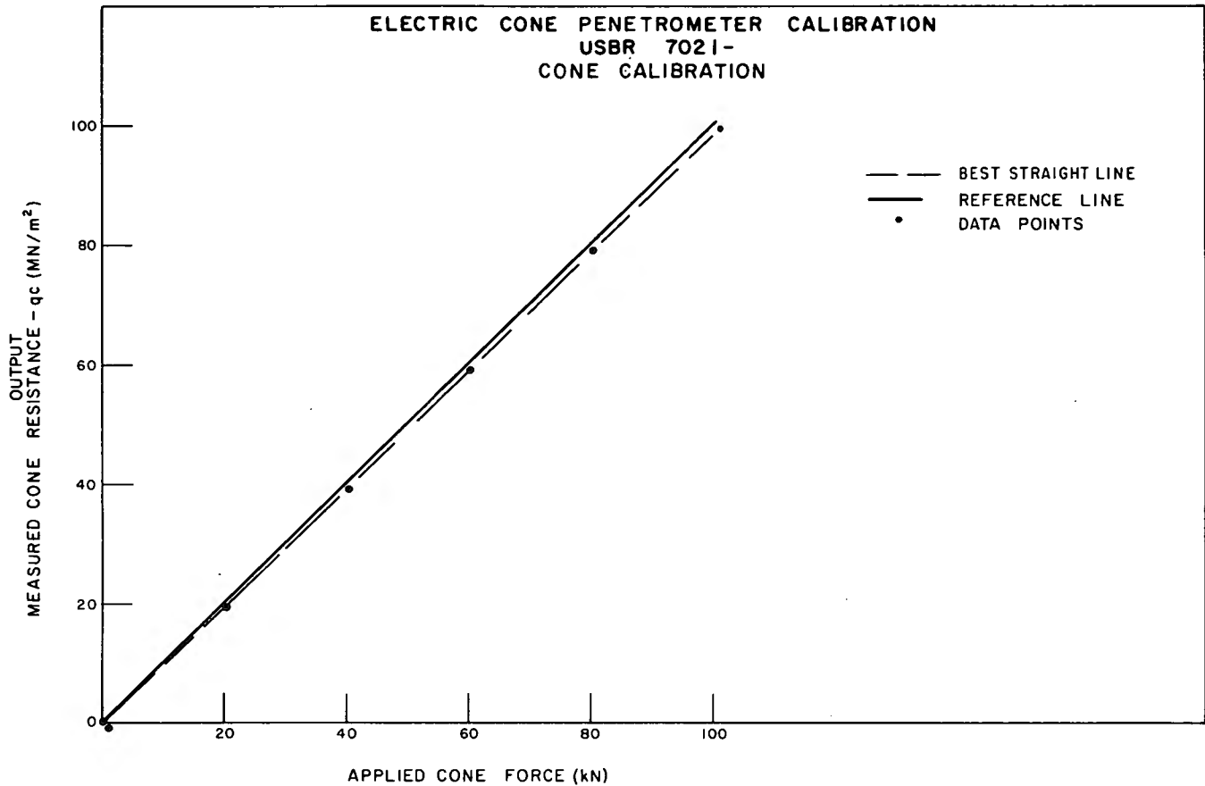
Figure A1.2. – Electric cone penetrometer cone calibration — example plot.
