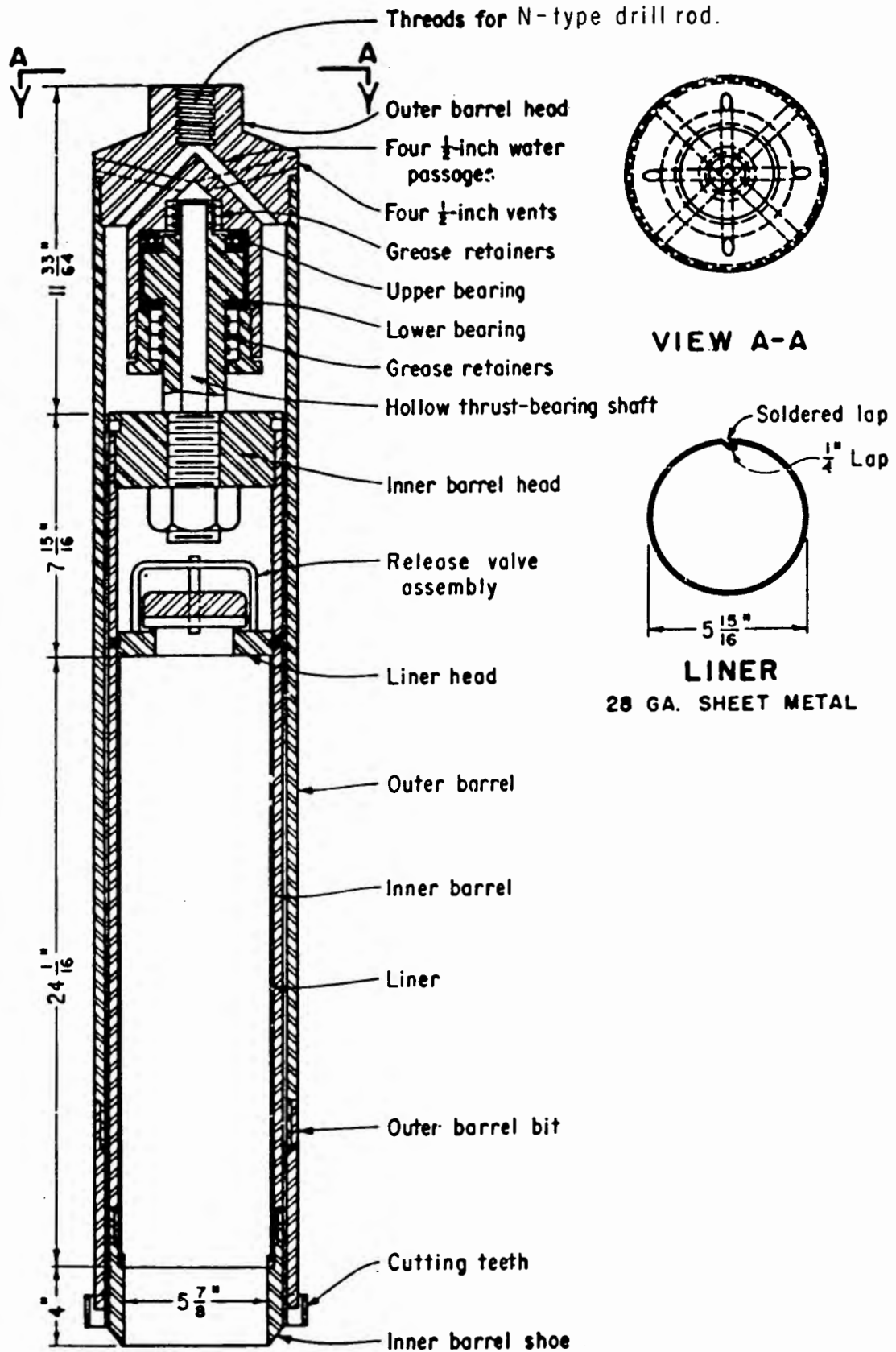
Figure 11. - Denison sampler (double-tube core barrel).
