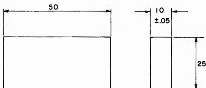
Figure 3. - Grooving tool (optional height-of-drop gauge attached) [ASTM D 4318].
