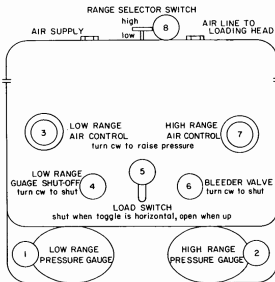
Figure 3. — Plan view of pneumatic load frame controls.
