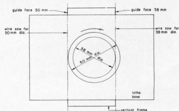
Figure X1.2. – Use of soil lathe guides for preparing either 1.5- or 2-inch (38- or 50-mm) diameter specimens.
