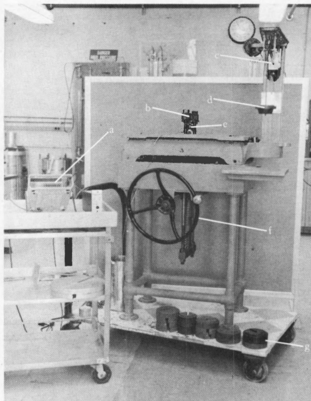
Figure 2. – Platform scale load frame. a) digital voltmeter, b) loading yoke, c) scale beam, d) scale beam hanger, e) load cell, f) wheel, and g) calibration masses.
