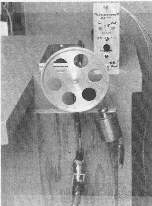
(b) Calibration assembly.
