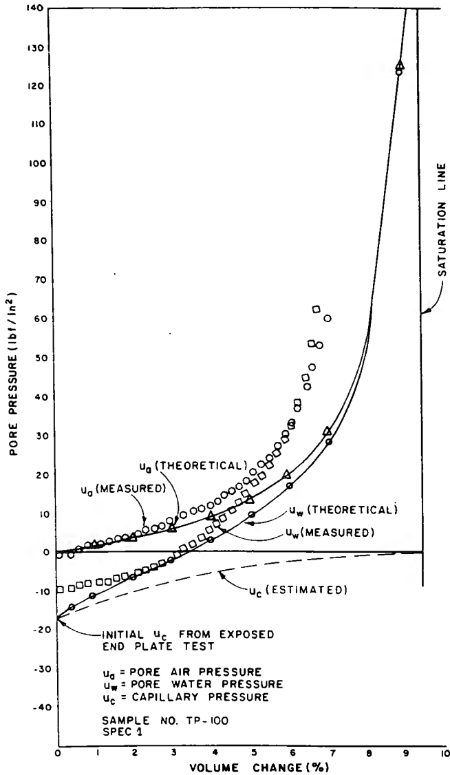
Figure X4.2. - Pore air and pore water pressures versus percent volume change—example.
