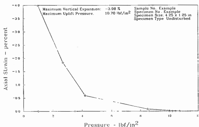
Figure 10. - Plot of test results — example.
