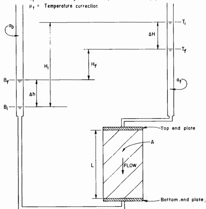
Figure X2.3.-Falling head permeameter with rising tailwater (flow from top end plate to bottom end plate).
