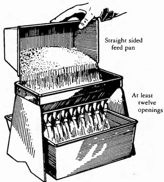
(b) Typical splitter for soils containing minus No. 4 sieve size particles.
