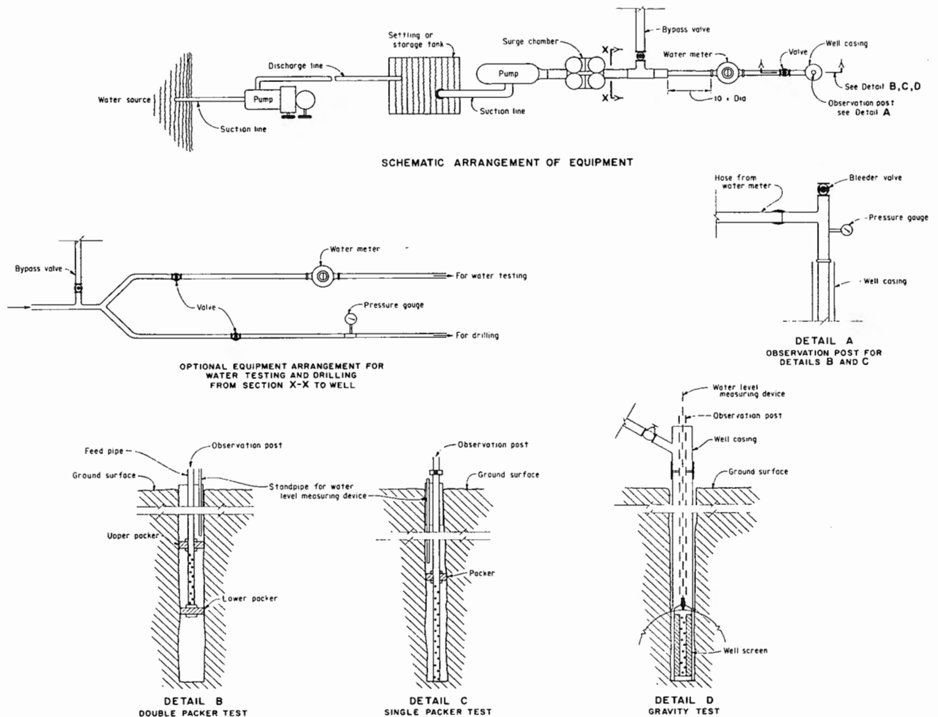
Figure 2. - Schematic arrangement of hydraulic conductivity equipment. 801-D-111
