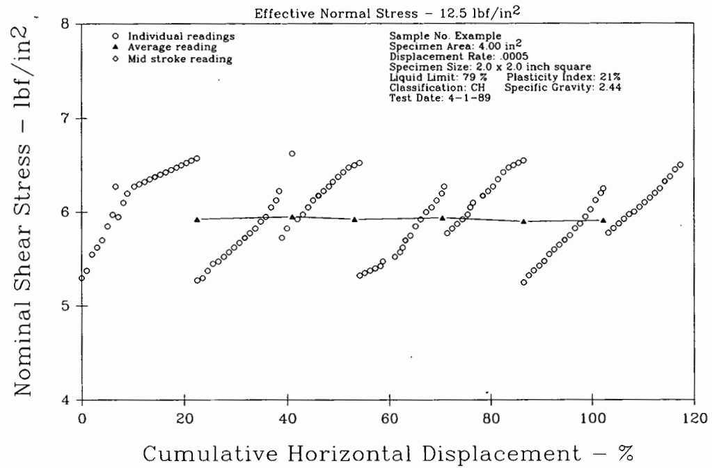
Figure 11. - Nominal shear stress versus cumulative horizontal displacement plot—example.
