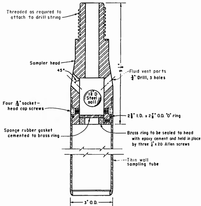
Figure 2. - Thin-wall push tube sampler.
