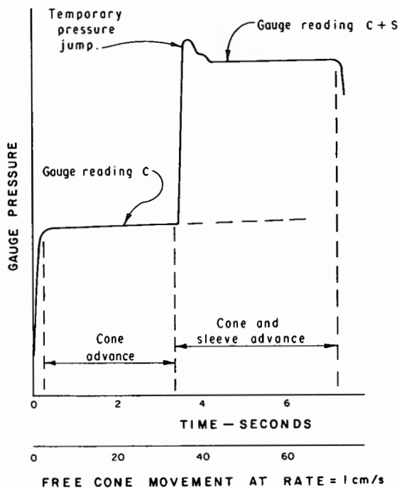
Figure 5. - Variation in gauge pressure during discontinuous mechanical friction — mantle cone penetration through a homogeneous deposit.
