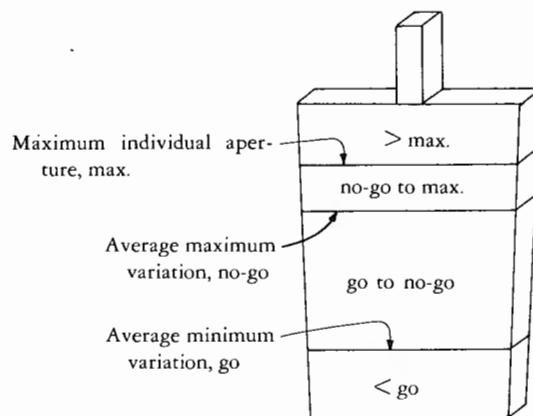
Figure 9. — Plug gauge schematic.
