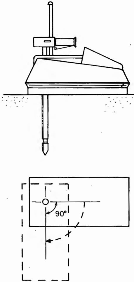
Figure 3. – Orientation of nuclear moisture-density gauge showing 90-degree rotation for second reading.
