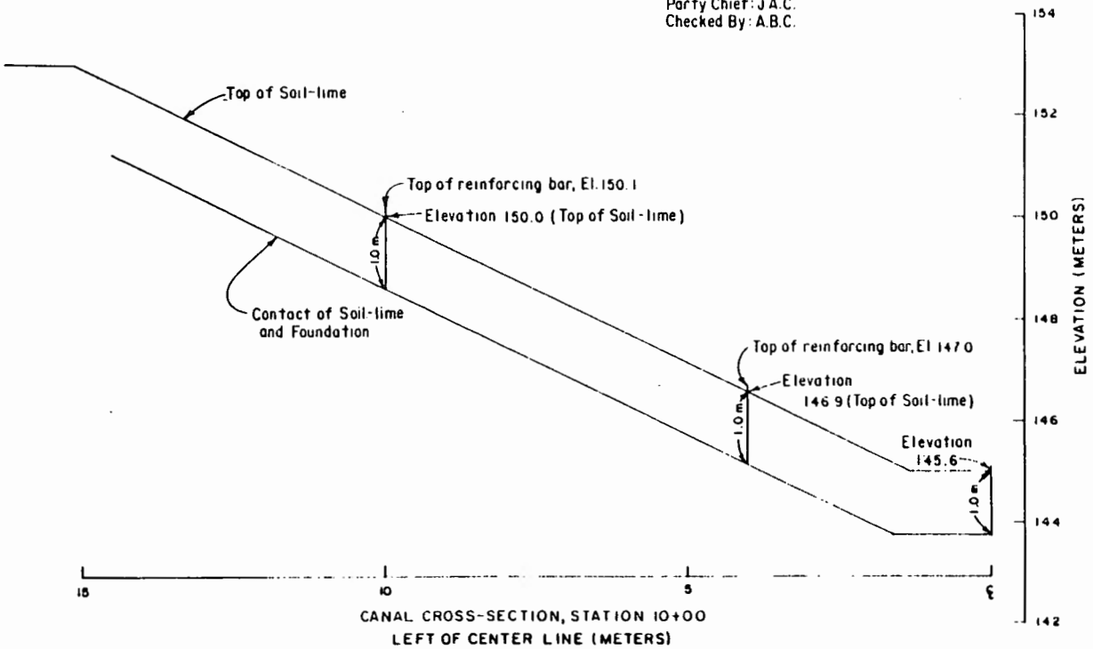
Figure 3B. - Typical soil-lime cross section (SI units).
