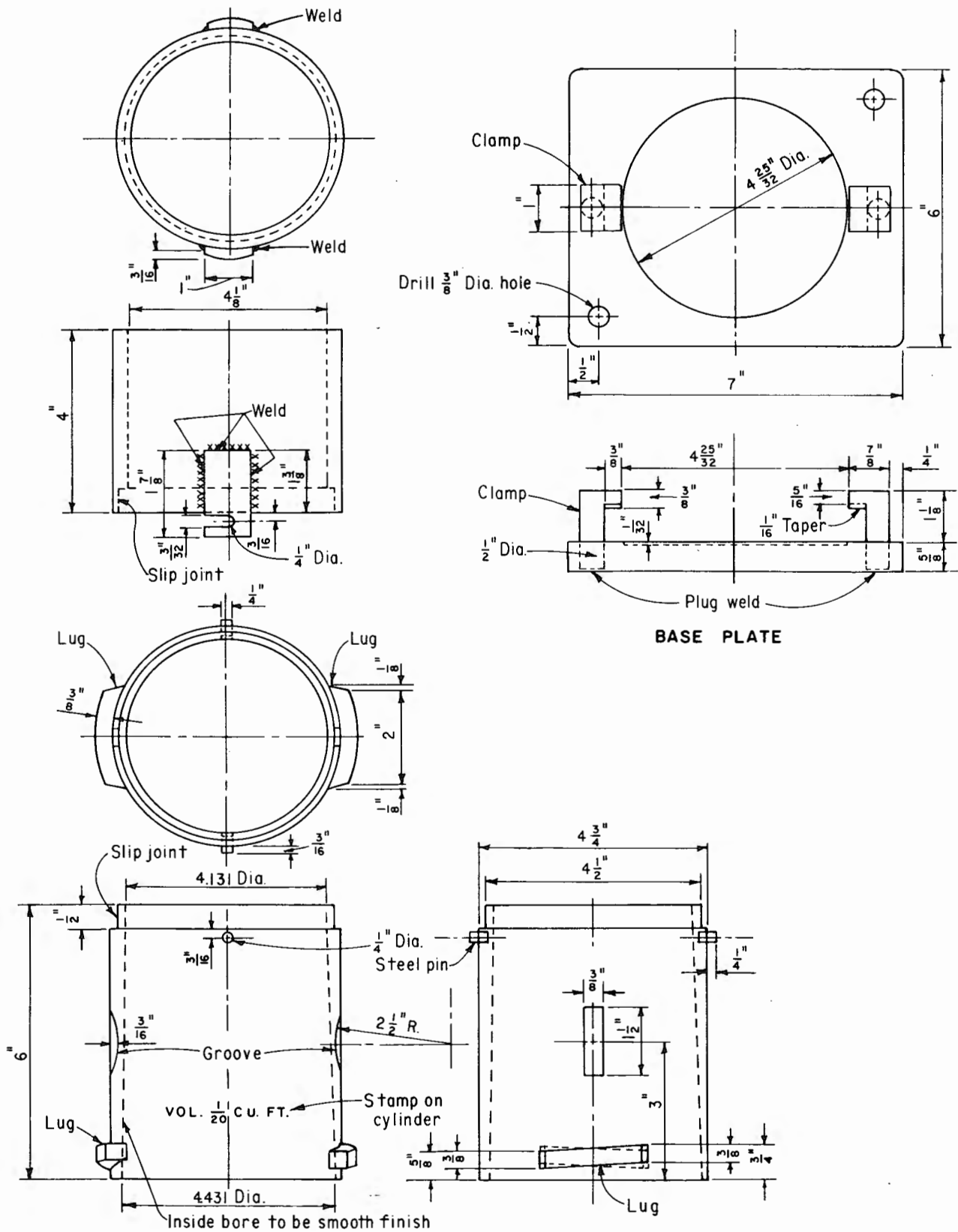
Figure 1. – Compaction mold.
