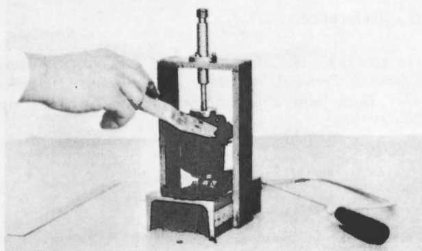
(b) Removing surplus soil by progressive vertical cuts.
