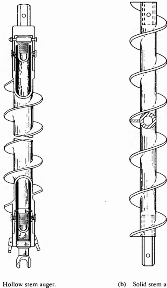
Figure 2. – Helical machine-operated augers.
