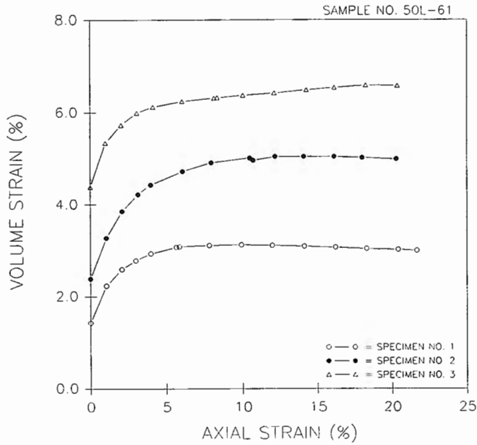
Figure 13. - Percent axial strain versus percent volume strain—example.
