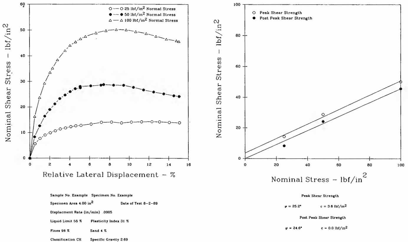
Figure 13. - Direct shear test plots — example.
