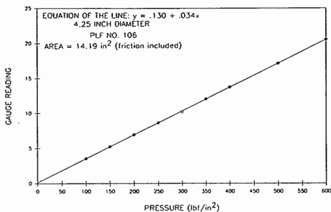
Figure X3.4.—Gauge reading versus applied pressure calibration (4.25-inch diameter specimen-high range) — example.
