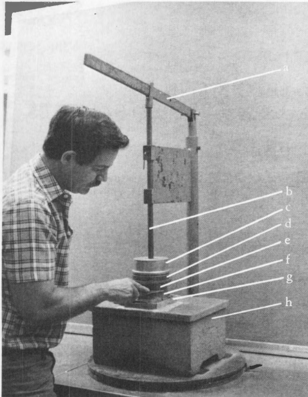
Figure 1. - Cutting an undisturbed soil specimen directly into testing chamber. (a) lever arm, (b) guide rod, (c) spacer chamber, (d) testing chamber, (e) cutting bit, (f) soil sample, (g) wax, and (h) cutting stand.
