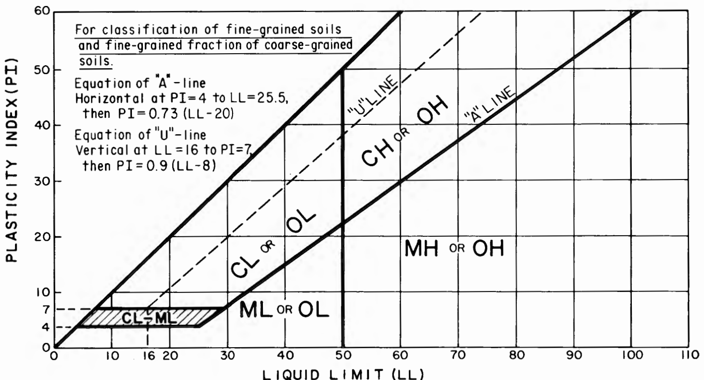
Fig. 3. — Plasticity chart.
