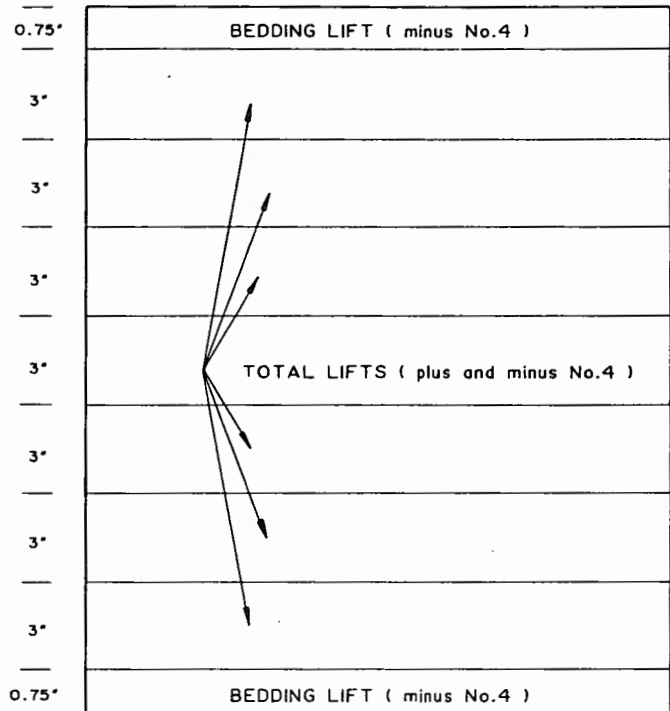
Figure 12.—Bedding lift placement information.
