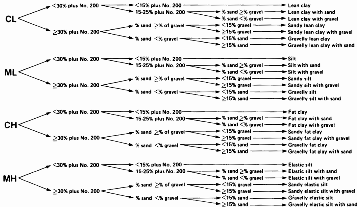
Figure 1a. – Flowchart for identifying inorganic fine-grained soil (50% or more fines) — visual-manual method.
