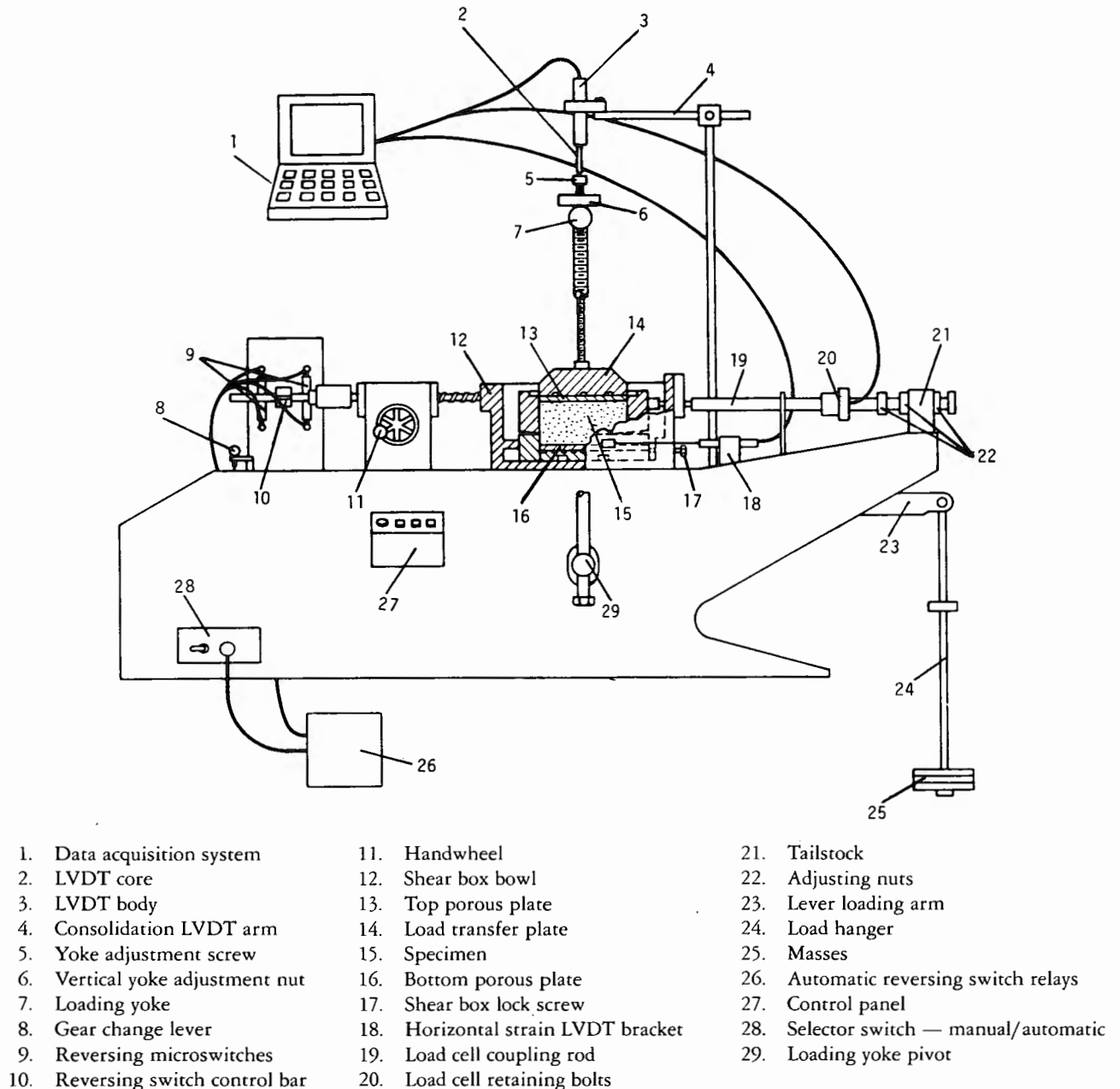
Figure 1. — Schematic of direct shear apparatus.
