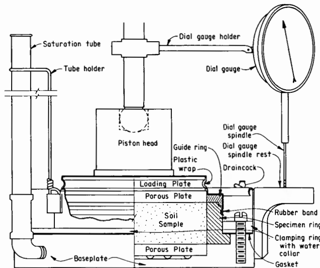
Figure 1. – Schematic of fixed-ring consolidometer.
