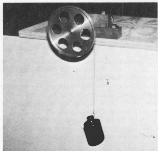
(b) Mass hung from Torvane calibration wheel.
