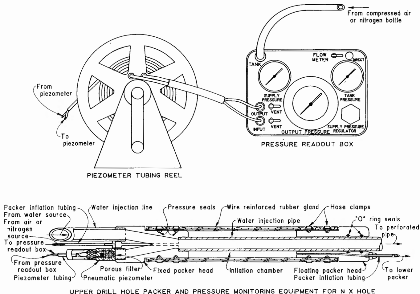
Figure X1.2. – Upper drill hole packer and pressure monitoring equipment for NX hole.
