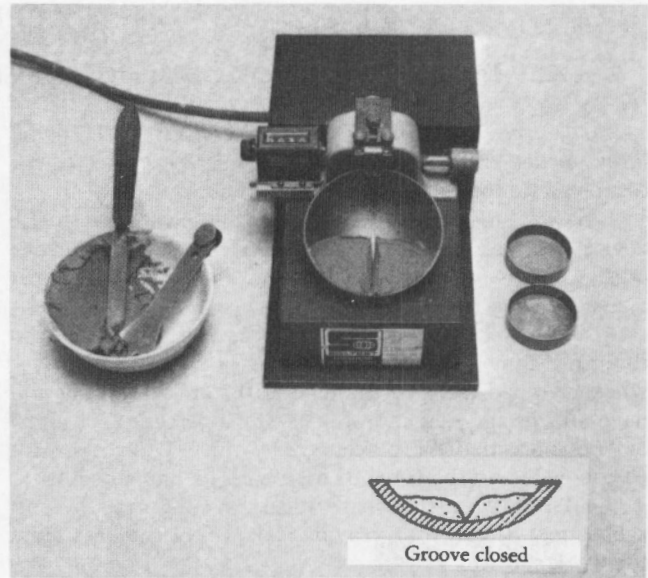
(b) Soil closed after test. Note groove closed in cup.
