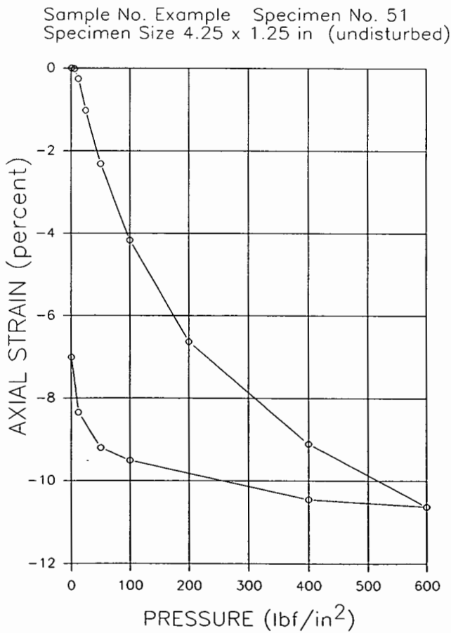
(a) Axial strain versus pressure.
