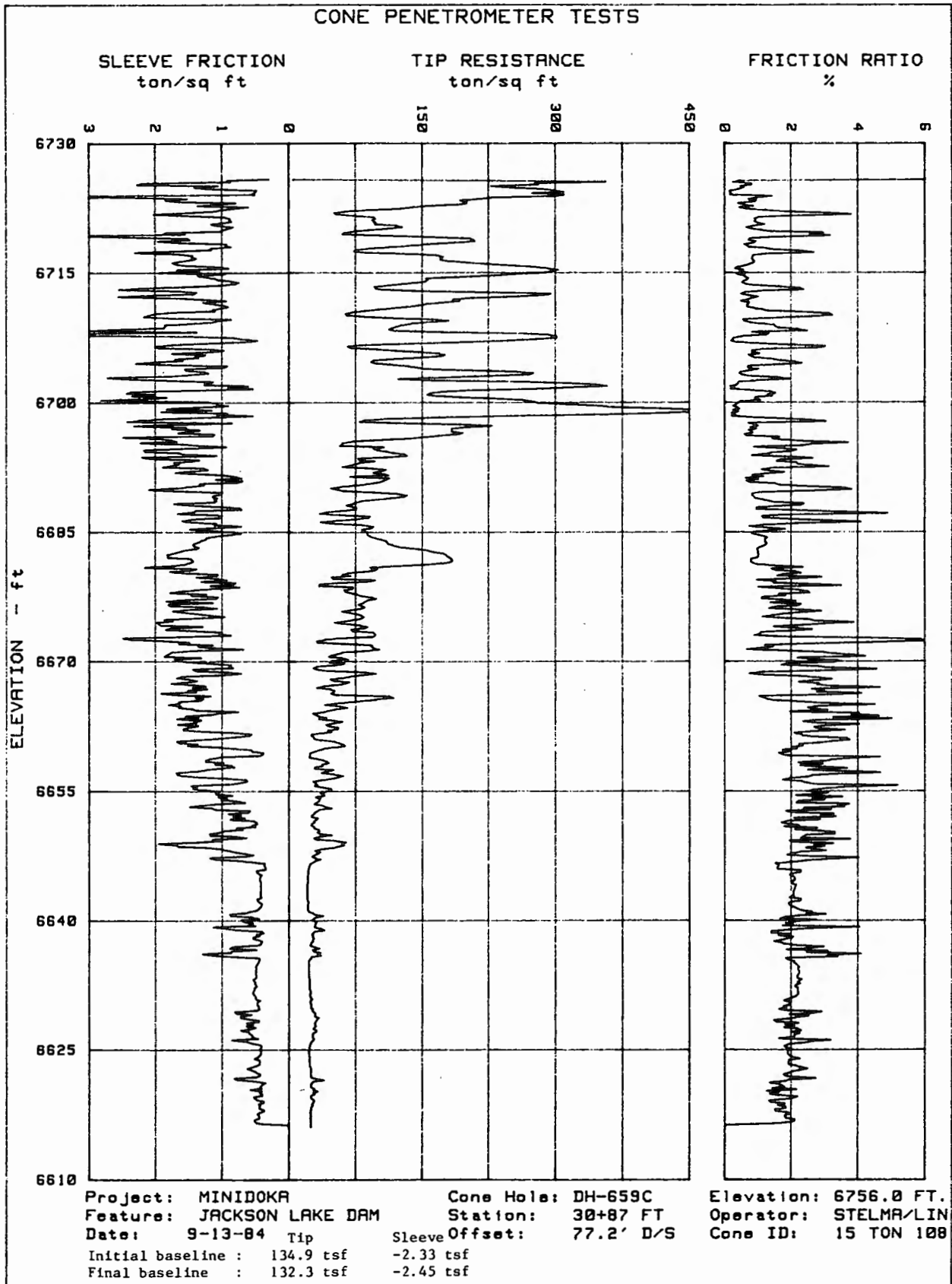
Figure 4. - Cone penetrometer tests — example.
