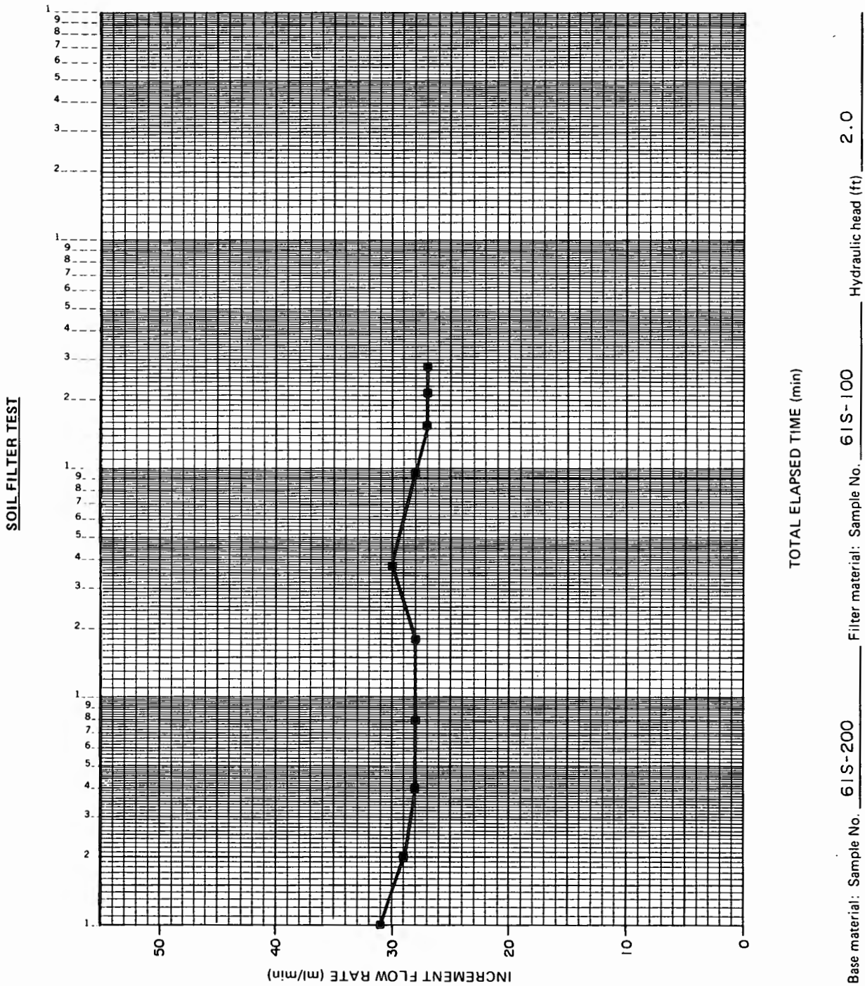
Figure 12. - Increment flow rate versus total elapsed time summary plot — 2.0 ft head example.
