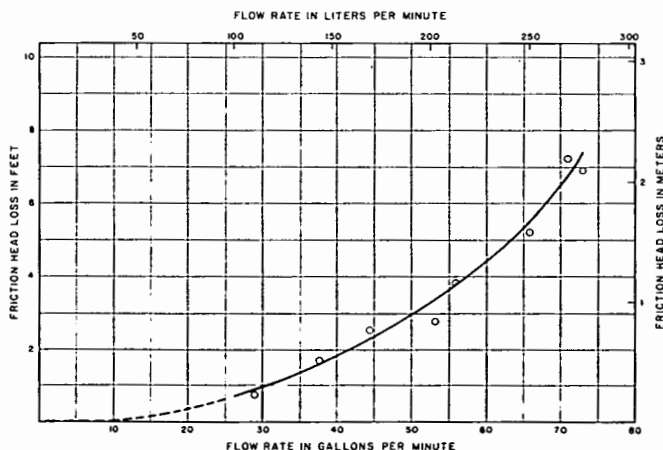
Figure 3. — Head loss due to friction at increasing flow rates for a 10-foot (3-m) 1-1/4-inch (32-mm) diameter iron pipe.
