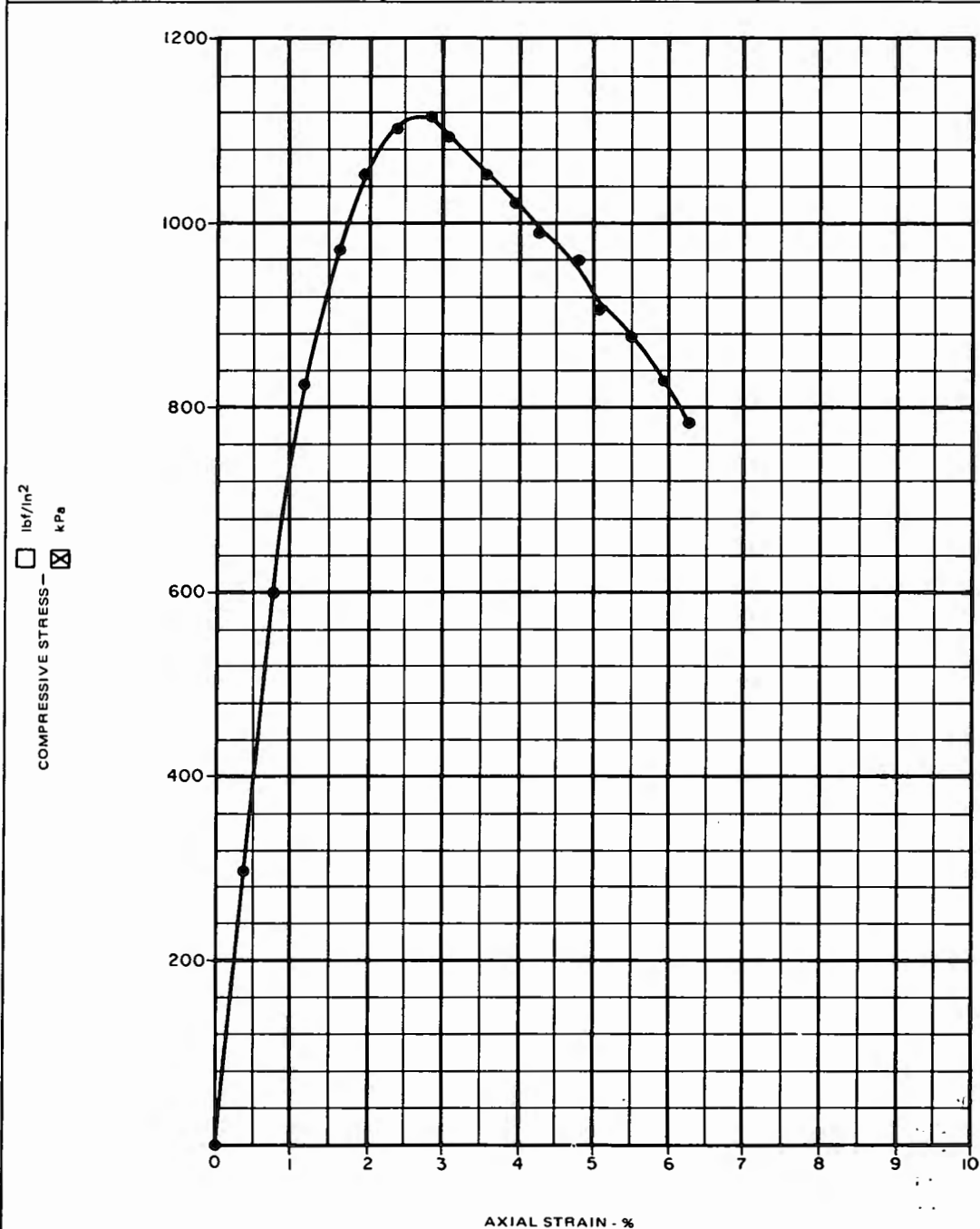
Figure 2B. - Soil-lime unconfined compressive strength test plot (SI example).
