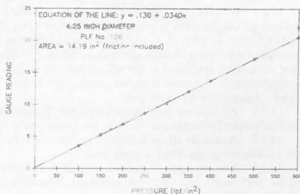
Figure 11. – Pneumatic load frame calibration (high range) — example.
