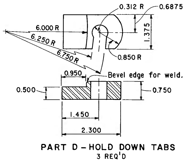
Figure X2.2. - Vibratory table calibration equipment — Continued. 101-D-647
