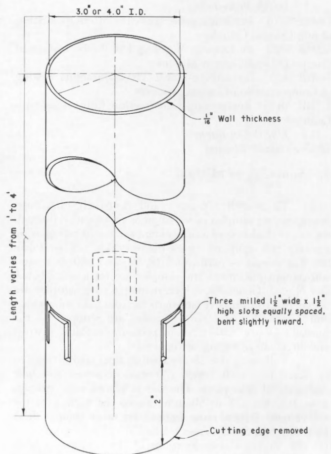
Figure 2. – Core retrieval barrels made from worn diamond studded core barrels.
