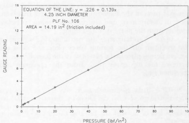
Figure 12. – Pneumatic load frame calibration (low range) — example.
