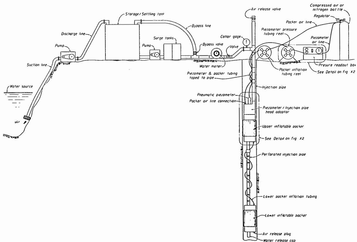
Figure X1.1. - Schematic arrangement of drill hole packer and pressure monitoring equipment. 801-D-180
