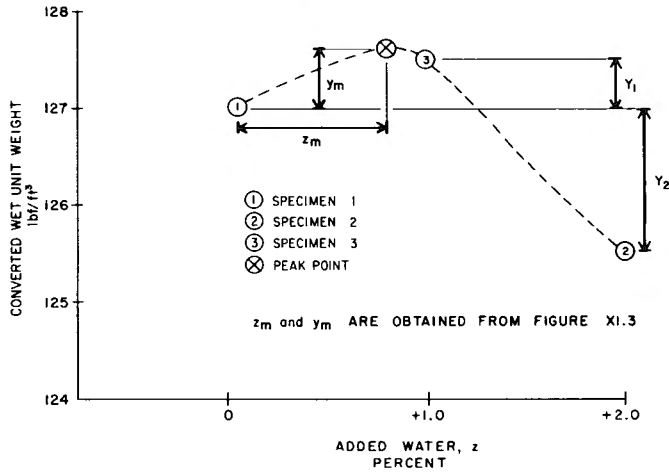
Figure X1.2. – Determining peak point of compaction curve, Y_1/Y_2 method.
