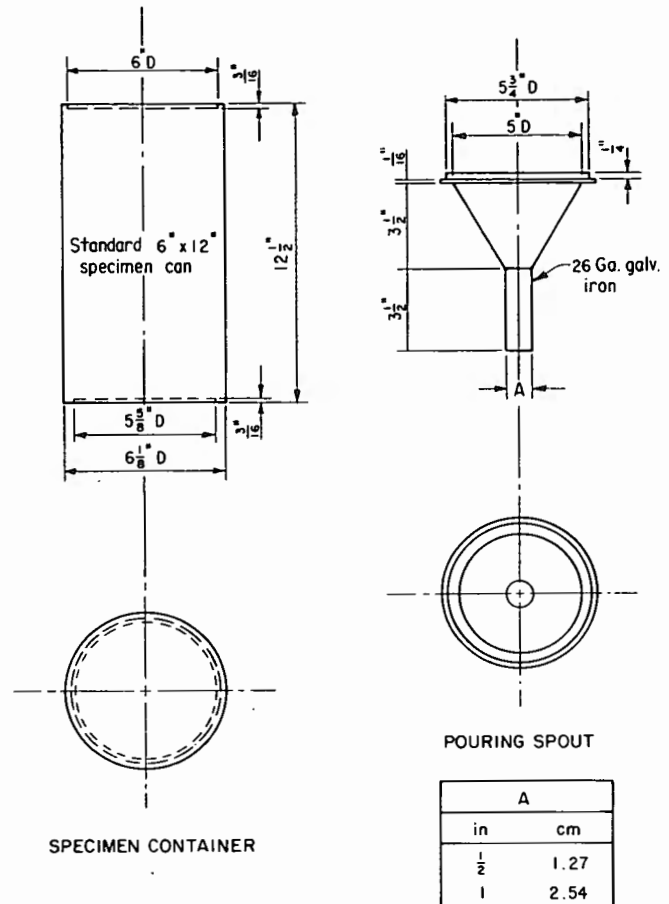
Figure 3. – Minimum index unit weight pouring device.
