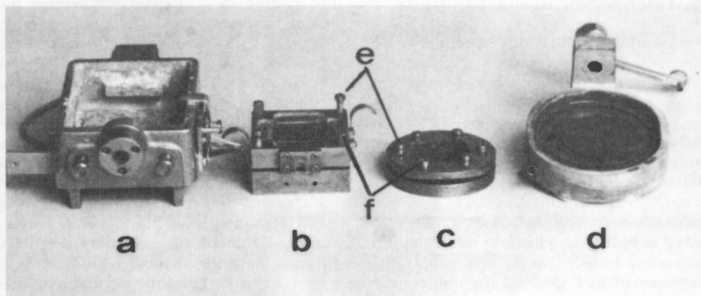
Figure 2.—Shear box bowls with associated shear boxes with gap and alignment screws installed. (a) shear box bowl, (b) shear box with removable bottom porous plate, (c) shear box, (d) shear box with bottom porous plate attached, (e) gap screws, and (f) alignment screws.
