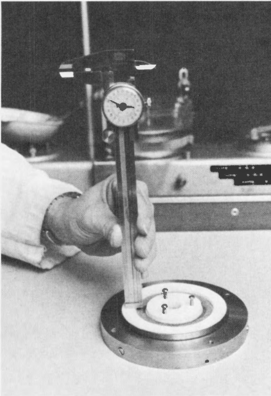
Figure 8. - Height of the inner confining disk is controlled by turning the three screws in it.
