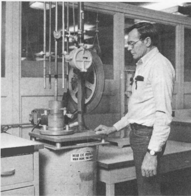
(a) Rainhart compactor
