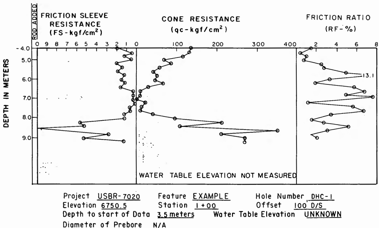
Figure 6. — Mechanical cone penetration test — example.
