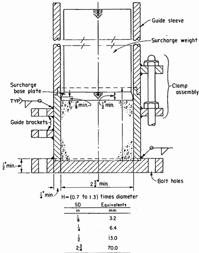
Figure 2. – Special unit weight measures [ASTM D 4254].
