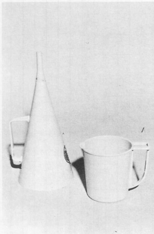
Figure 1. — Marsh funnel and graduated cup.
