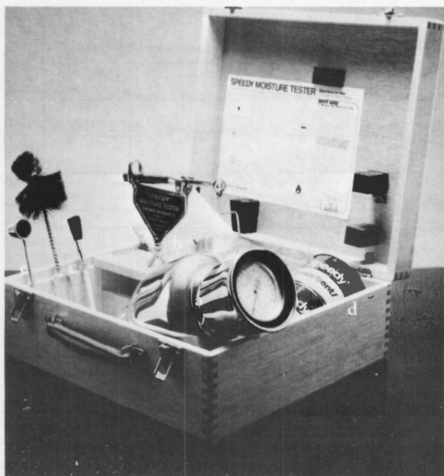
Figure 1. – Calcium carbide reaction device and accessory equipment, (a) CCRD, (b) brass beam balance, (c) cleaning brushes, (d) calcium carbide reagent, and (e) standard measuring scoop.
