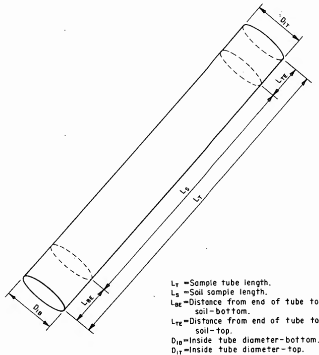
Figure 5. – Uncut sample tube showing trimmed soil sample within sample tube.
