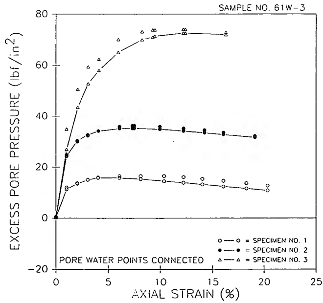
Figure 12. - Percent axial strain versus excess pore pressure—example.
