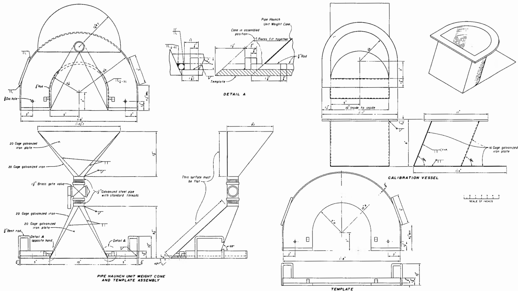
Figure 3. - Pipe haunch calibration vessel. (801-D-223)
