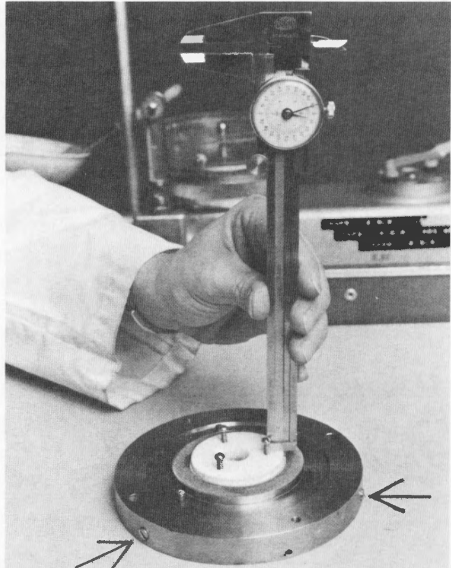
Figure 9. - The height of the outer confining ring is controlled by three screws in the lower platen. The heads of two (arrows) are visible in this view.
