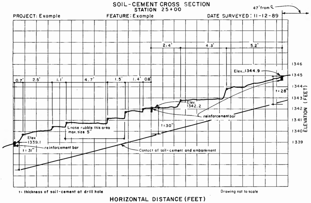
Figure 5. - Soil-cement cross-section detail — example.
