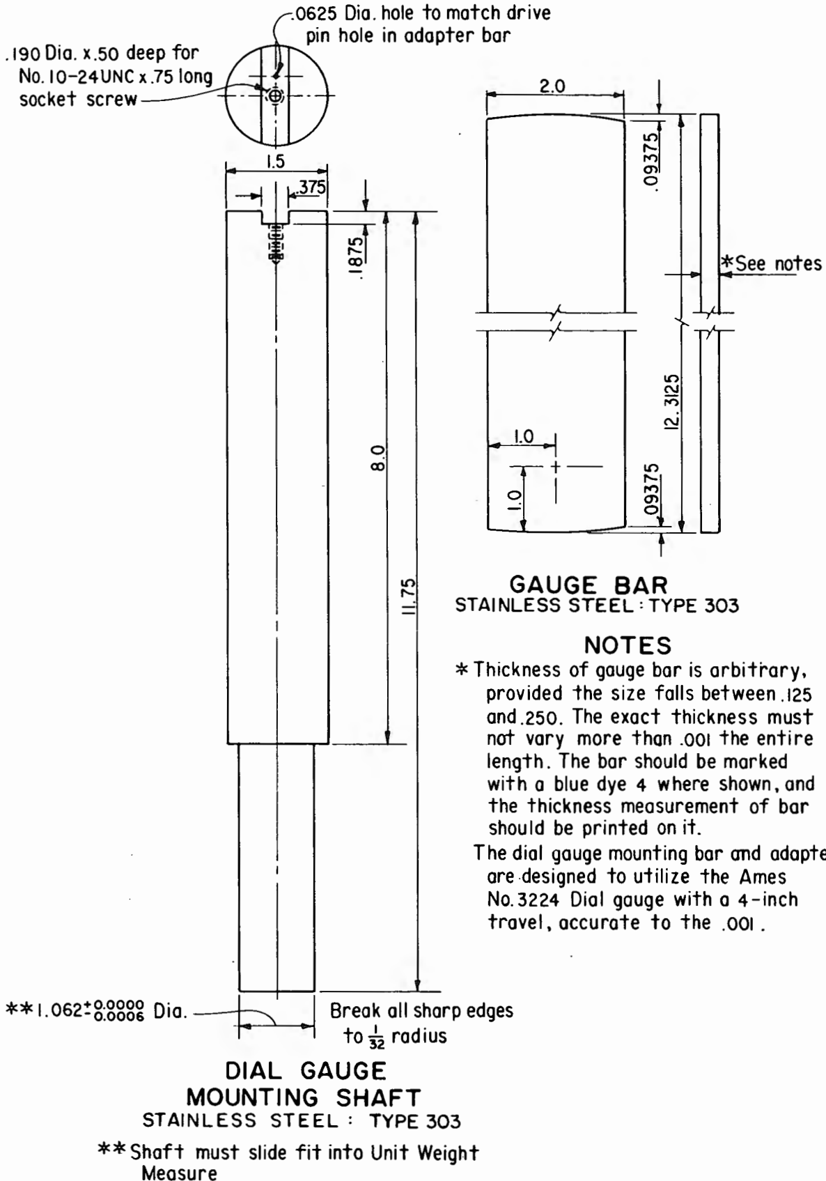
Figure 6. - Maximum index unit weight test equipment (sheet 4 of 4).
