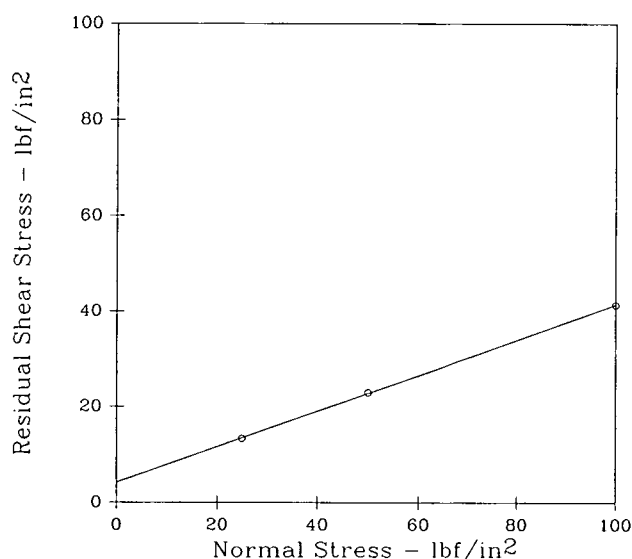
Figure 22. - Residual shear stress (average) versus normal stress plot (Feature: torsional shear) — example
