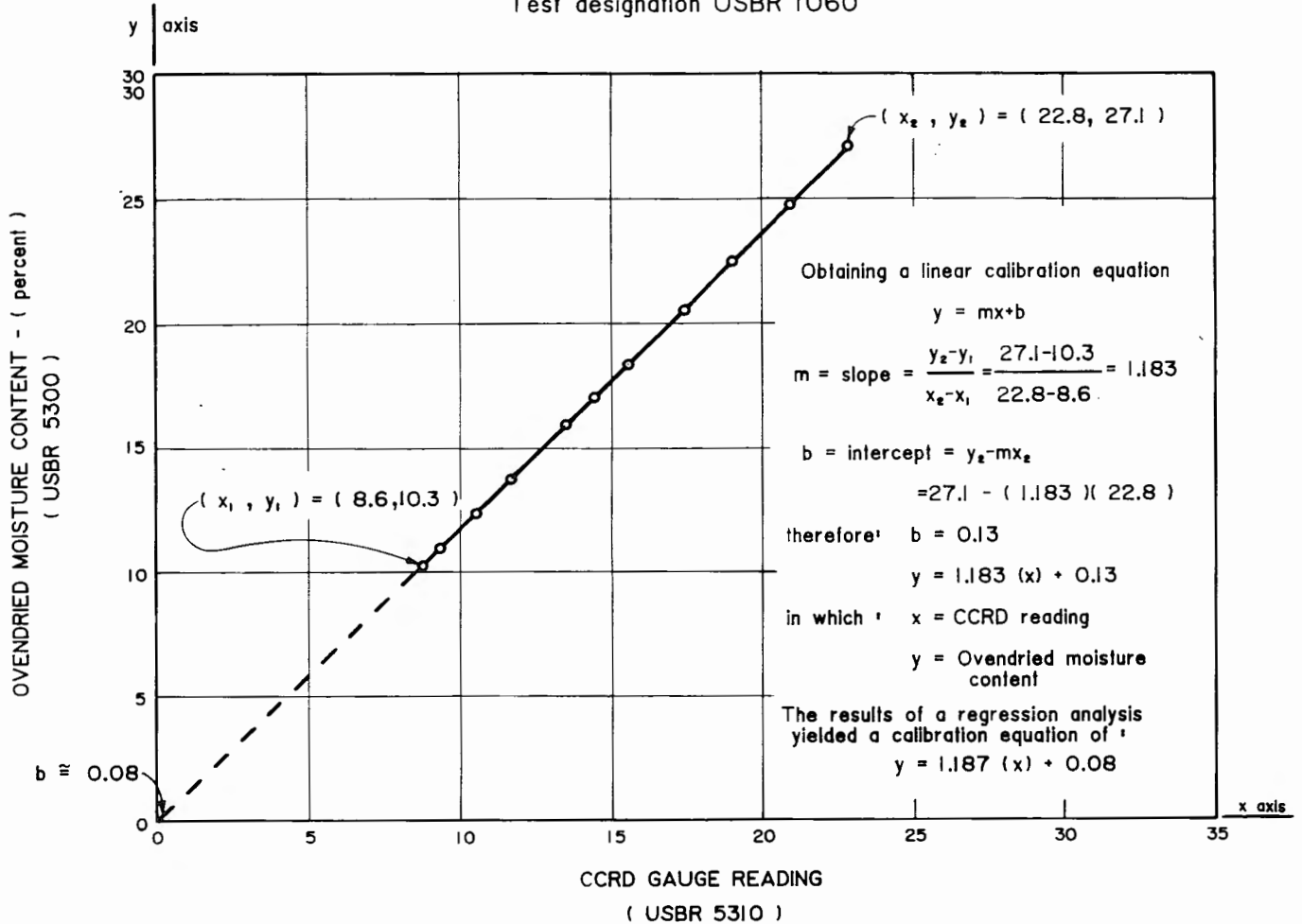
Figure 2. - Ovendried moisture content versus CCRD gauge reading — example.
