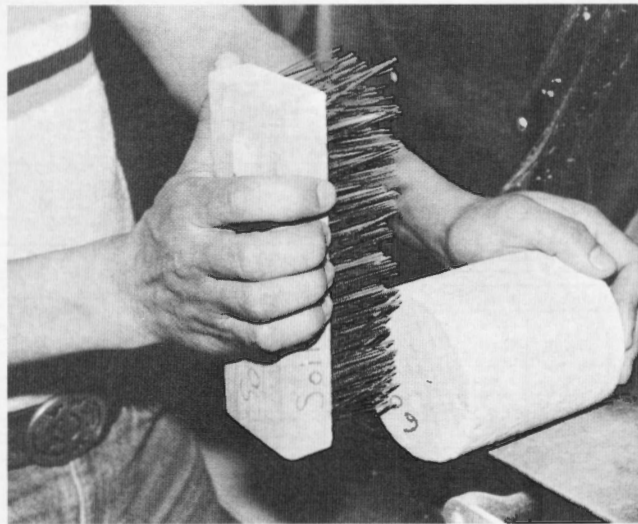
(c) Closeup view of brush strokes applied to the end of a soil-cement durability test specimen.
