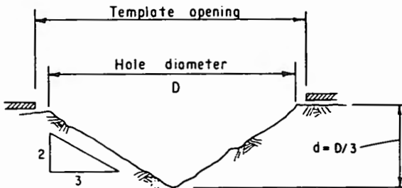
Figure X1.1. – Test pit configurations.
