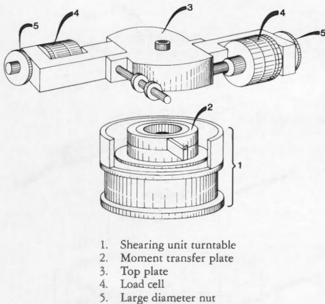
Figure 4. - Top plate placement onto the shearing unit turntable.
