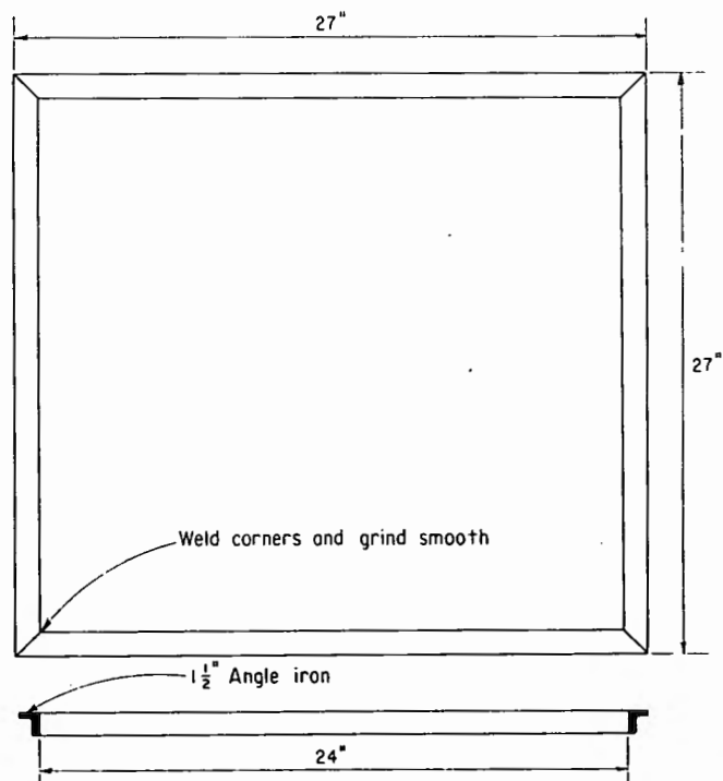
Figure 1. — Square template.—The template represents a design that has proved satisfactory. Template dimensions will vary according to the size of the test pit to be excavated. Other sizes may be used as long as the template is rigid enough to serve as a pattern for the excavation.
