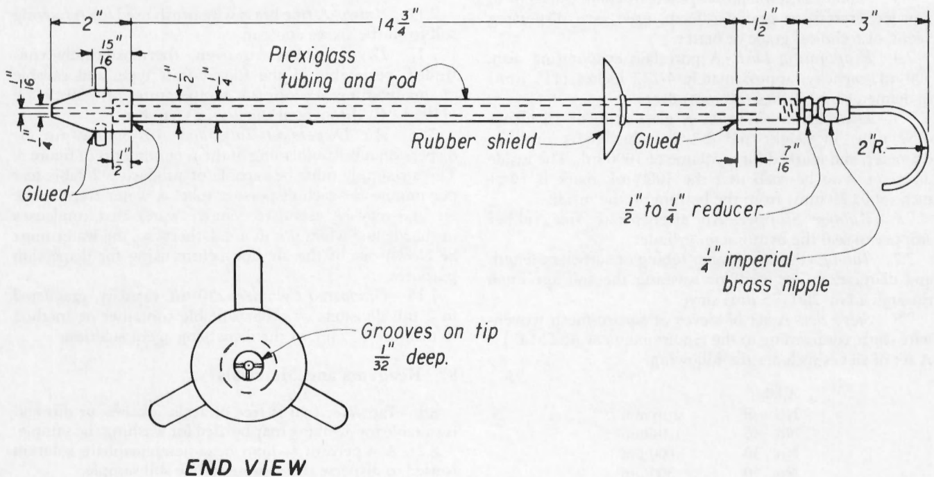
Figure 3. - Air dispersion tube. 101-D-523
