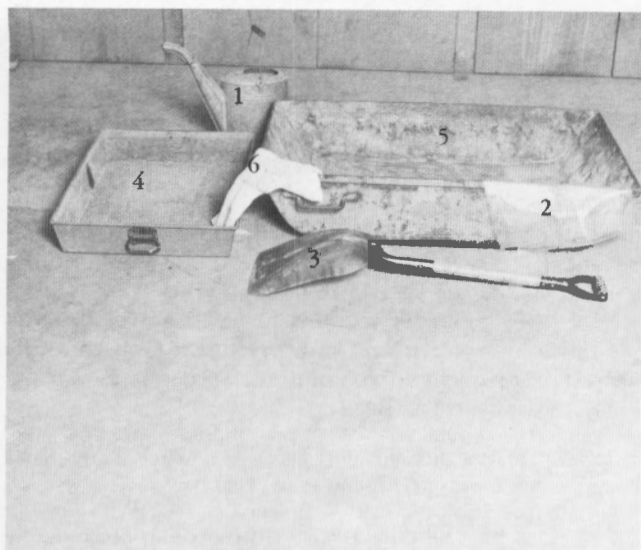
Figure 1. - Mixing equipment: 1) sprinkler can, 2) moisture bag, 3) shovel, 4) large moisture pan, 5) mixing pan, and 6) towel.
