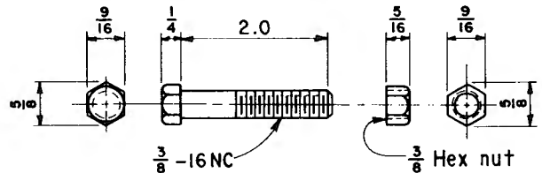
STANDARD \frac{3}{8} NC BOLT AND NUT PART G TWO REQUIRED
