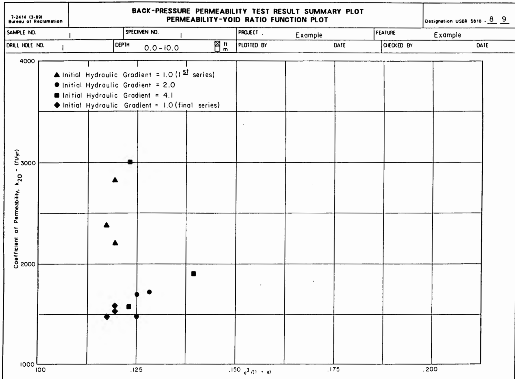
Figure 9. - Back-pressure permeability test result summary plot (permeability-void ratio function plot) — example.
