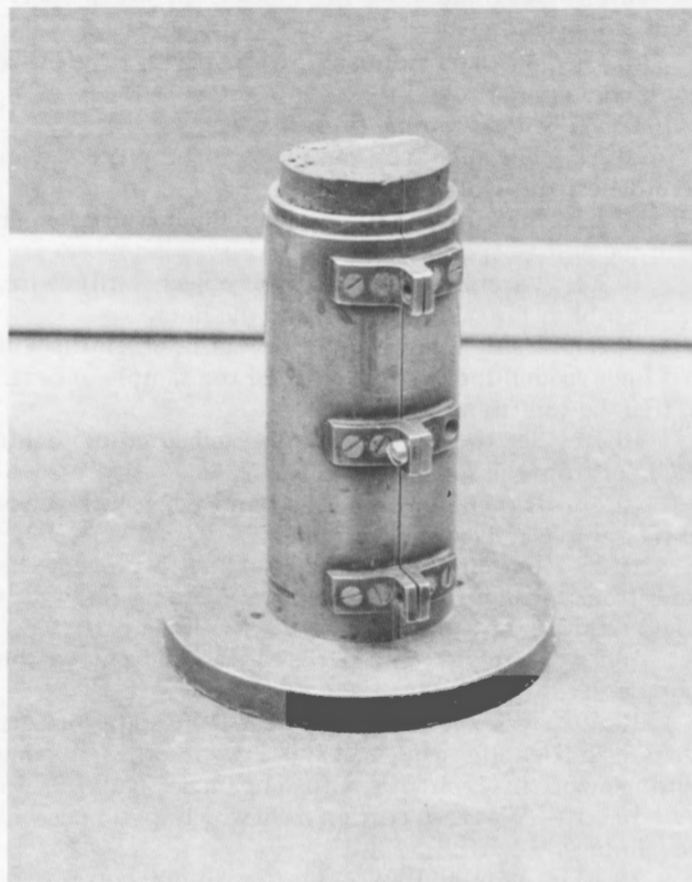
Figure 3. — Soil specimen in trimming mold.
