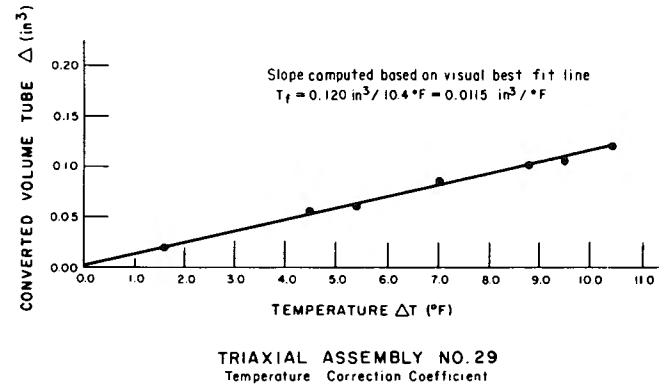
Figure X1.2. – Temperature correction coefficient plot—example.
