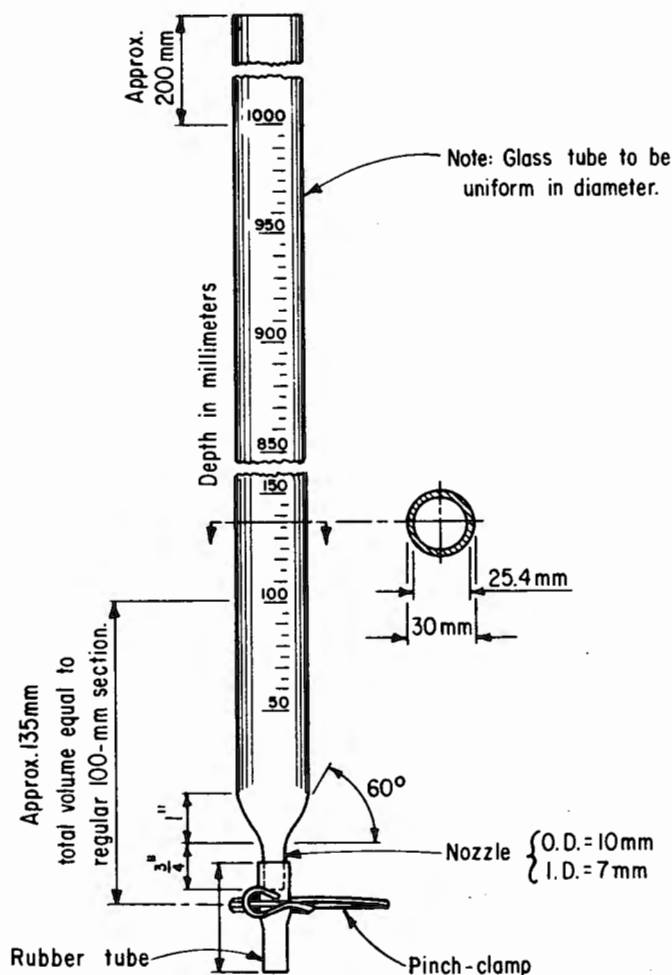
Figure 1. — Bottom withdrawal tube with quick acting outlet.
