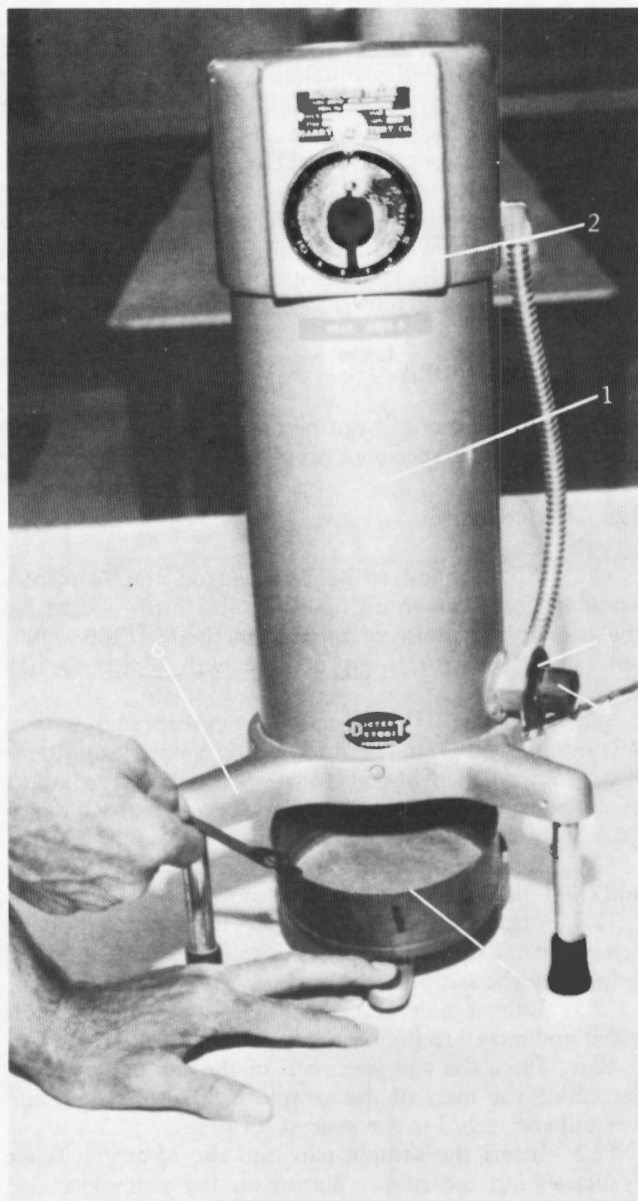
Figure 1. — Moisture Teller with accessory equipment. 1) Moisture Teller device, 2) timer, 3) adjustable thermostat, 4) thermometer, 5) pan holder, and 6) pan lifter.
