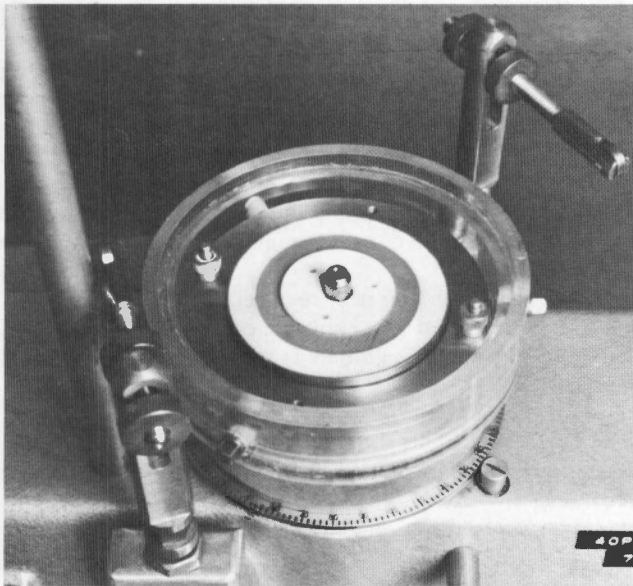
Figure 14. - Lower platen secured by clamp nuts (nuts to the left and right of the outer confining ring).
