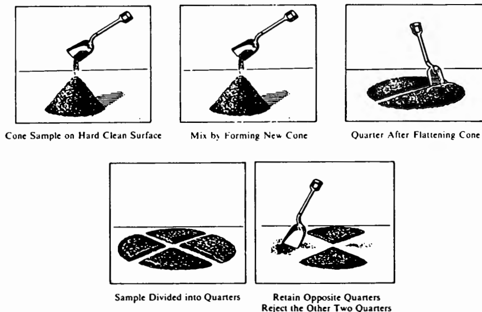
Figure 2. – Quartering done on a hard, clean, level surface [ASTM C 702].
