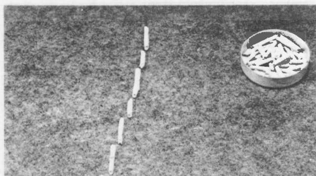
Figure 3. - Test for plastic limit.
