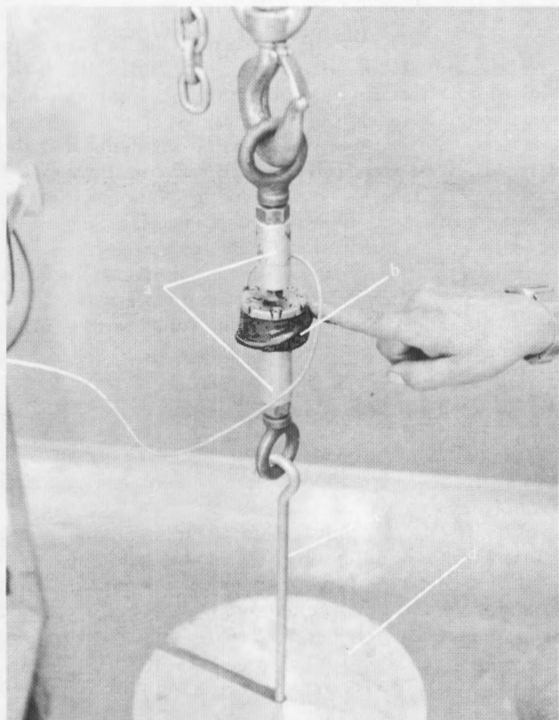
Figure 1. – Force transducer (load cell) and hanger. a) load cell couplers, b) load cell, c) hook, and d) hanger assembly with mass.
