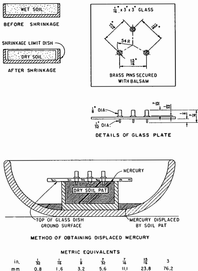
Figure 1. — Apparatus for determining the volumetric change [ASTM D 427, vol. 04.08].
