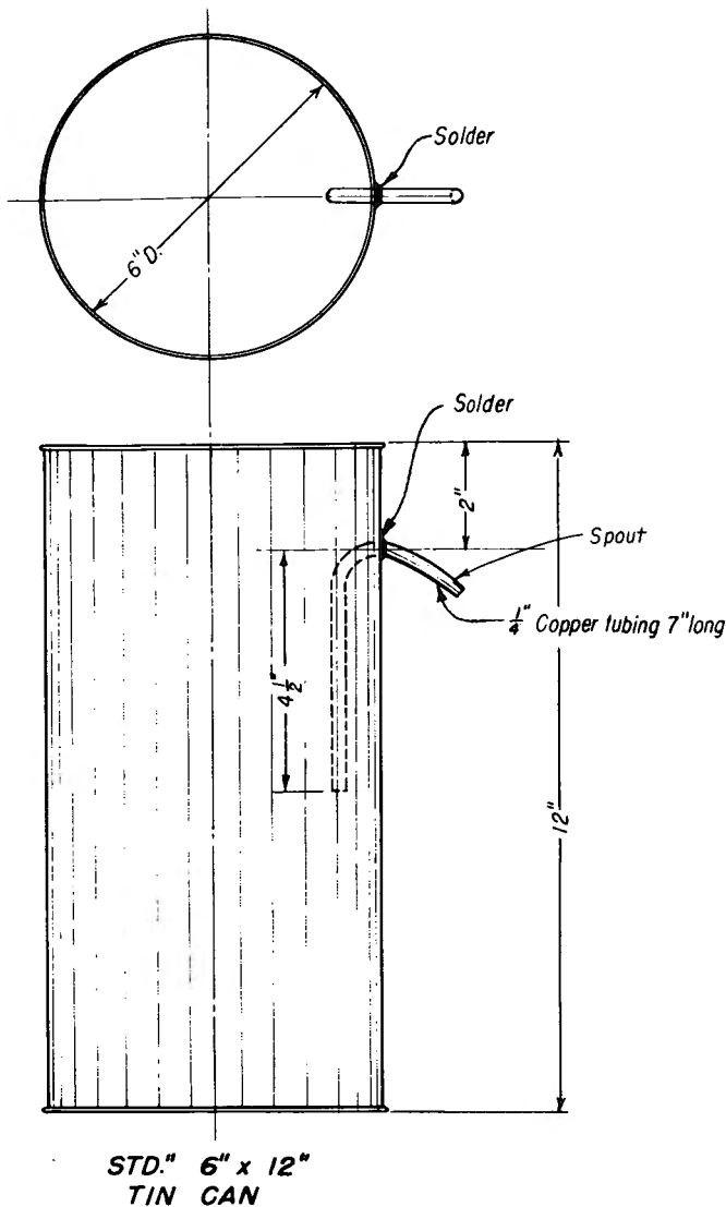
Figure 5. – Specific gravity siphon can.
