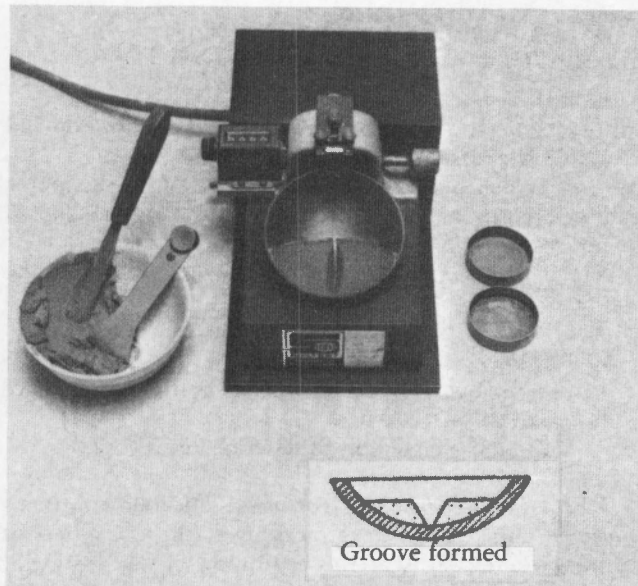
(a) Soil divided before test. Note groove formed in cup.
