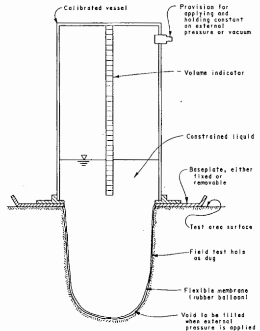
Figure 1. — Rubber balloon apparatus (drawing not to scale).
