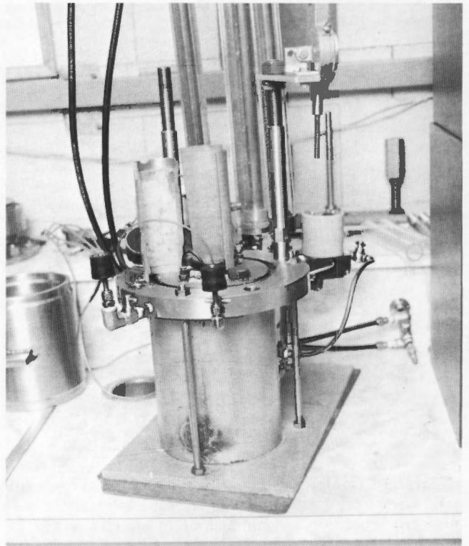
Figure 7.—Stand-up vacuum mold with membrane under vacuum (2.0-dia. by 5.0-in high).
