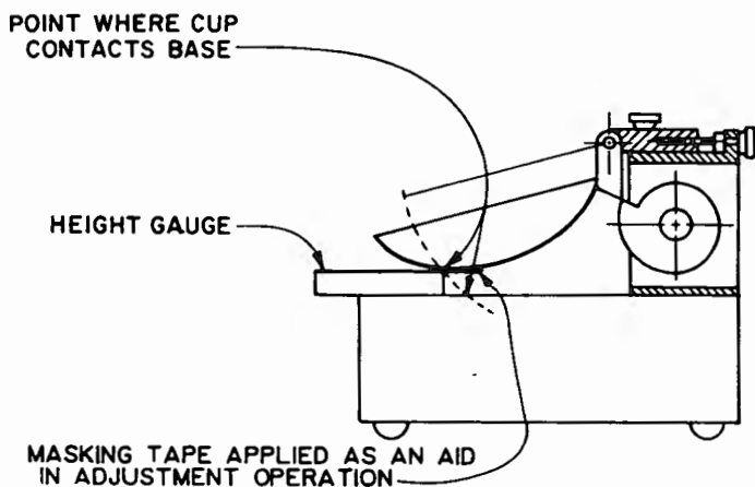
Figure 5. - Calibration for height of drop [ASTM D 4318].
