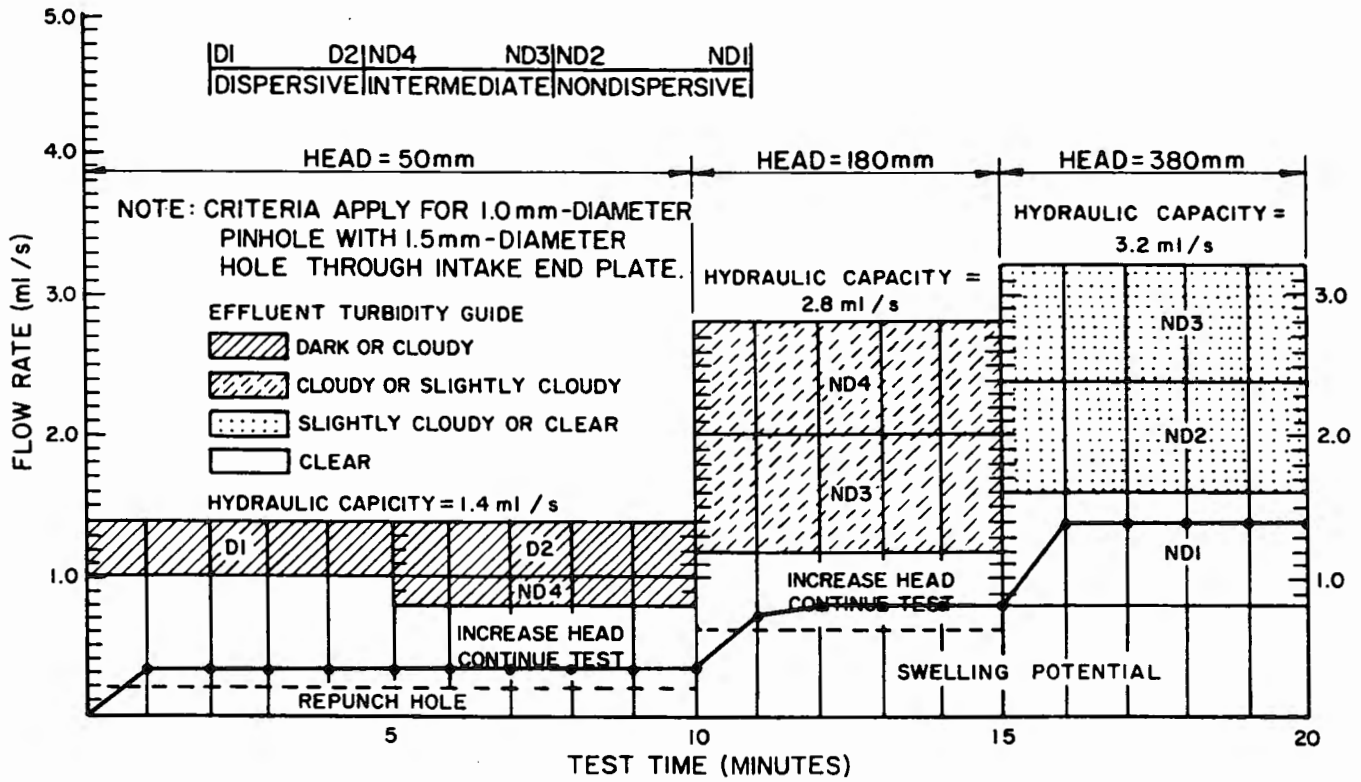
DISPERSIVE GRADE VS FLOW RATE
