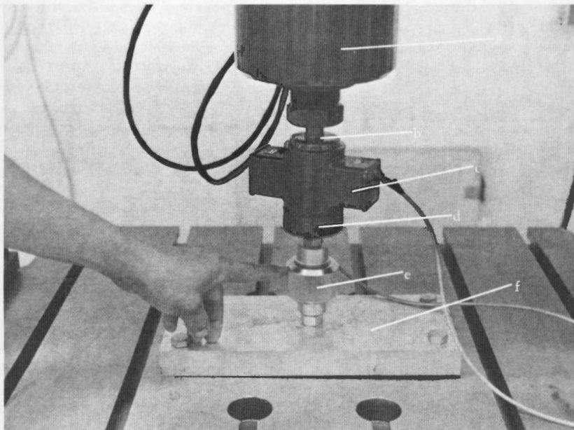
(b) Force transducer calibration using universal testing machine (tension). a) universal testing machine force transducer, b) coupler, c) force transducer being calibrated, d) coupler, e) swivel coupler, and f) platform adaptor.
