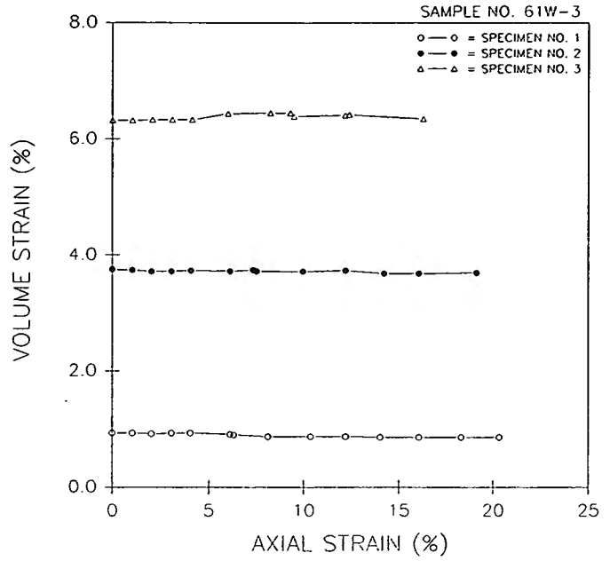
Figure 13. - Percent axial strain versus volume strain—example.
