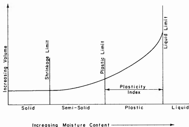
Figure 1. - Atterberg limits.
