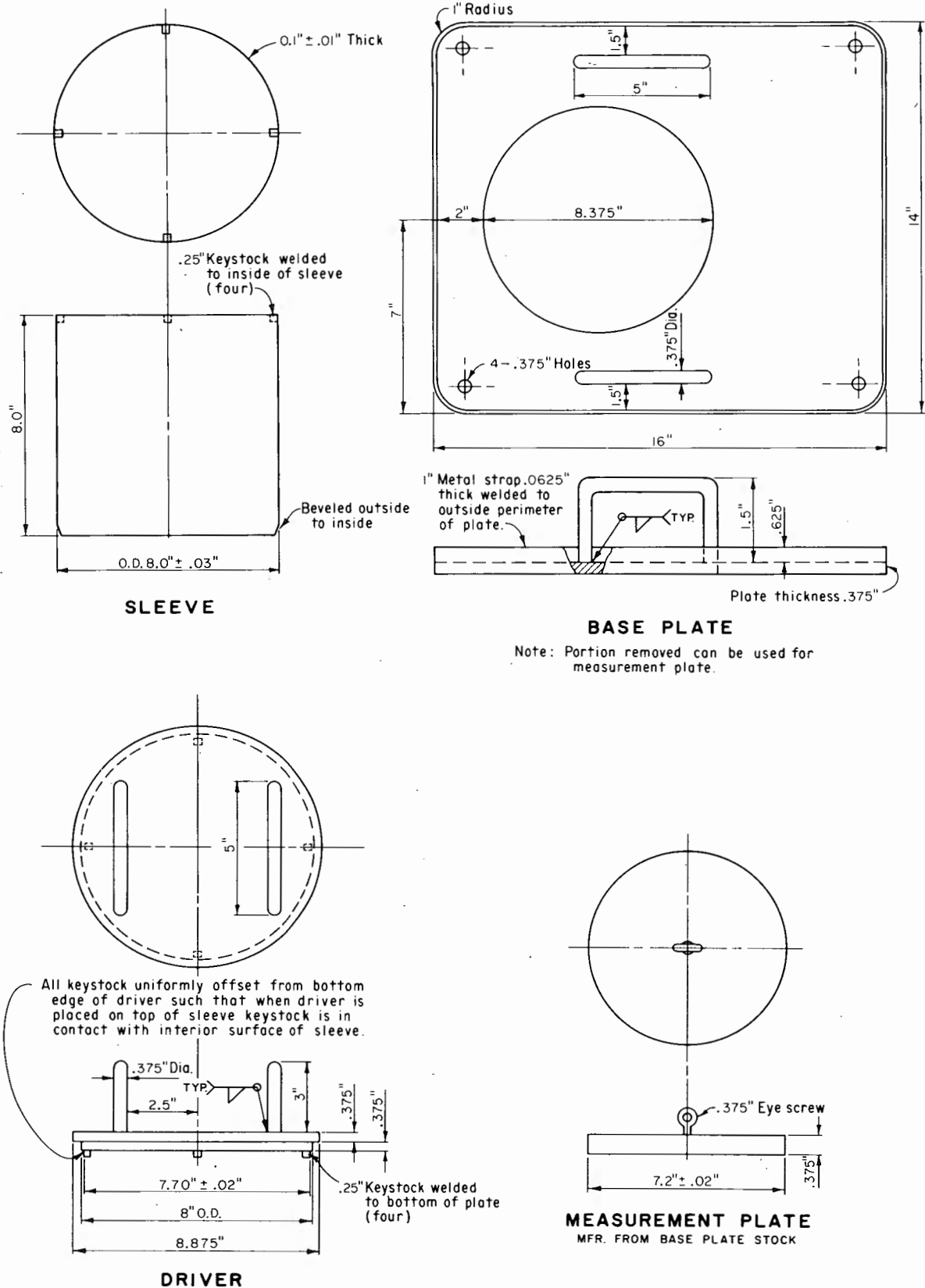
Figure 1. - In-place soil density equipment —sleeve apparatus.
