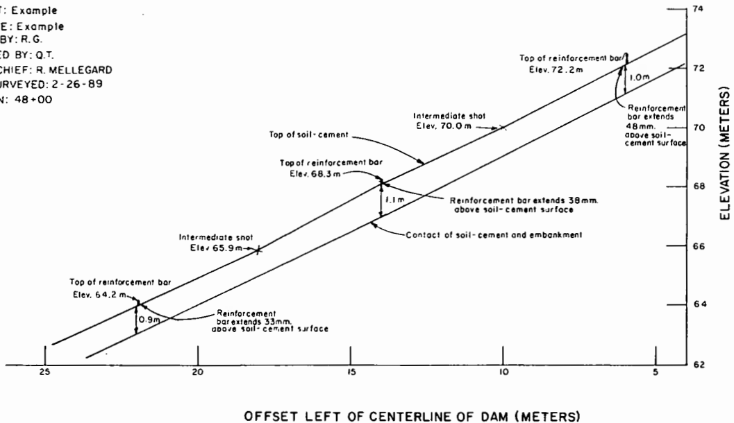
Figure 4B. - Soil-cement cross section (SI example).
