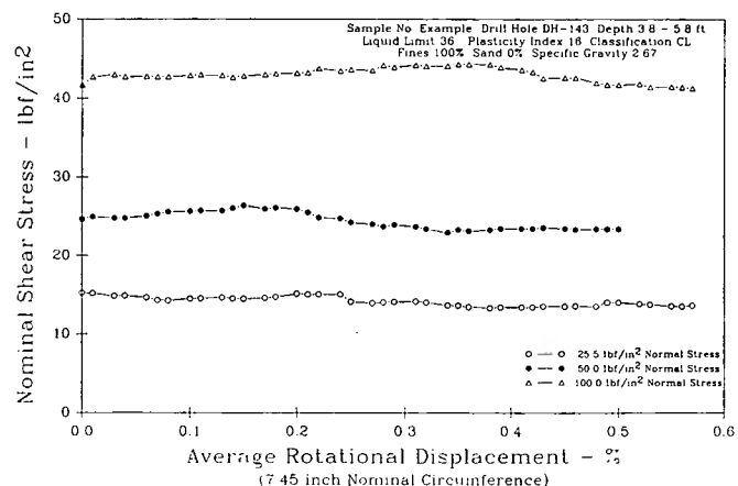
Figure 21. - Nominal shear stress versus average rotational displacement (%) plot — example.
