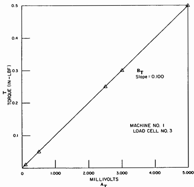
Figure 5. — Torque transducer calibration plot — example.
