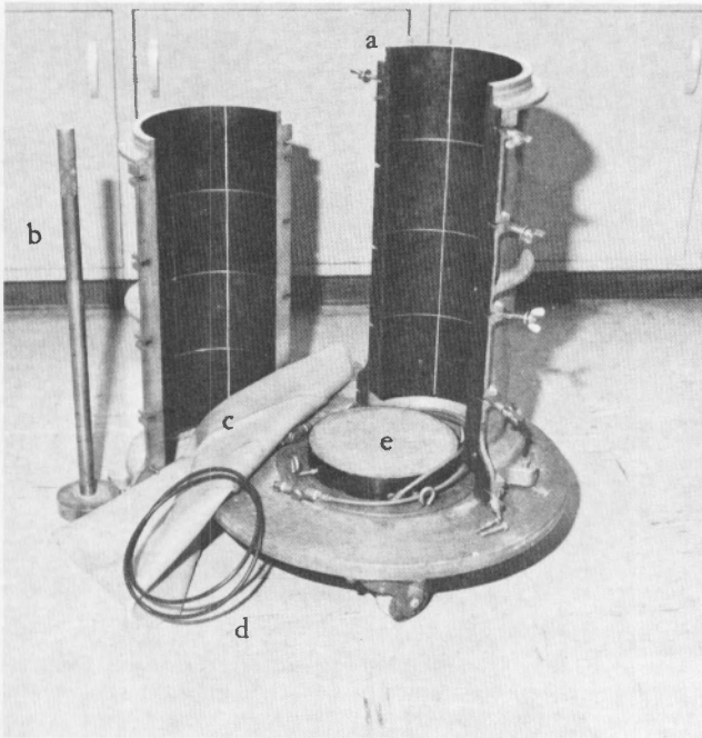
Figure 8.—Stand-up vacuum mold equipment (9.0-dia. by 22.5-in high). a) split compaction mold, b) tamper, c) specimen membrane, d) O-rings, and e) bottom end plate (triaxial).
