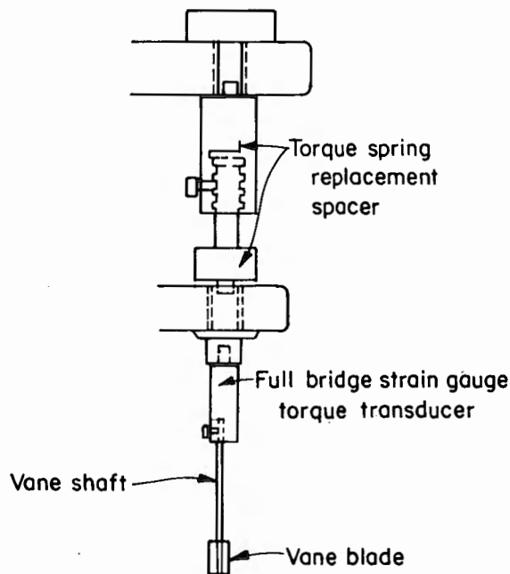
(a) Electrical torque transducer.
