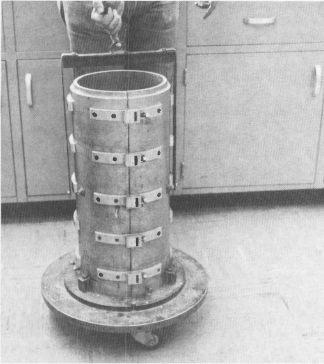
Figure 4.—Assembled split mold with lifting cradle.
