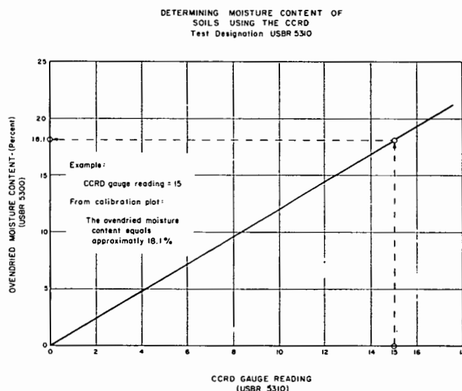
Figure 3. - CCRD calibration plot — example.
