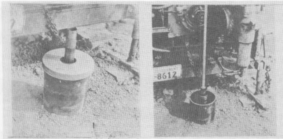
(a) Install 8-inch anchor casing and press vane stem to position.
