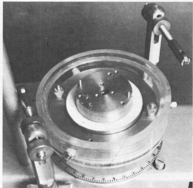
Figure 15. - Upper platen in place over the soil specimen.
