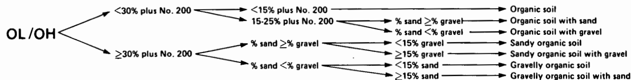
Figure 1b. – Flowchart for identifying organic fine-grained soil (50% or more fines) — visual-manual method.
