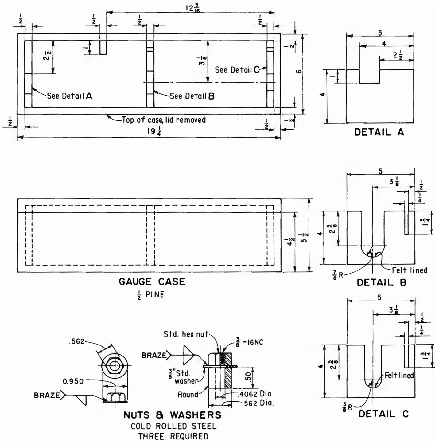
Figure 6. - Maximum index unit weight test equipment (sheet 3 of 4).
