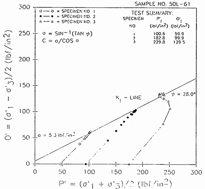
Figure 9. - p' - q' diagram—example.
