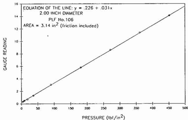
Figure X3.3.—Gauge reading versus applied pressure calibration (2.00-inch diameter specimen-low range) — example.
