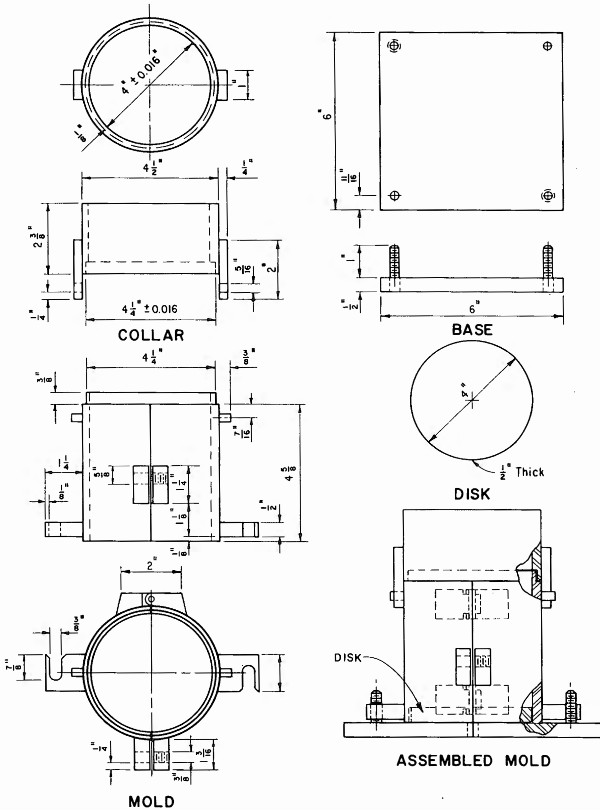
Figure 1. - Soil-cement durability mold.
