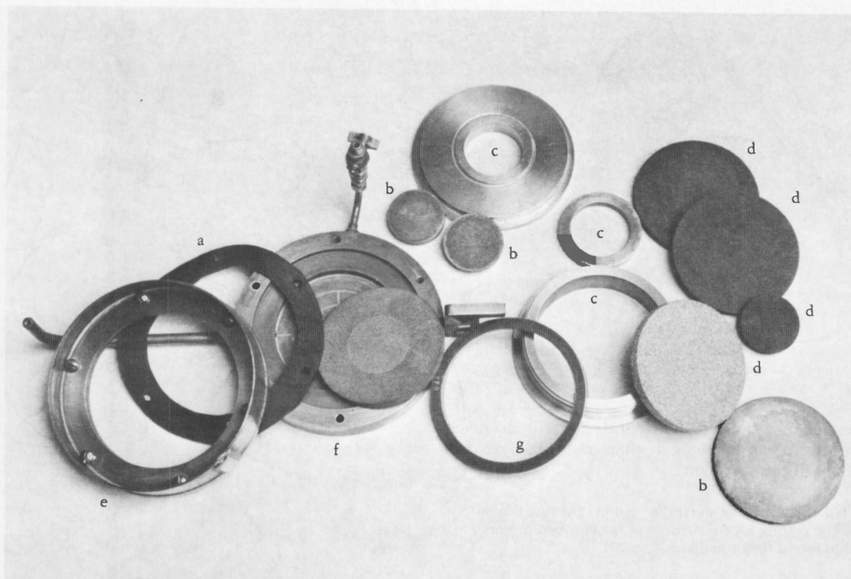
Figure 4. – Unassembled fixed-ring consolidometer. (a) gasket (rubber), (b) loading plates, (c) specimen ring, (d) porous plates, (e) water collar with clamping ring, (f) baseplate, (g) guide ring.
