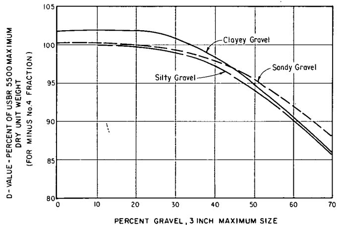
Figure 4. - Percent gravel versus D -value. 101-D-390
