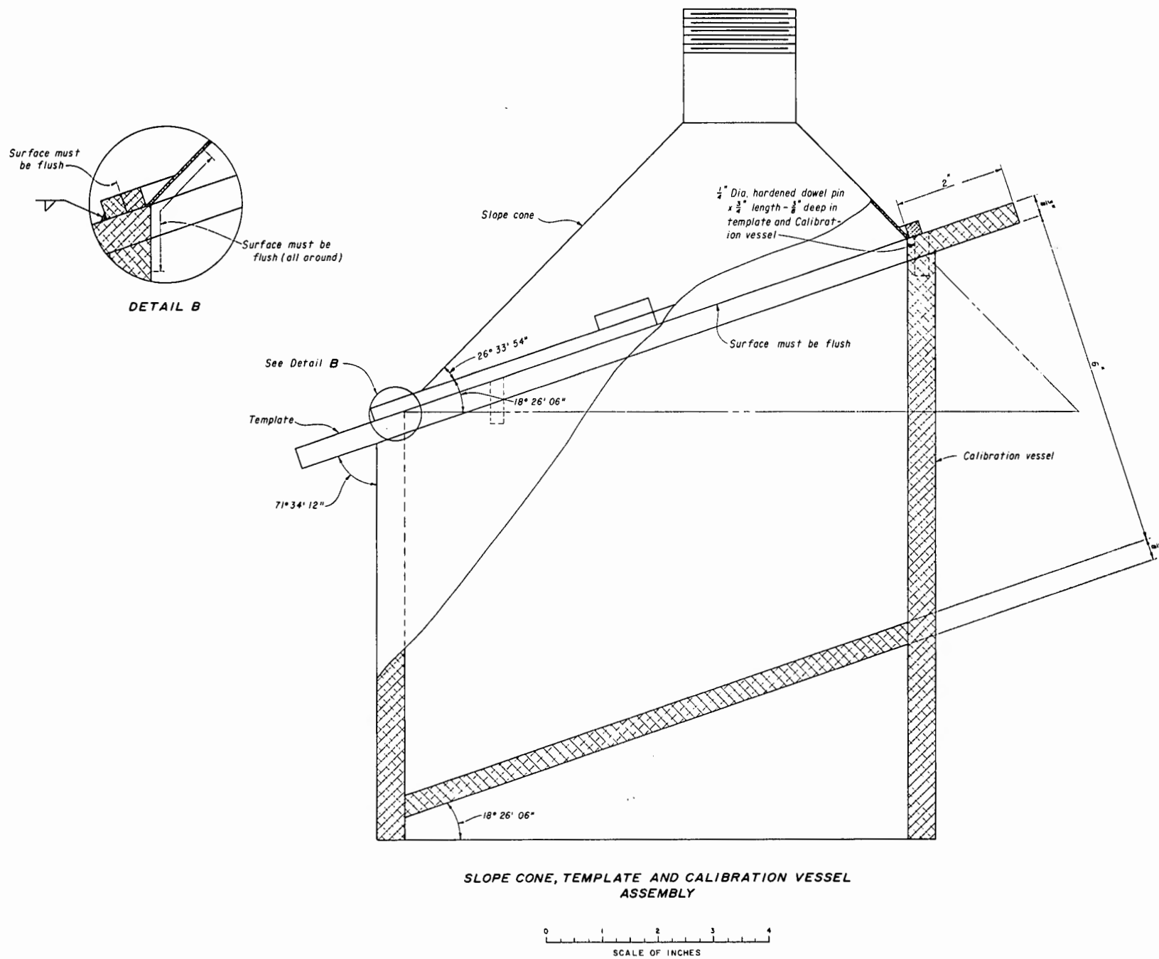
Figure 2. - Slope cone calibration vessel. (801-D-228)
