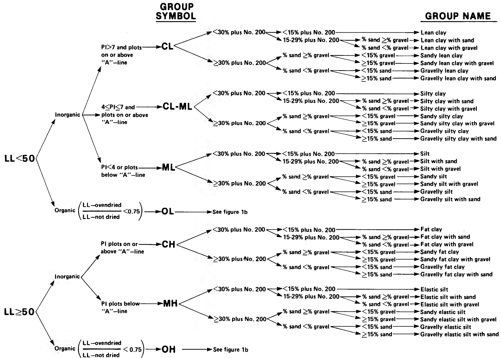
Figure 1a. – Flow chart for classifying inorganic fine-grained soils – laboratory method (50% or more passes No. 200 sieve).
