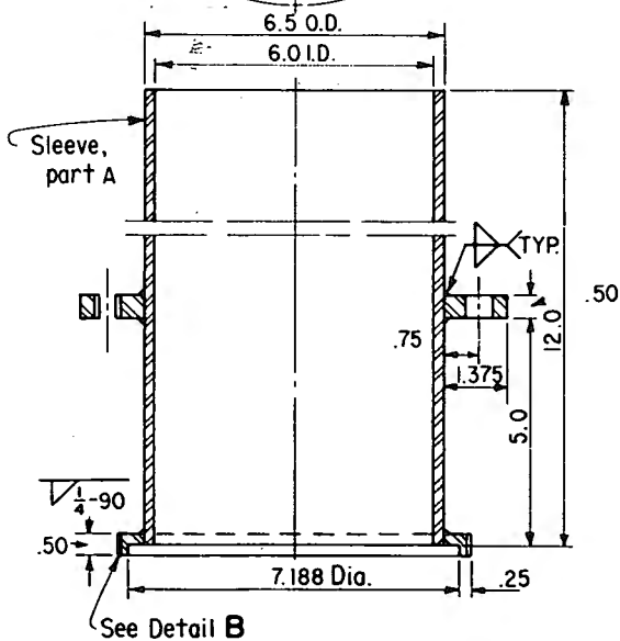
Figure 3. - Surcharge guide sleeve for 0.10 ft 3 (2831 cm 3 ) measure.
