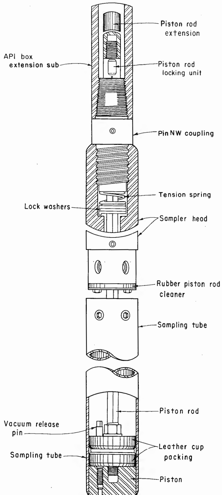
Figure 8. - Butters thin-wall fixed-piston sampler (Hvorslev type).
