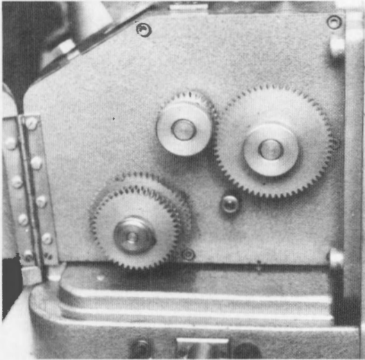
(a) Gear wheel combination for controlling the displacement rate.
