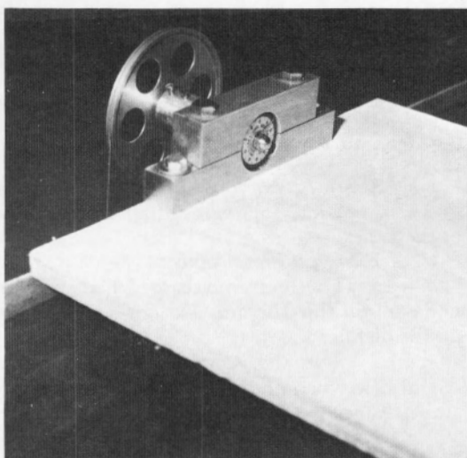
(a) Torvane, hub, and calibration wheel clamped in Torvane vise.
