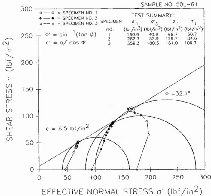
Figure 10. – Mohr's diagram—example.
