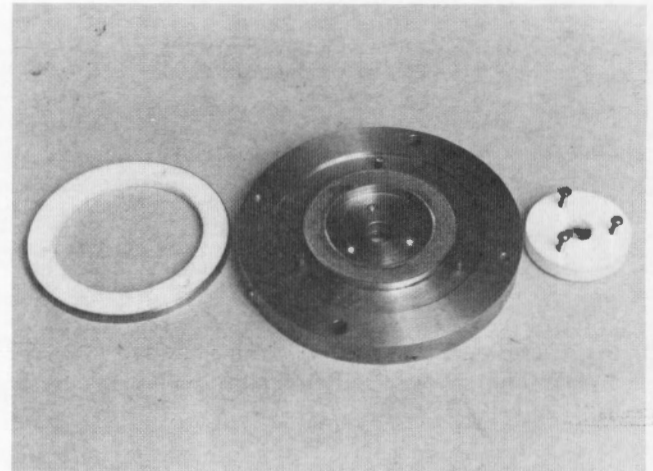
Figure 7. - The outer confining ring, lower platen, and inner confining disk from left to right.
