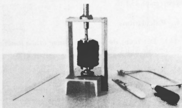
(a) Sample roughly trimmed and mounted in lathe.
