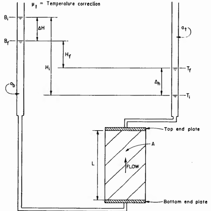
Figure X2.2.-Falling head permeameter with rising tailwater (flow from bottom end plate to top end plate).
