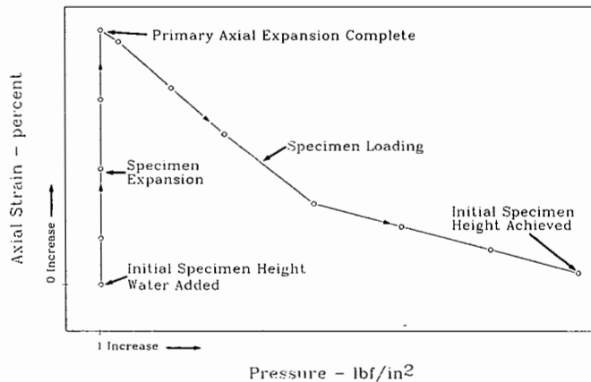
Figure 2. - Schematic of one-dimensional expansion test.
