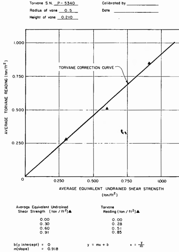
Figure 5. - Torvane correction curve — example.
