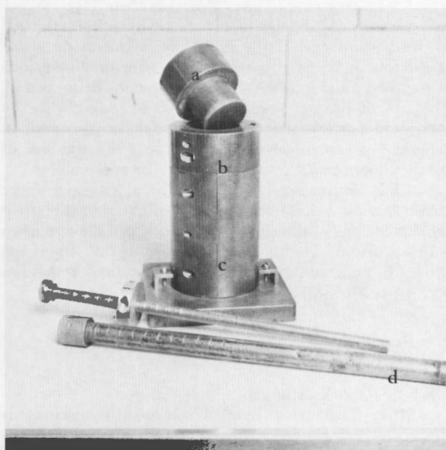
Figure 2.—Assembled split compaction mold (2.0-dia. by 5.0-in high). a) top plug, b) compaction collar, c) split compaction mold, and d) tampers.
