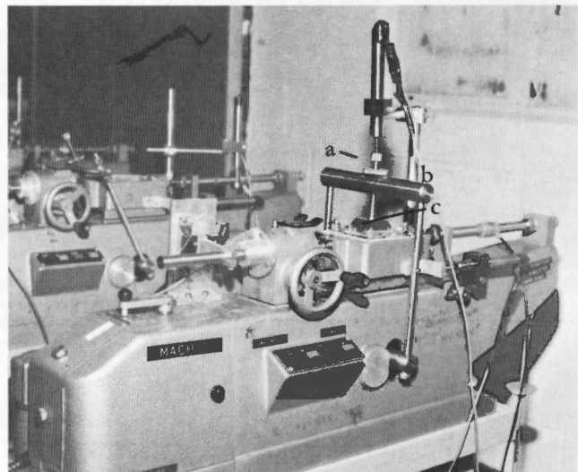
Figure 8. — Loading yoke in position for testing. (a) yoke adjustment screw, (b) loading yoke, and (c) load transfer plate.
