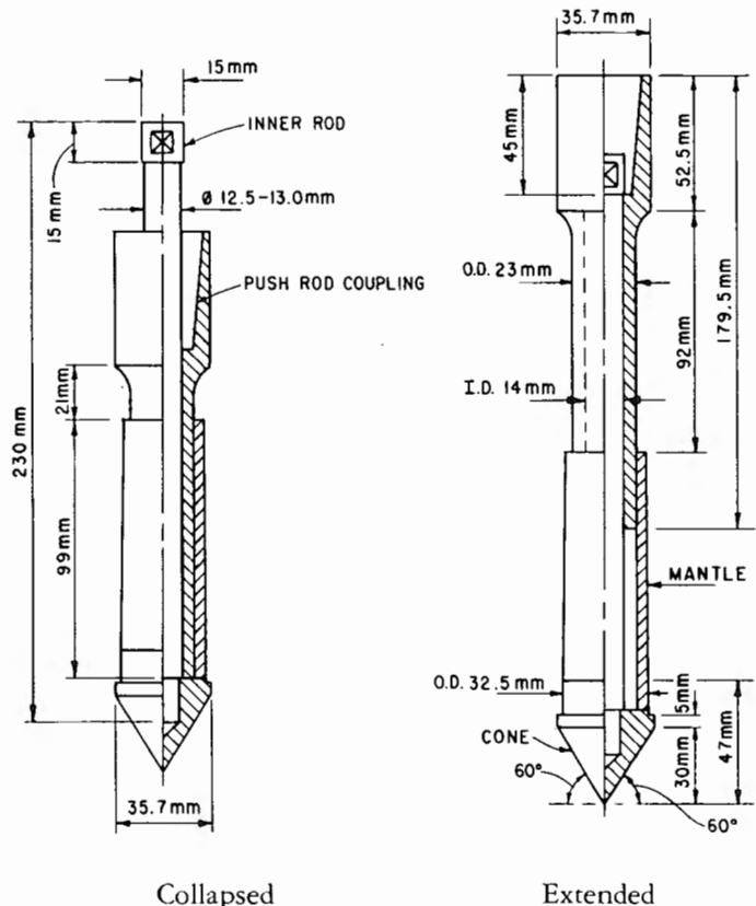
Figure 1. — Mechanical mantle cone penetrometer tip (Dutch mantle cone).
