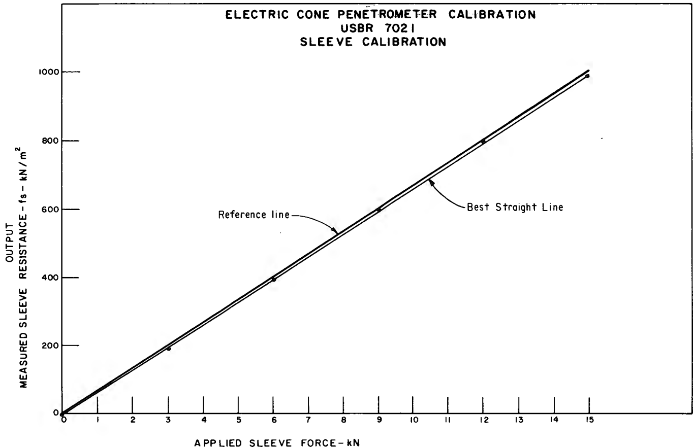
Figure A1.3. - Electric cone penetrometer sleeve calibration — example plot.
