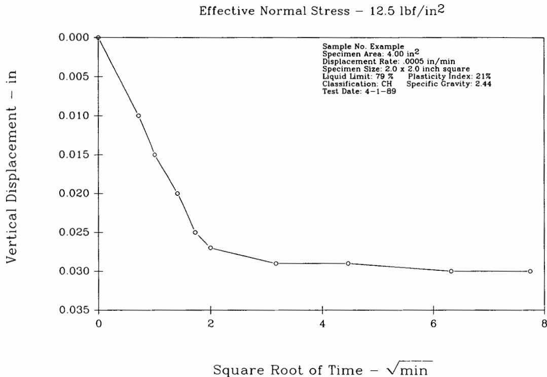
Figure 9. – Vertical displacement versus square root of time plot—example.
