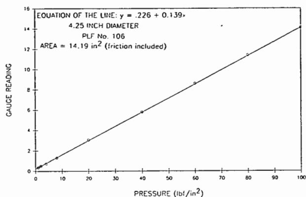
Figure X3.2.—Gauge reading versus applied pressure calibration (4.25-inch diameter specimen-low range) — example.
