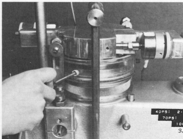
Figure 18. – Turning the horizontal support screws to center the outer confining ring on the specimen.
