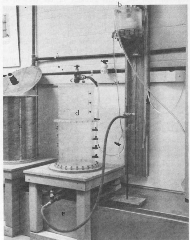
Figure 2. — Filter test cylinder system. a) aluminum test cylinder system, b) adjustable constant head tank, c) inflow plumbing, d) acrylic test cylinder system, and e) outflow plumbing.
