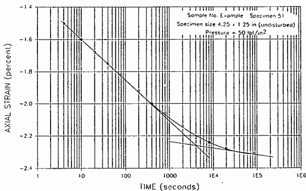
Figure 16. – Axial strain versus log-time — example.
