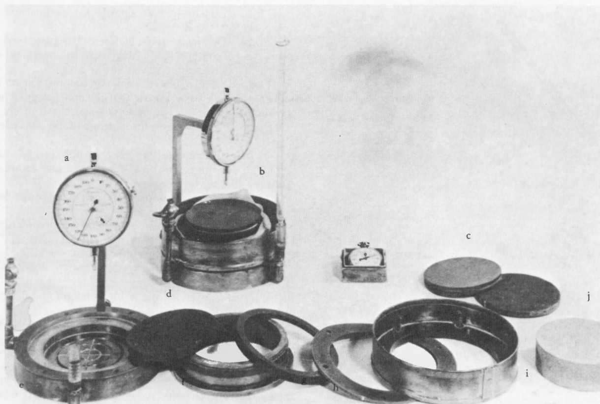
Figure 4. – Fixed-ring consolidometer. (a) dial gauge, (b) assembled consolidometer, (c) porous plates, (d) top load plate, (e) base plate, (f) specimen ring, (g) guide ring, (h) rubber gasket, (i) water collar with clamping ring, and (j) gauge block.
