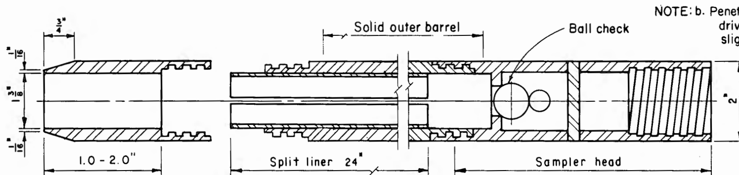
SOLID BARREL PENETRATION RESISTANCE SAMPLER
