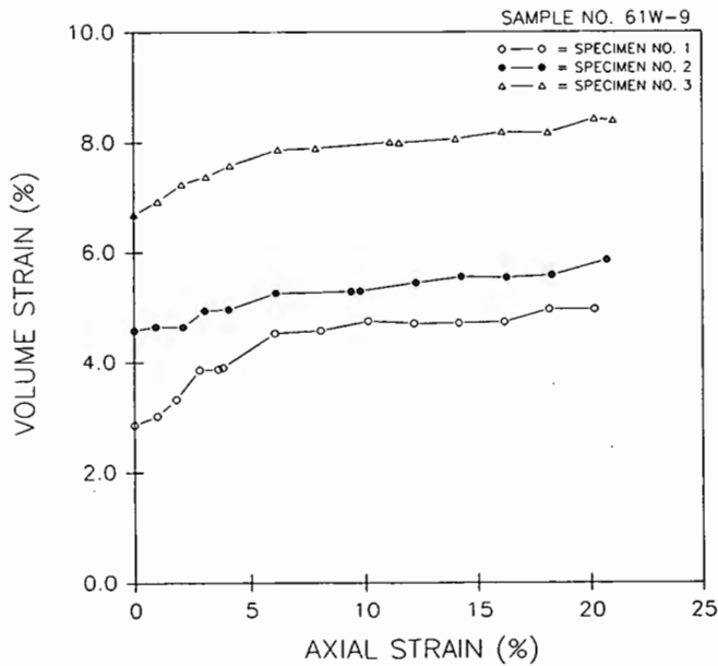
Figure 12. - Percent axial strain versus volume strain — example.
