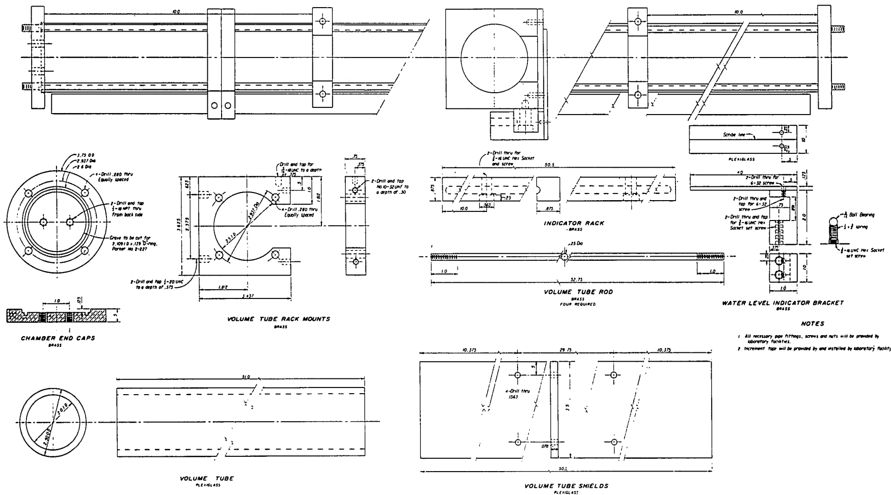
Figure X1.3.—Back-pressure permeability test—head tank—volume tube assembly details.
