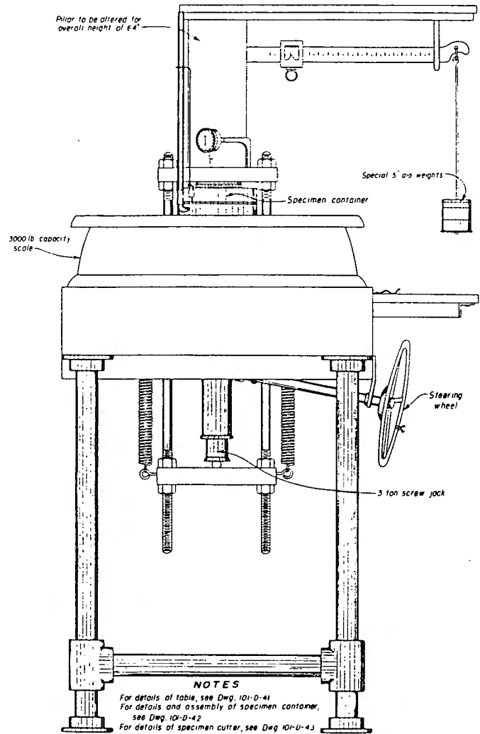
Figure 3. — Platform scale load frame with fixed-ring consolidometer in place. (101-D-40)
