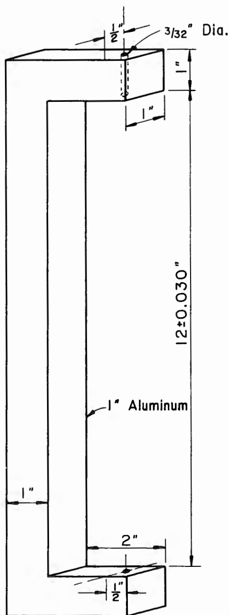
Figure X1.1. - Dial indicator reference bracket for 19-inch permeability cylinder.
