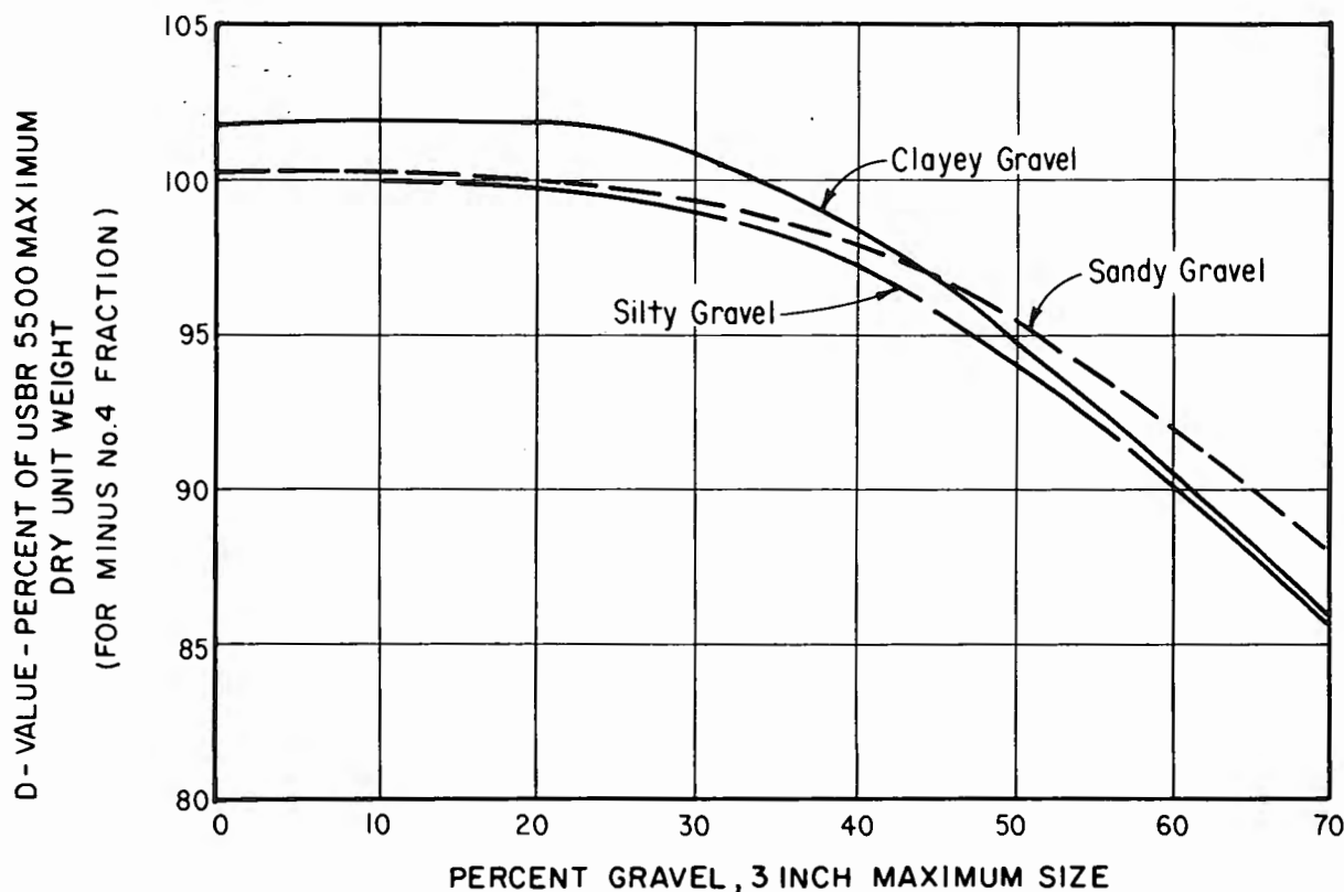
Figure 6. - Percent gravel versus D-value. 101-D-390
