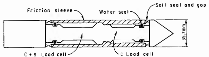
(b) Subtraction-type electric friction — cone penetrometer.
