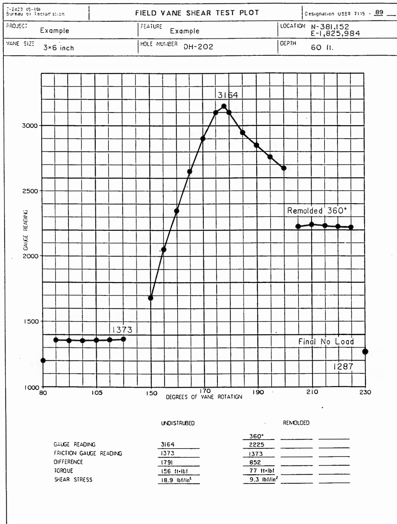
Figure 7. - Field vane shear test plot — example.
