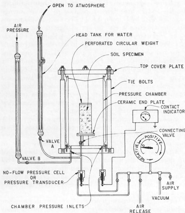
Figure 1. — Test chamber for measuring negative pore pressure by the exposed end plate method.
