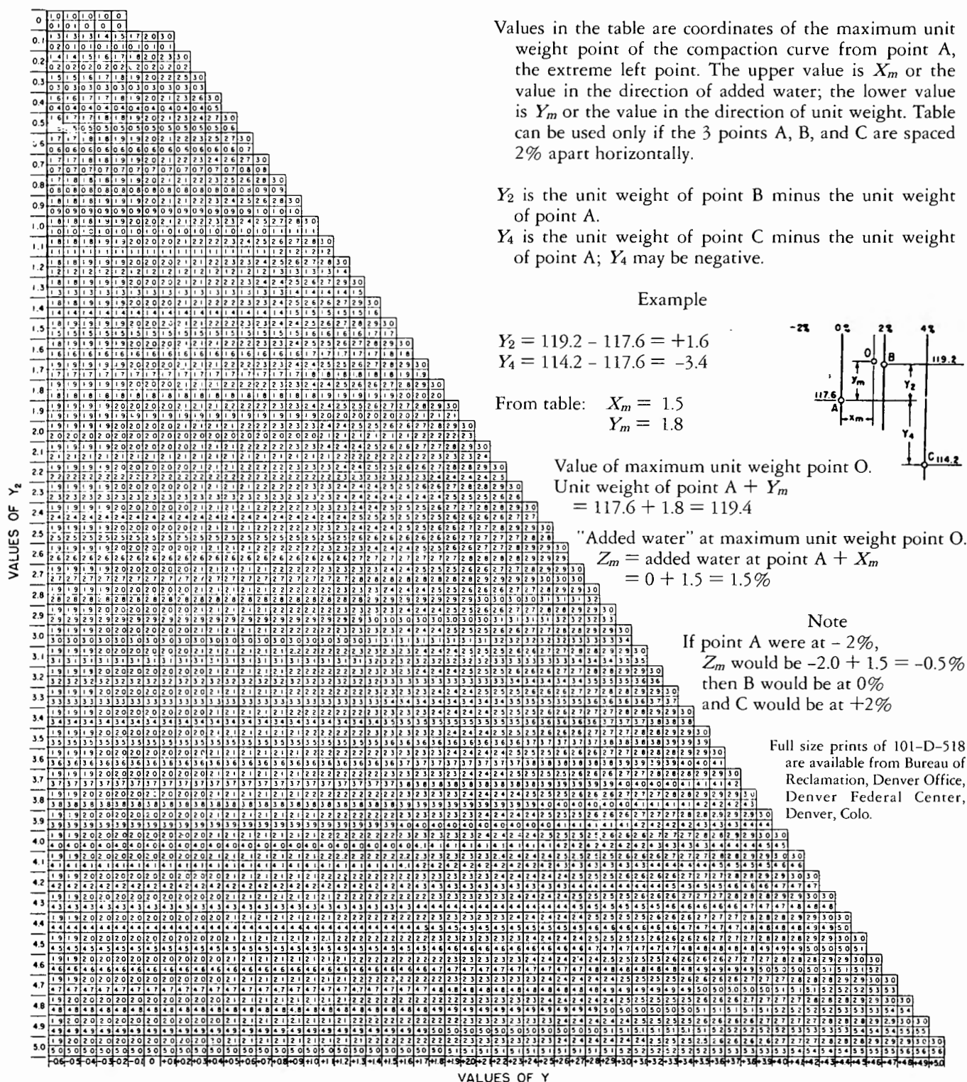
Figure 4. - Y_2/Y_4 Chart — rapid method of construction control - Continued.
