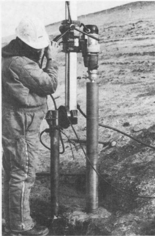
(a) View of coredrill set-up used for soil-cement coring.
