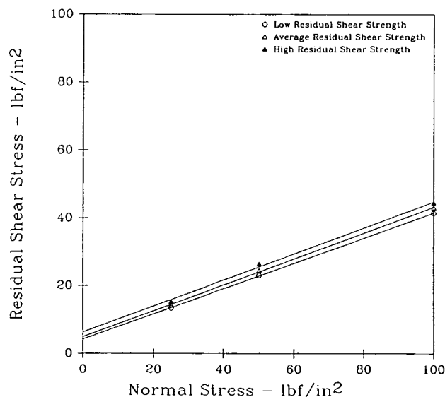
Figure 23. - Residual shear stress (average, low, high) versus normal stress plot (Feature: torsional shear) — example.
