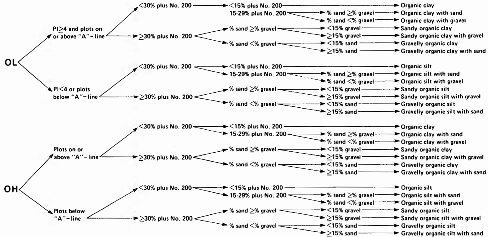
Figure 1b. – Flow chart for classifying organic fine-grained soils – laboratory method (50% or more passes No. 200 sieve).
