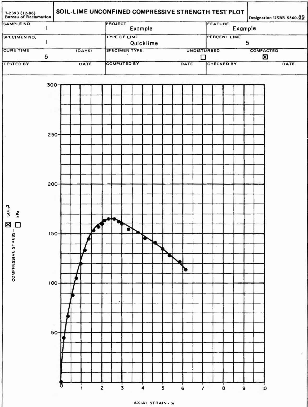
Figure 2A. - Soil-lime unconfined compressive strength test plot (in-lb example).
