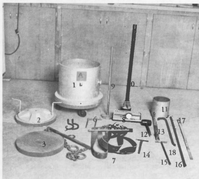
Figure 2. - Compaction equipment: 1) compaction mold, 2) loading plate with porous disc attached, 3) porous disc, 4) yoke — use to lift mold, 5) collar wrench, 6) modified spanner wrench, 7) four-point sling, 8) dial indicator with case, 9) small tamping hammer, 10) large tamping hammer, 11) 9-inch ring gauge, 12) rubber mallet, 13) straightedge, 14) scraper, 15) T-bar, 16) digging bar, 17) yardstick, and 18) pry bar.
