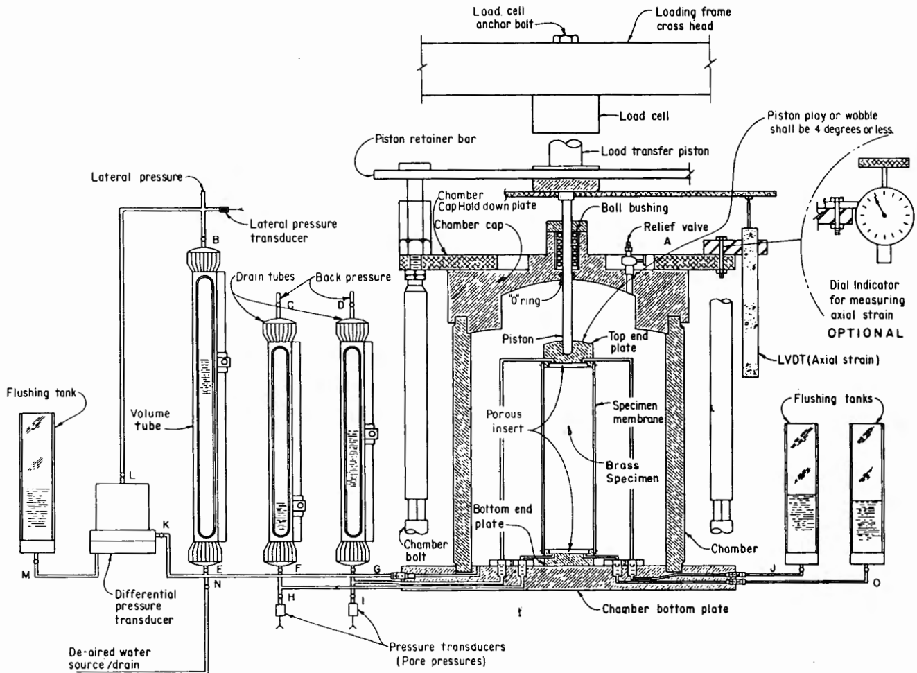
Figure 1. – Schematic of triaxial-type chamber assembly for pressure-volume change relations — calibration.
