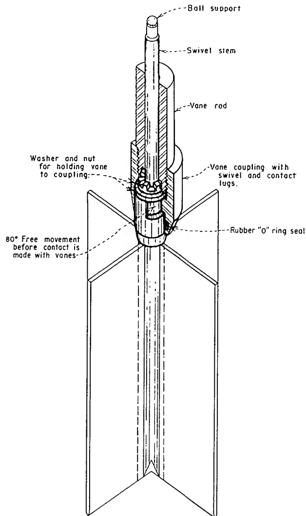
Figure 2. — Modified vane for friction determination.
