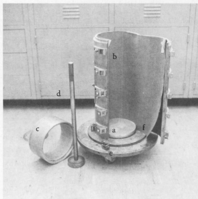
Figure 3.—Split compaction mold equipment (9.0-dia. by 22.5-in high). a) compaction pedestal, b) split compaction mold, c) compaction collar, d) tamper, e) baseplate, and f) paper liner.
