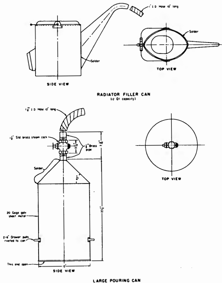
Figure 1. – Sand pouring devices. 101-D-341
