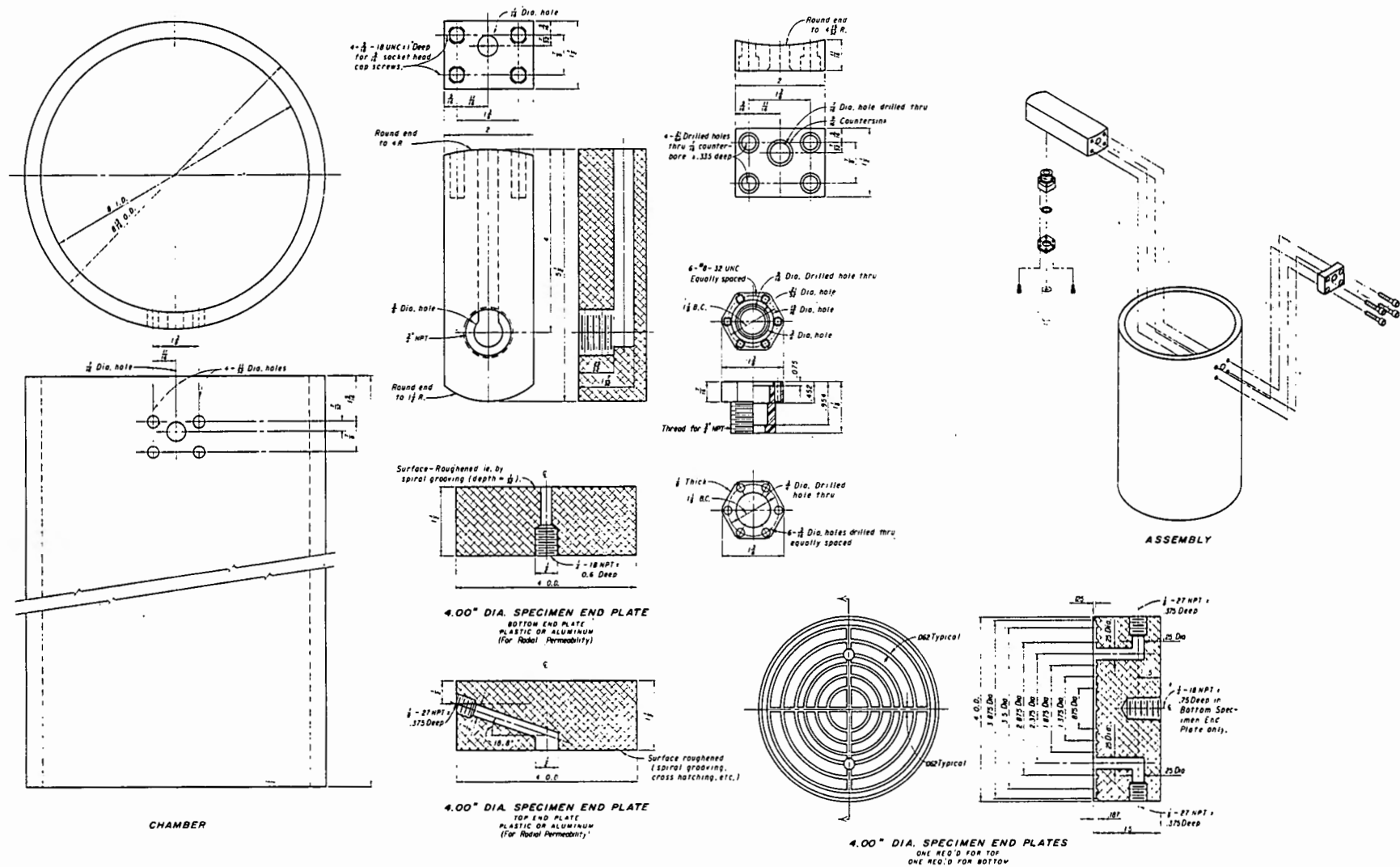
Figure X1.1.—Back-pressure permeability test chamber—details.
