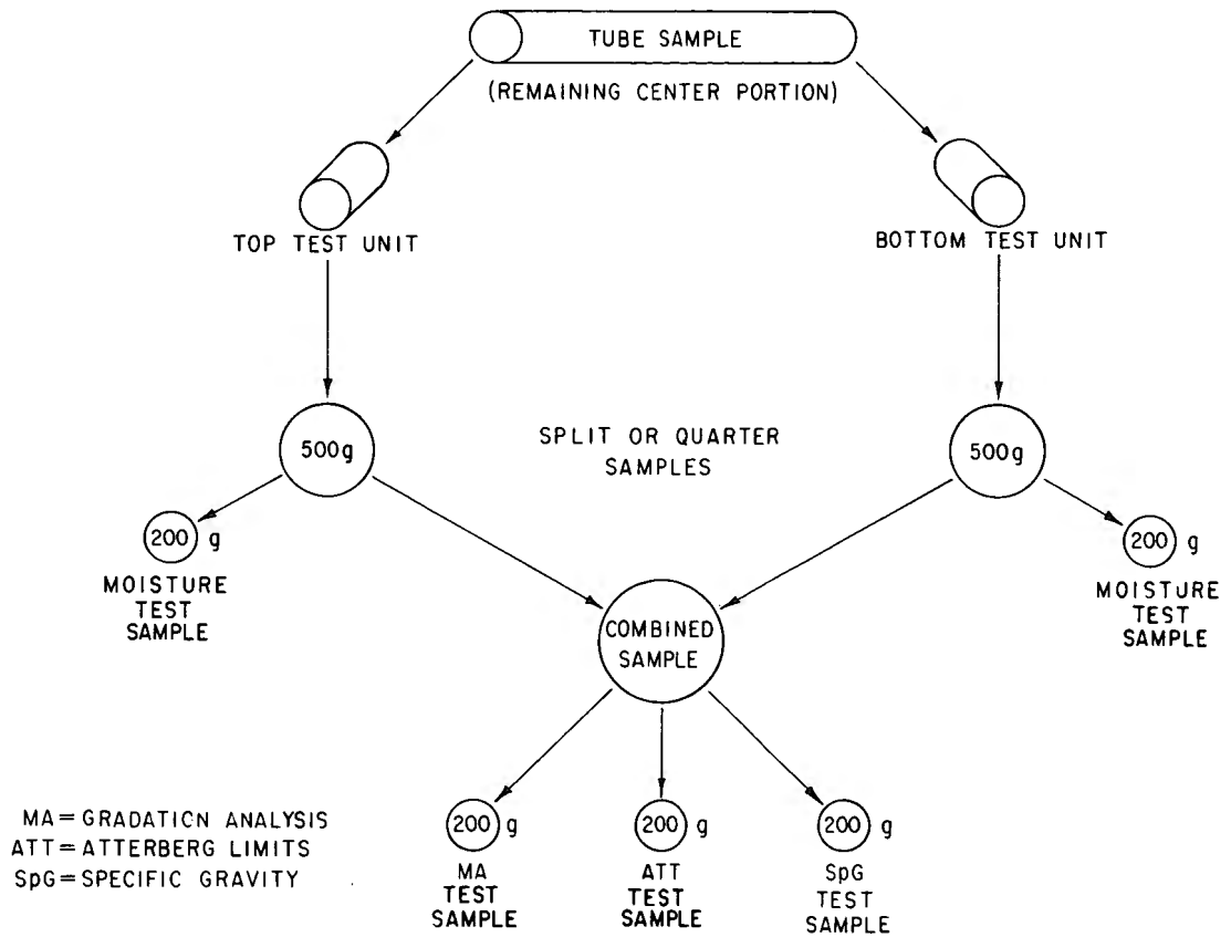
Figure 1. - Schematic of tube processing (similar material — minus No. 4).
