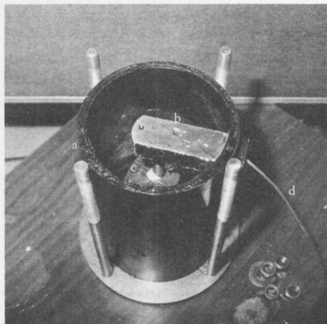
(b) Pressure chamber assembly. a) pressure chamber cylinder, b) LVDT support bracket, c) LVDT casing, and d) LVDT wiring harness.
