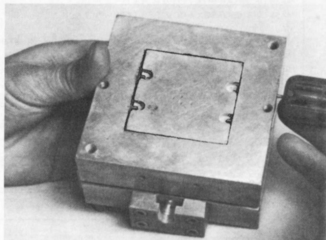
Figure 6. – Pushing in retaining pins over a correctly positioned lower plate.
