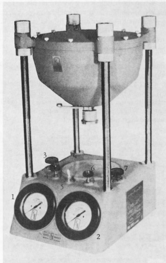
Figure 2. — Pneumatic load frame. (1) low range pressure gauge, (2) high range pressure gauge, (3) low range air control, (4) low range gauge shut-off, (5) load switch, (6) bleeder valve, (7) high range air control.
