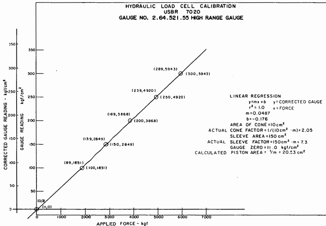
Figure A1.2. - Hydraulic load cell calibration — high range gauge example.
