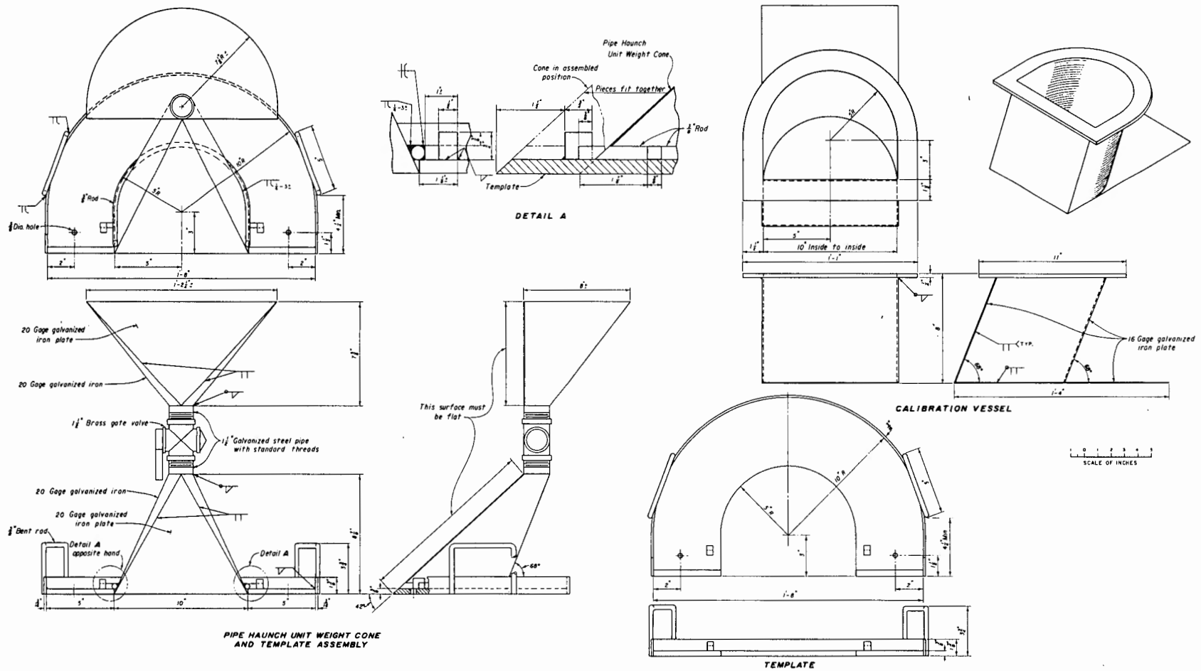
Figure 3. - Sand calibration measure for haunch cone. 801-D-223
