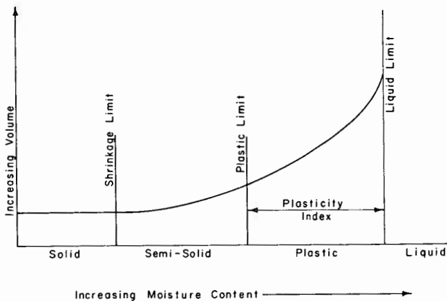
Figure 1. - Atterberg limits.
