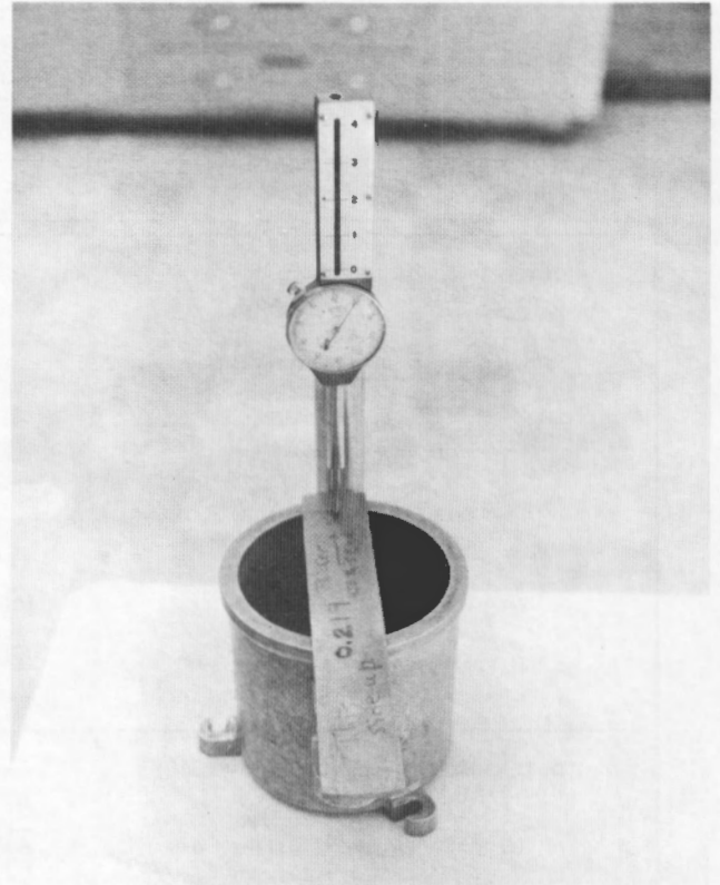
Figure 4. – Determination of reference dial reading constant.
