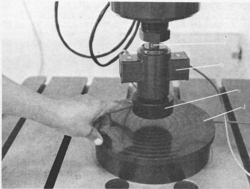
(a) Force transducer calibration using universal testing machine (compression). a) coupler, b) force transducer being calibrated, c) force transducer loading platen, and d) universal testing machine platform base.
