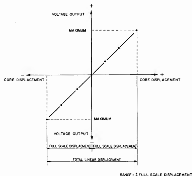
Figure 1. - Terminology of the LVDT.
