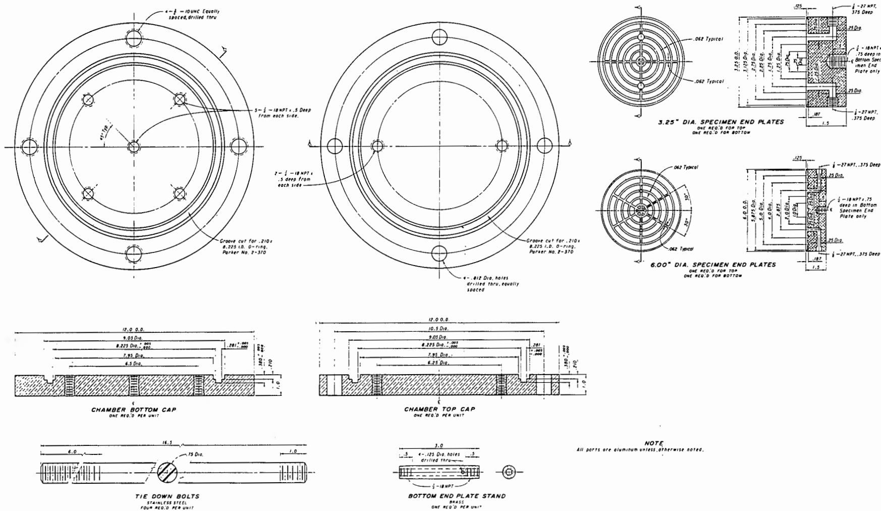
Figure X1.2.—Back-pressure permeability test chamber—details — Continued.
