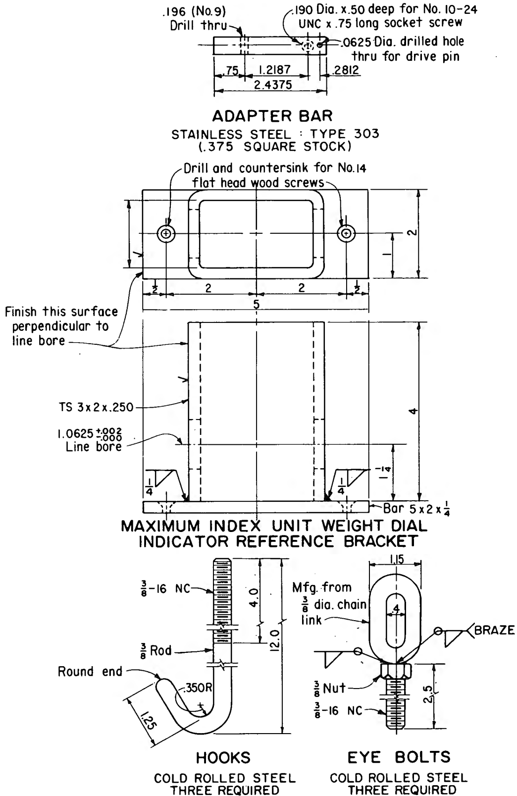
Figure 6. - Maximum index unit weight test equipment (sheet 2 of 4).
