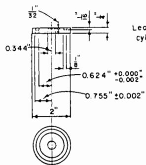
ANVIL (c)
