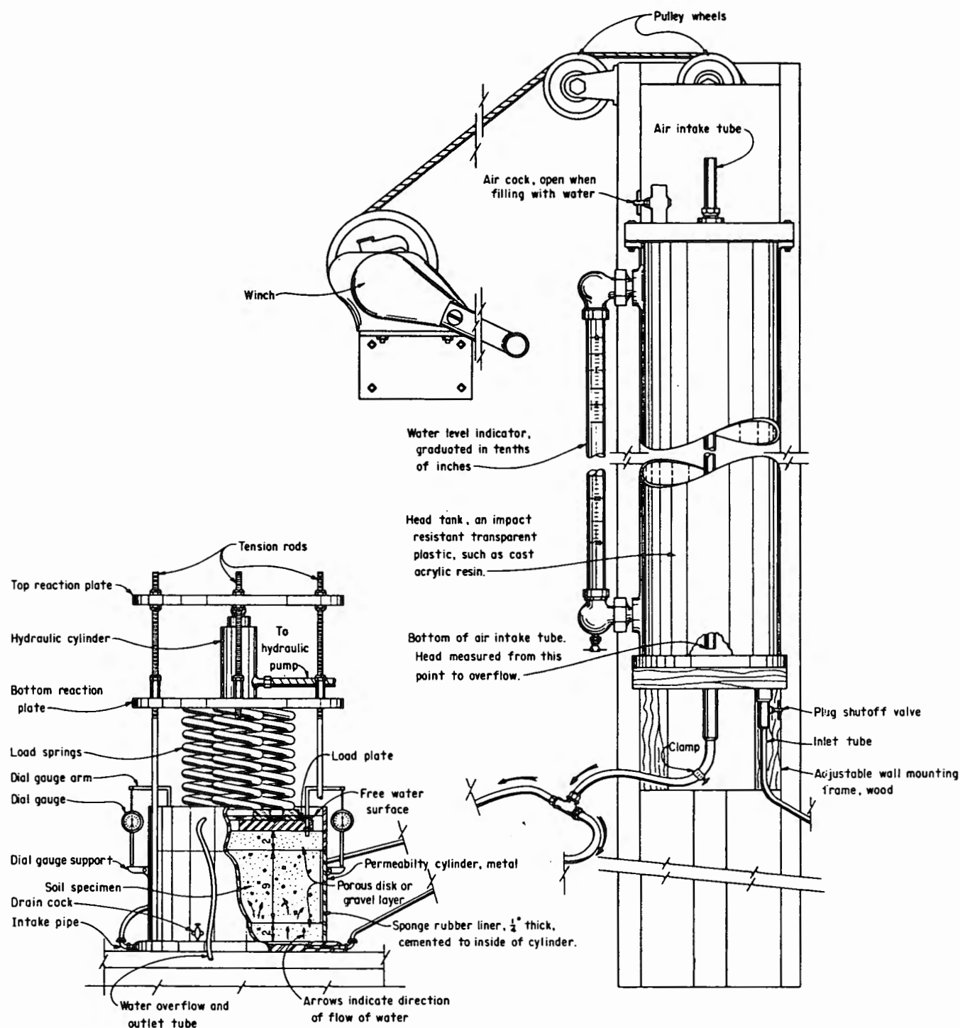
Figure 1. - 19-inch inside diameter permeability apparatus illustration.
