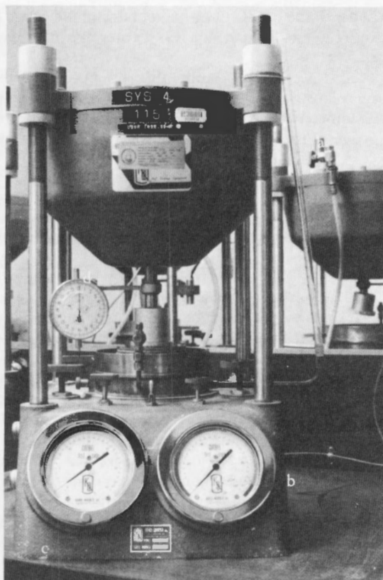
Figure 10. – One-dimensional consolidation test assembly. (a) saturation tube, (b) low range pressure gauge, (c) high range pressure gauge, (d) dial gauge.
