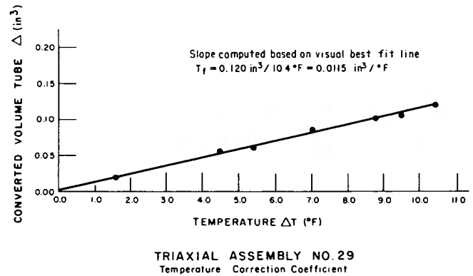
Figure X1.2. — Temperature correction coefficient plot — example.
