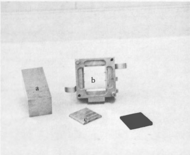
Figure 5.—Direct and repeated direct shear test specimen equipment. a) compaction tamper, b) shear box, c) baseplate, and d) porous plate.
