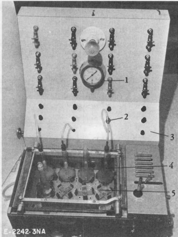
Figure 2. - Apparatus for determining apparent specific gravity. (1) vacuum gauge, (2) rubber tubing, (3) vacuum source, (4) specific gravity flask, and (5) constant temperature bath.
