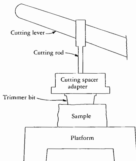
Figure 5. - Cutting assembly with soil sample.
