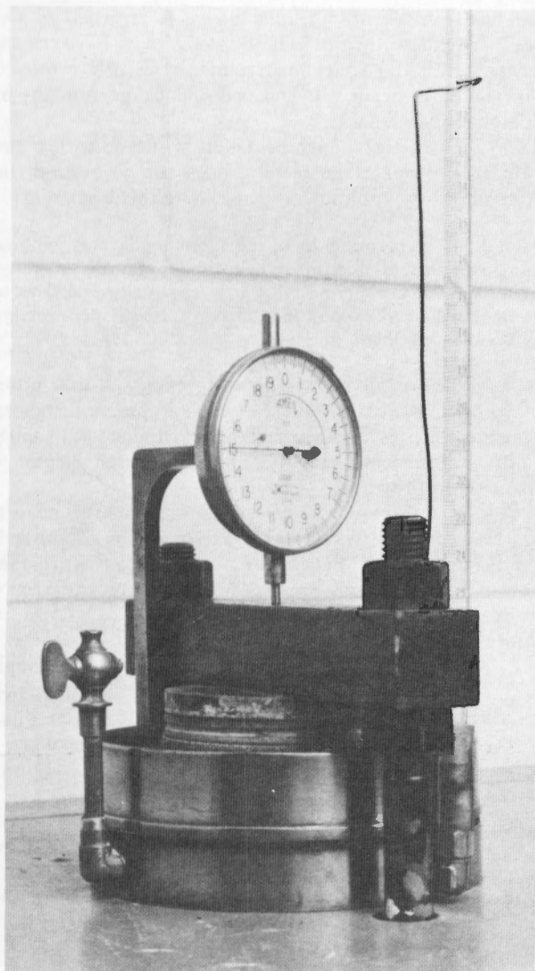
Figure 8. – Fixed-ring consolidometer with specimen placed in load frame.
