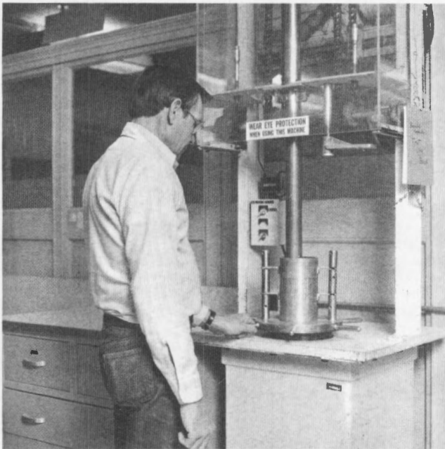
(b) Howard compactor
