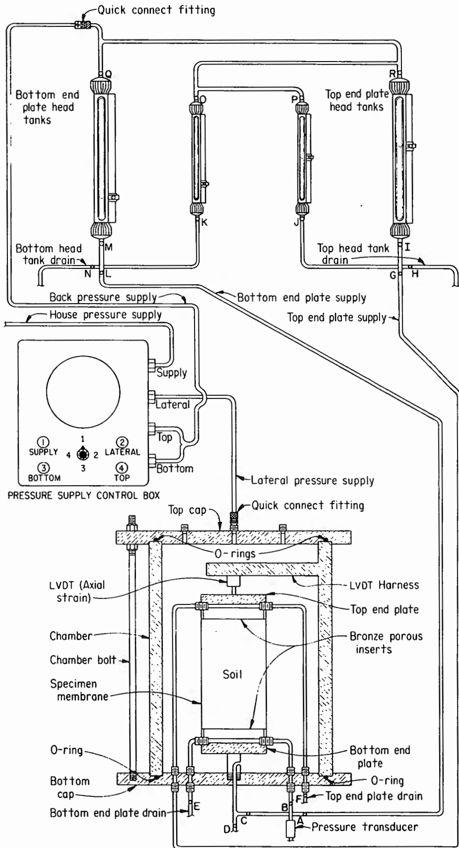
Figure 1. - Back pressure permeability schematic.
