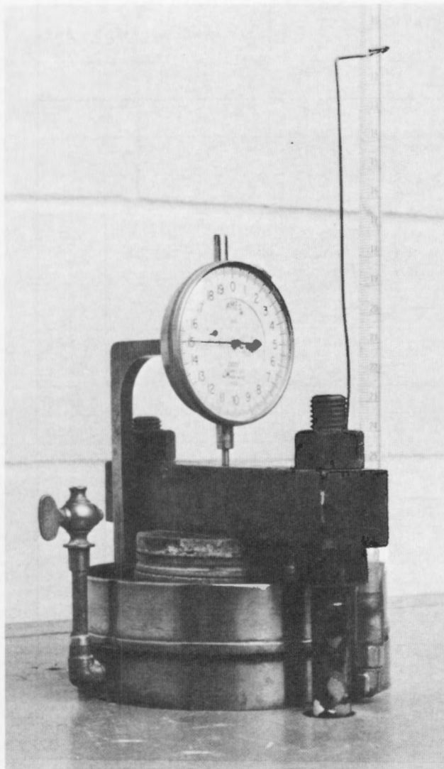
Figure 8. – Fixed-ring consolidometer with specimen placed in load frame.
