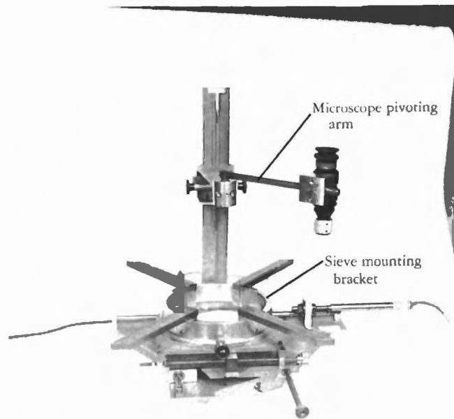
(a) Placement of Gilson™ sieve in sieve inspector.
