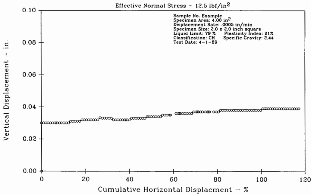
Figure 13. - Vertical displacement versus cumulative horizontal displacement plot—example.
