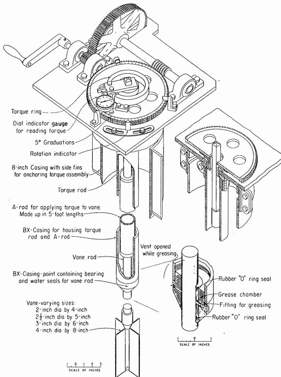
Figure 1. - Vane shear test apparatus.
