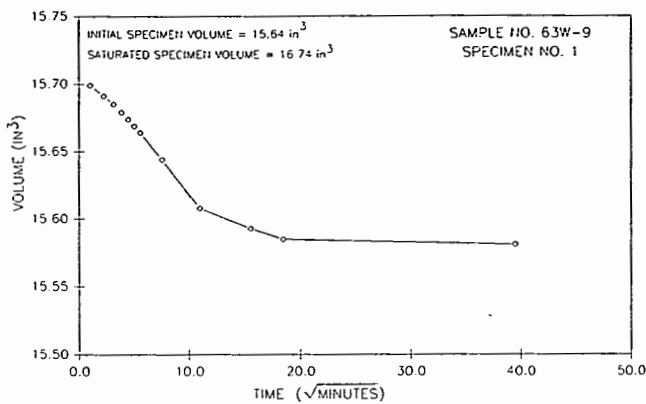
Figure 7. - Specimen volume versus square root of time — example.
