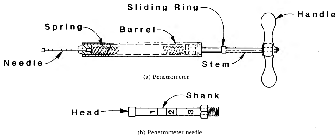
Figure 1. - Soil penetrometer.
