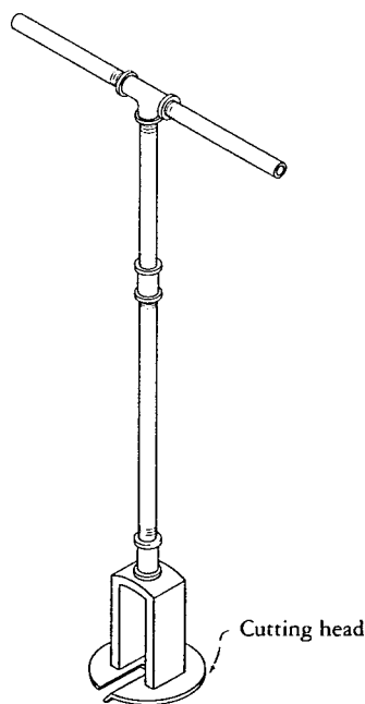
Figure 1. — Hand-operated trimming device (not drawn to scale). The diameter of the cutting head should be about 1/4 inch smaller than the inside diameter of the sample tube.
