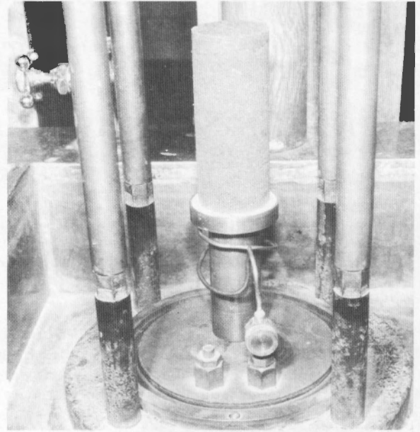
Figure 2. — Soil specimen on exposed ceramic end plate.
