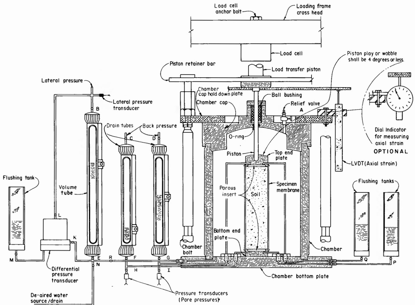
Figure 1. - Triaxial assembly for consolidated-drained tests.
