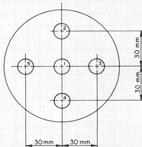
Figure 8. - Minimum spacing requirements for vane shear testing — minimum of three test locations required.
