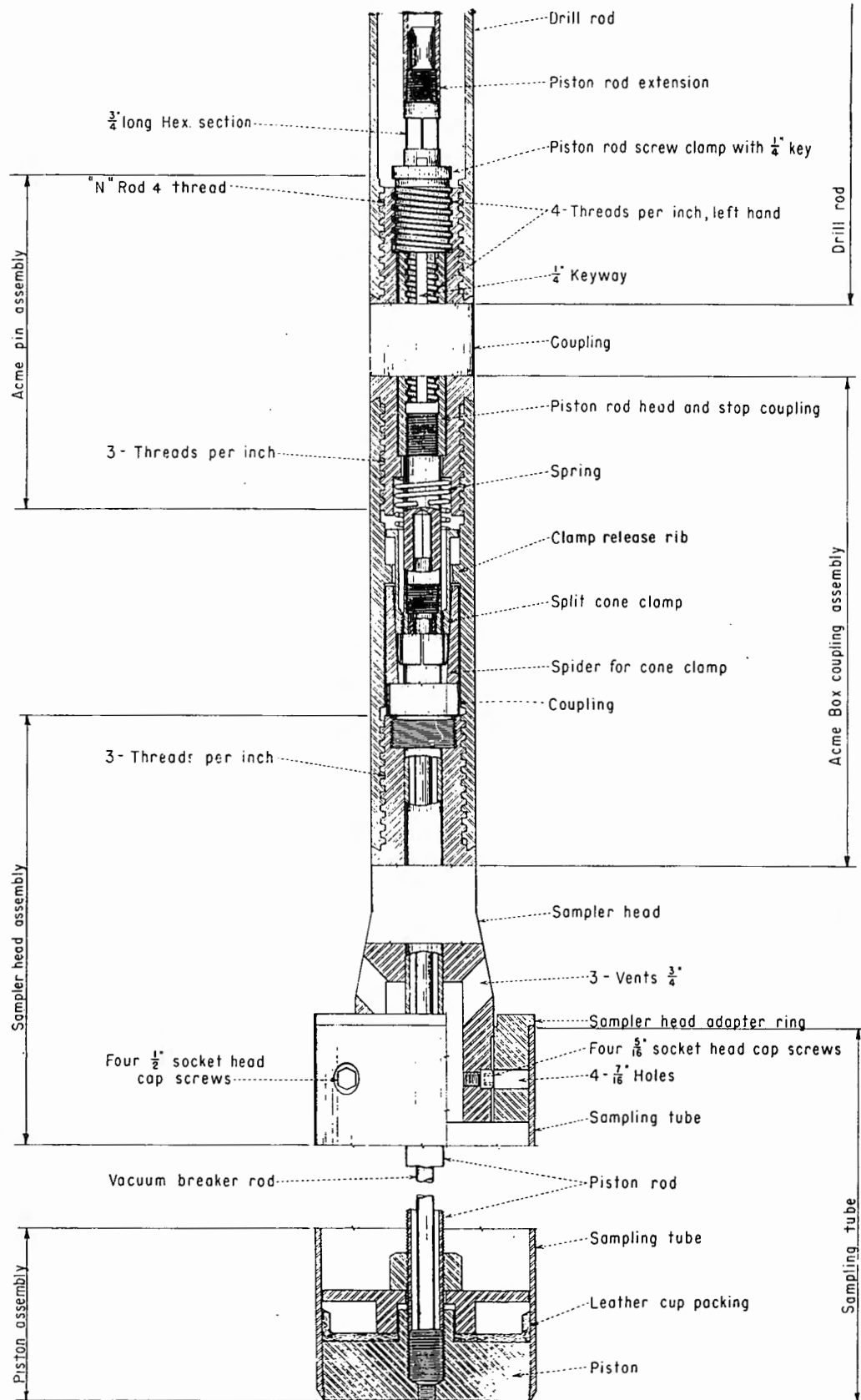
Figure 6. - Thin-wall fixed-piston sampler (Hvorslev type).
