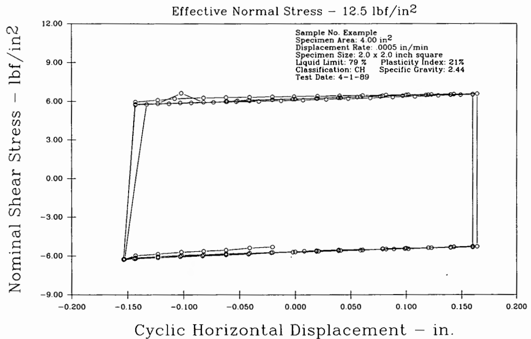
Figure 12. - Nominal shear stress versus cyclic horizontal displacement plot—example.
