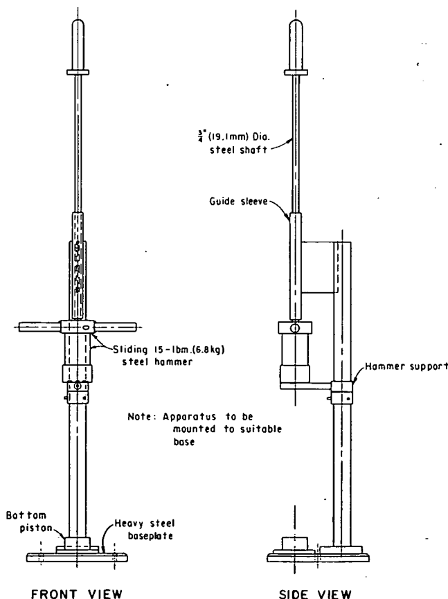
Figure 1. – Dropping-weight compacting machine.
