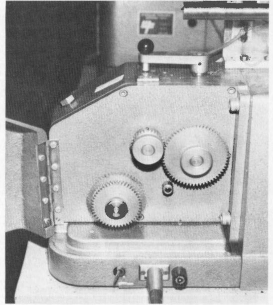
(a) Gear wheel combination for controlling the displacement rate.
