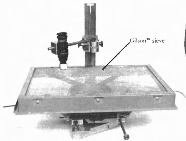
(a) Placement of Gilson™ sieve in sieve inspector.
