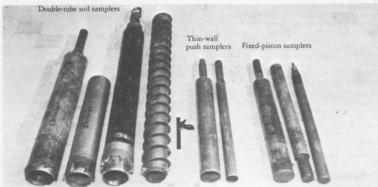
Figure 1. — Examples of undisturbed soil samplers.
