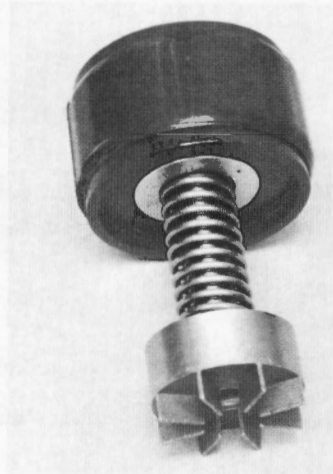
(b) Side view. Note vane at bottom.
