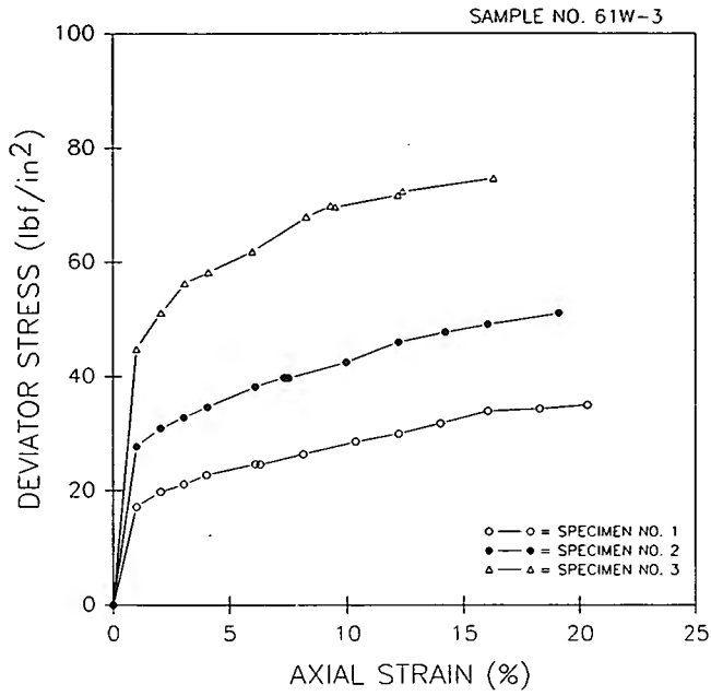
Figure 11. - Percent axial strain versus deviator stress—example.
