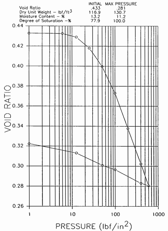
(b) Void ratio versus log of pressure.
