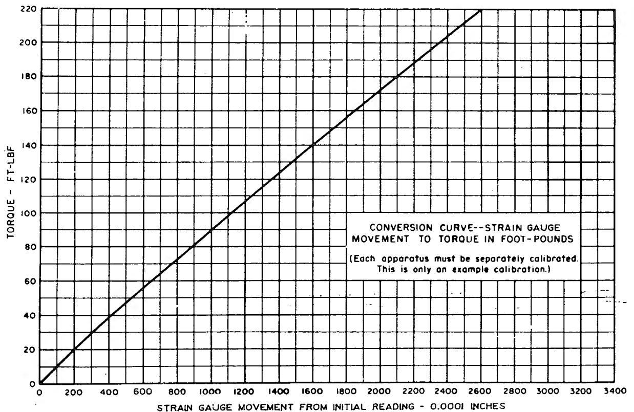
Figure 3. – Typical calibration curve for a vane shear test apparatus.
