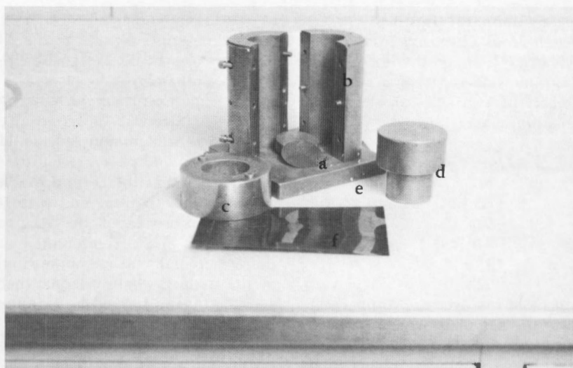
Figure 1.—Split compaction mold equipment (2.0 in diameter by 5.0 in high). a) compaction pedestal, b) split compaction mold, c) compaction collar, d) top plug, e) baseplate, and f) film liners.
