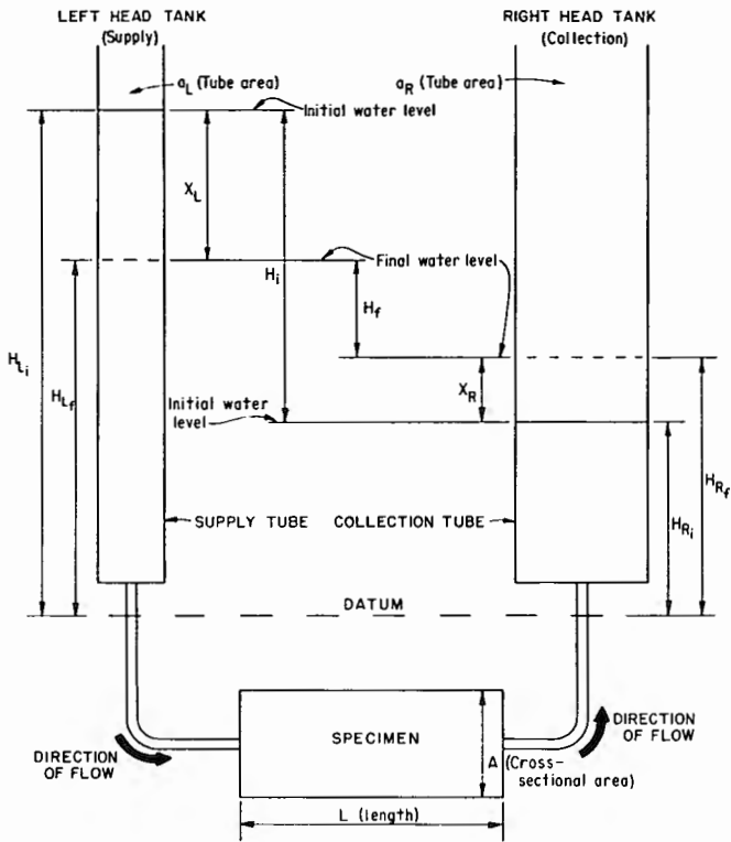
Figure X2.1.-Falling headwater-rising tailwater permeability test schematic.
