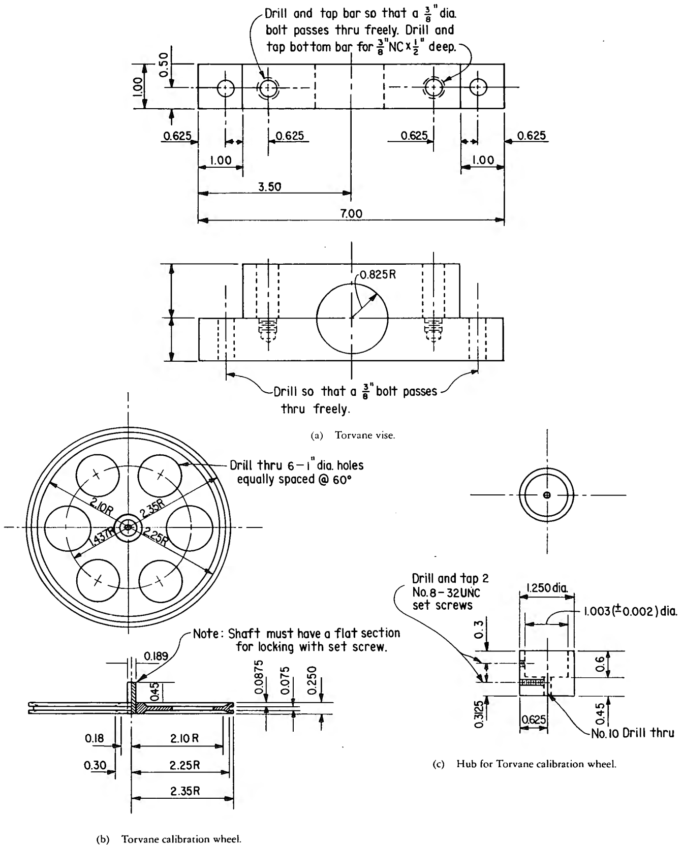
Figure 3. - Torvane calibration assembly.
