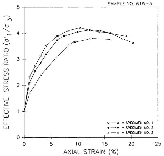
Figure 14. - Percent axial strain versus effective stress ratio—example.
