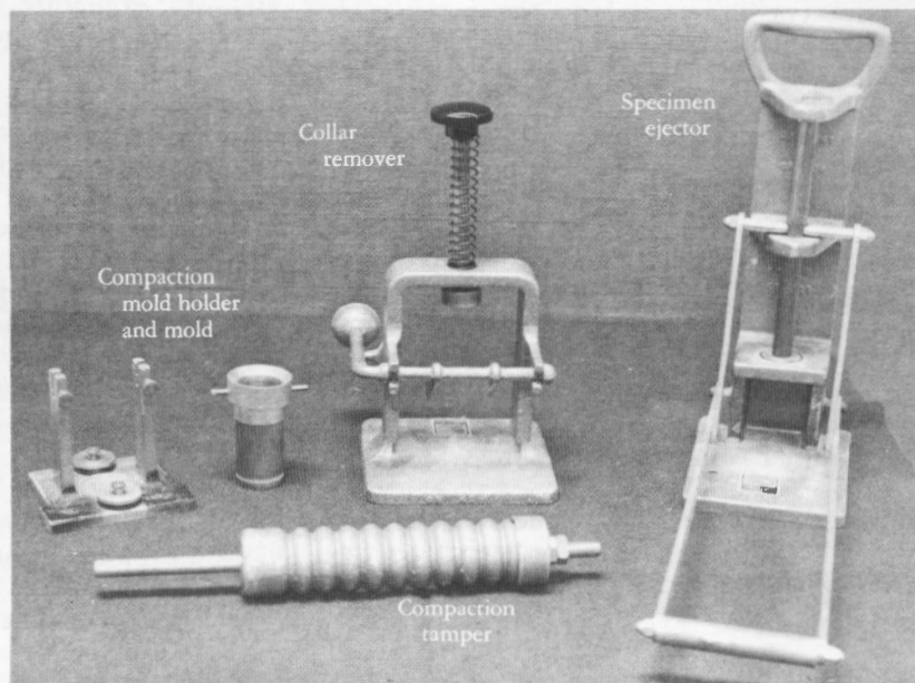
Figure 1. — Harvard miniature compaction test equipment.
