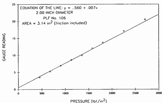
Figure X3.5.—Gauge reading versus applied pressure calibration (2.00-inch diameter specimen-high range) — example.
