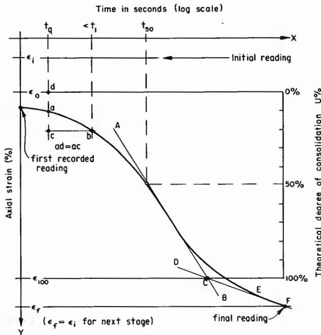
Figure X1.1.—Percent axial strain versus log time (log method) — example.
