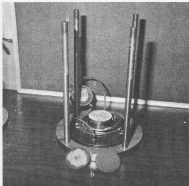
(a) Pressure chamber components-exposed. a) top cap tie down rods (4), b) bronze porous inserts, c) top end plate, and d) bottom end plate.
