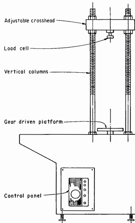
Figure 2. — Compression test machine.
