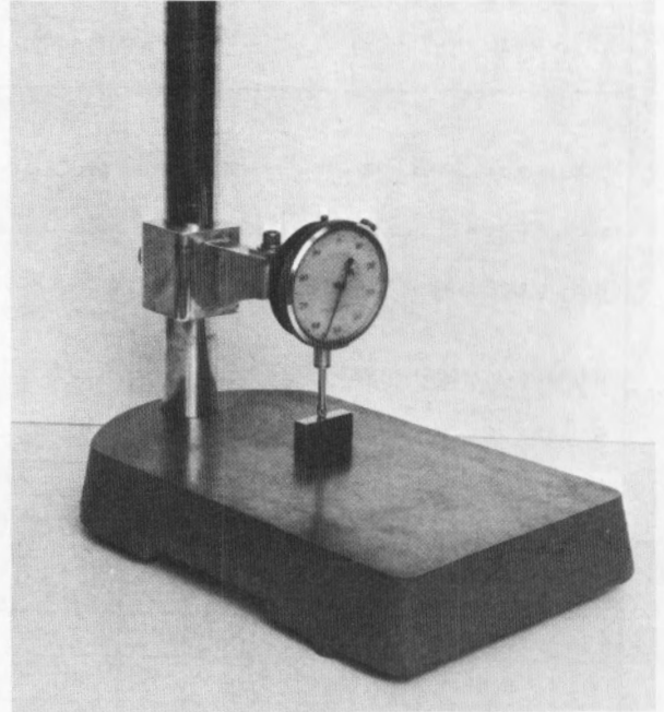
(b) Displacement of dial indicator with gauge block.
