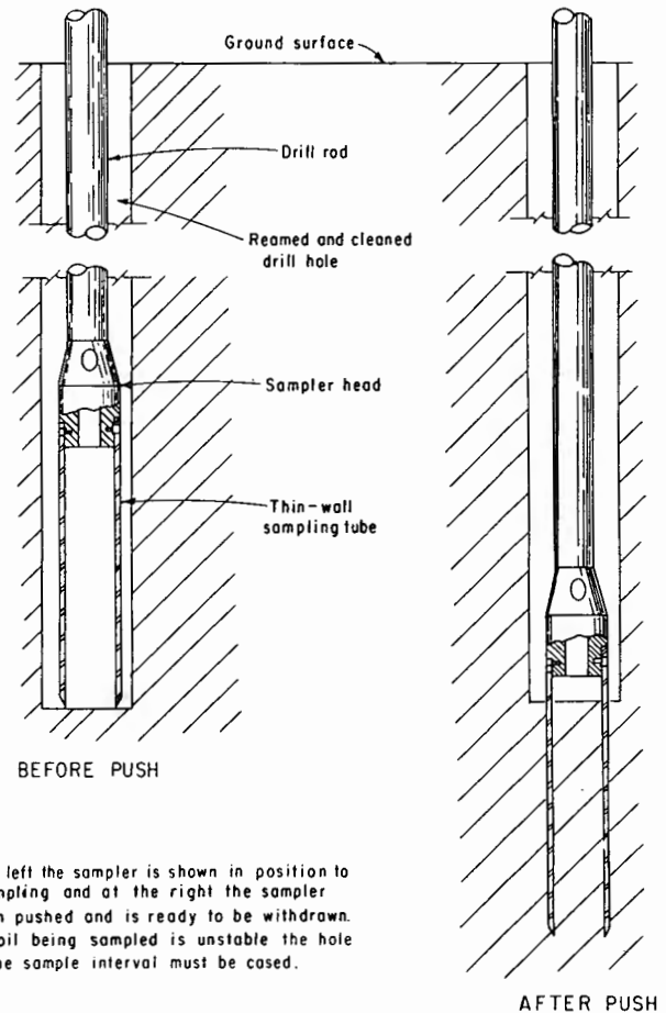
Figure 3. - Sampling with thin-wall push tube sampler.
