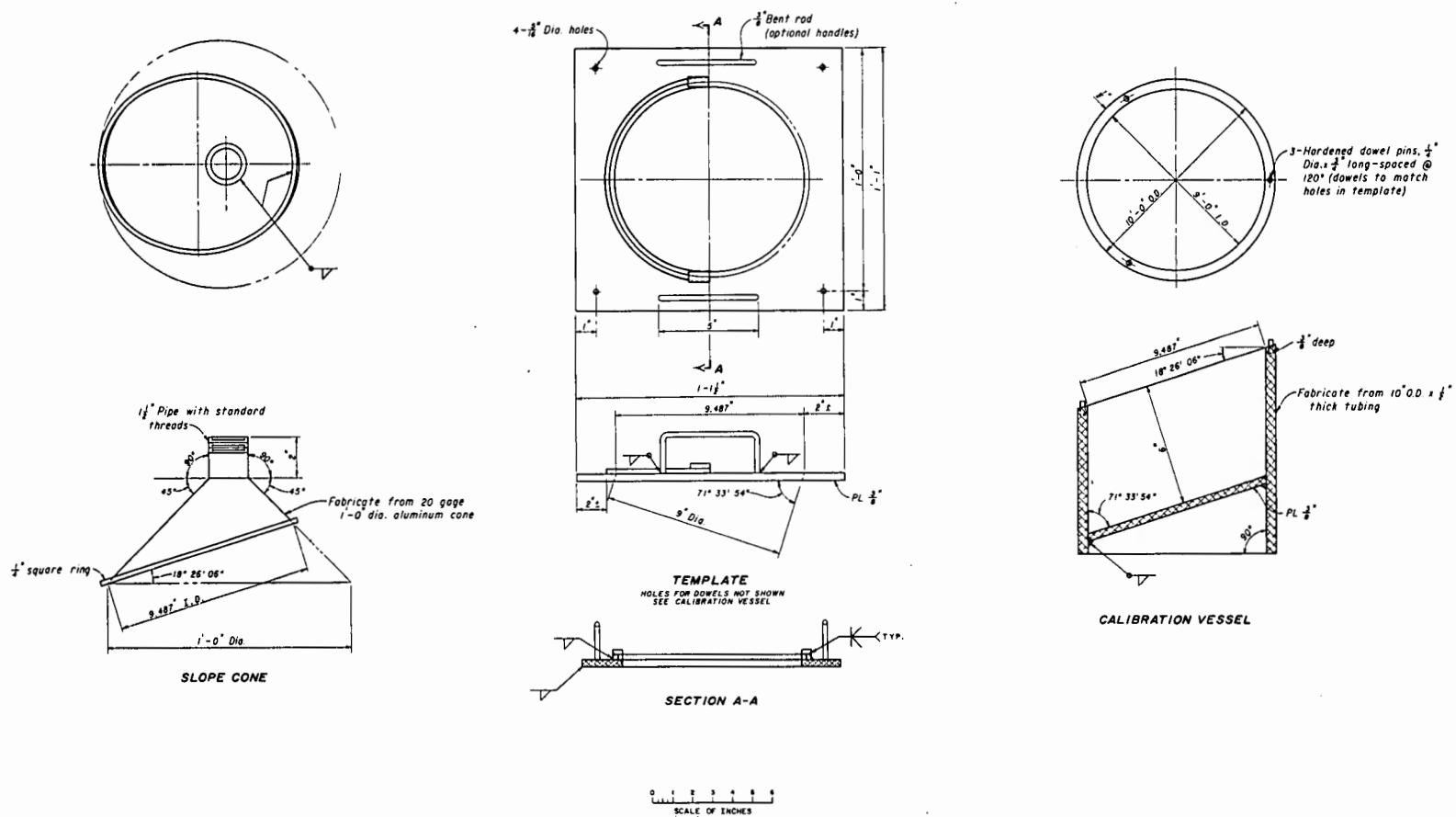
Figure 2. - Sand calibration measure for slope cone 801-D-227
