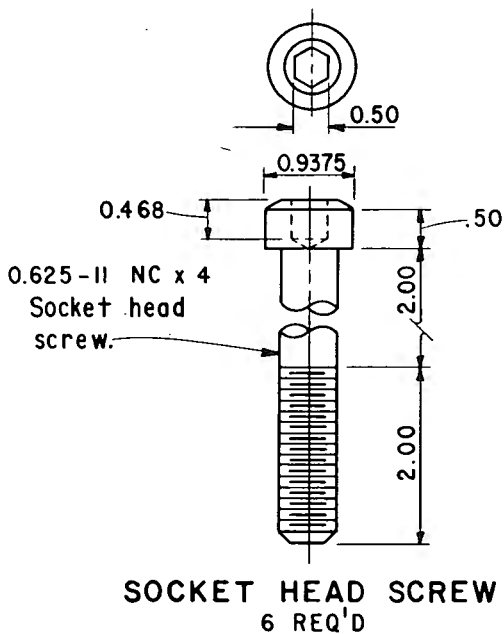
Figure X2.2. - Vibratory table calibration equipment — Continued. 101-D-647
