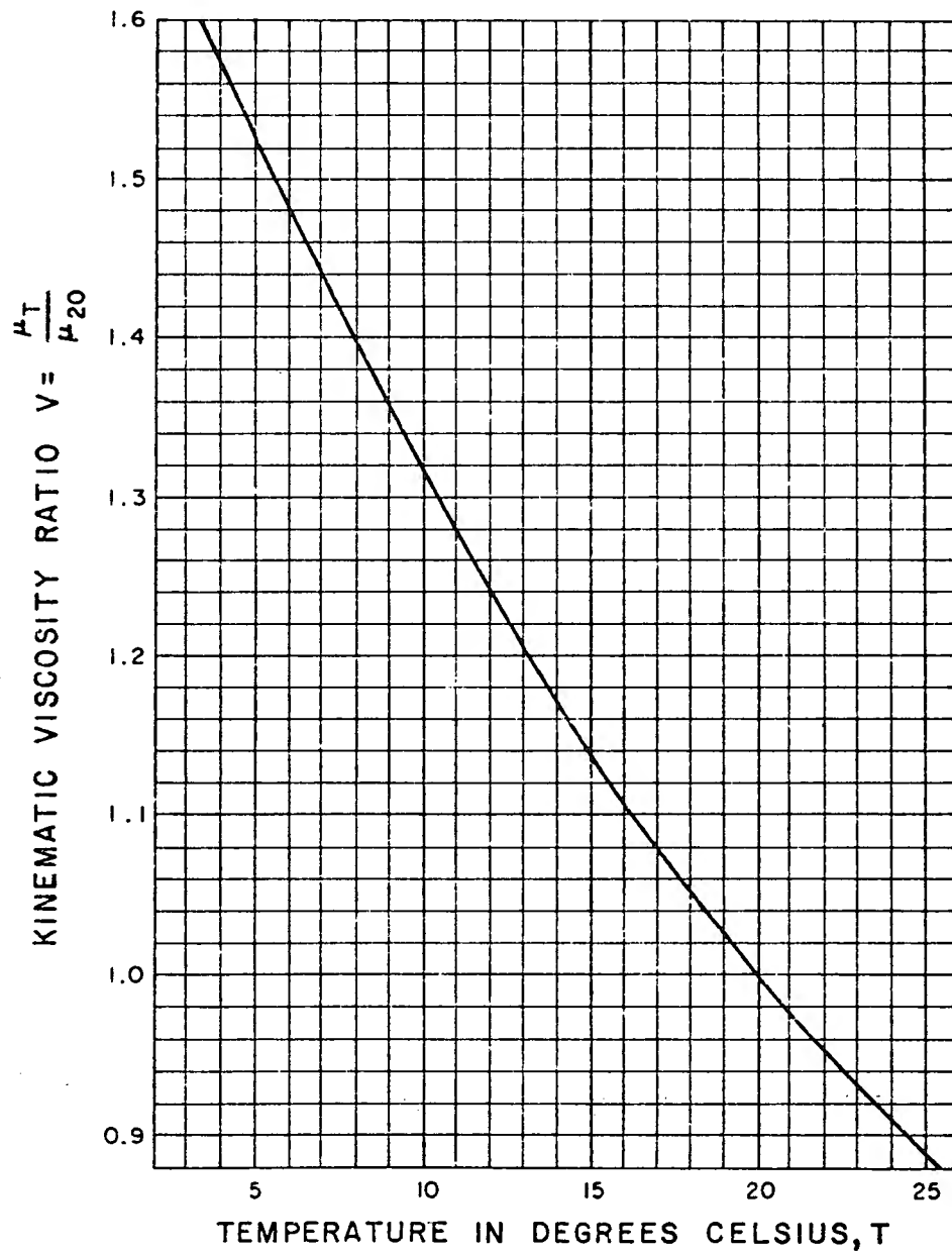
Figure 5. - Relationship between kinematic viscosity ratio of water and temperature.
