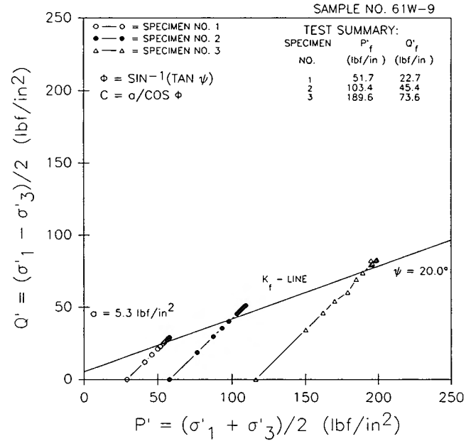
Figure 9. - p' - q' diagram — example.
