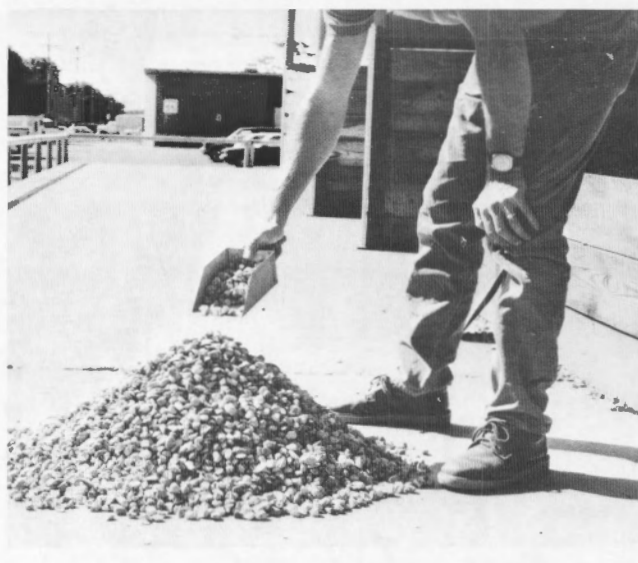
Figure 4. – Placement of soils greater than 3/8-inch maximum particle size while maintaining a 1-inch free fall height. The pouring device shown is a small scoop.
