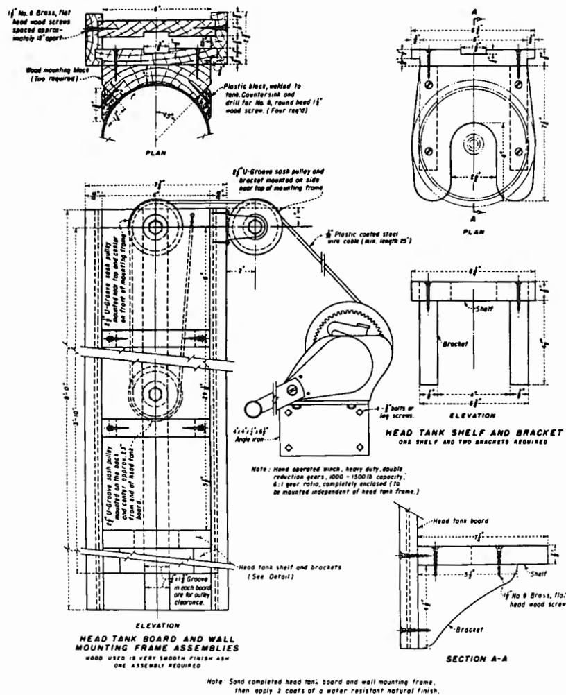
Figure X1.3. - 19-inch inside diameter permeability apparatus — Plexiglas head tank and mounting frame. 101-D-193
