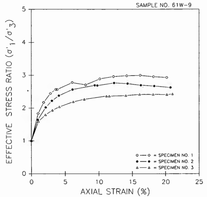
Figure 13. - Percent axial strain versus effective stress ratio — example.
