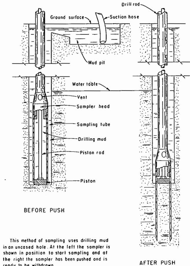
Figure 7. – Sampling with fixed-piston sampler (Hvorslev type).
