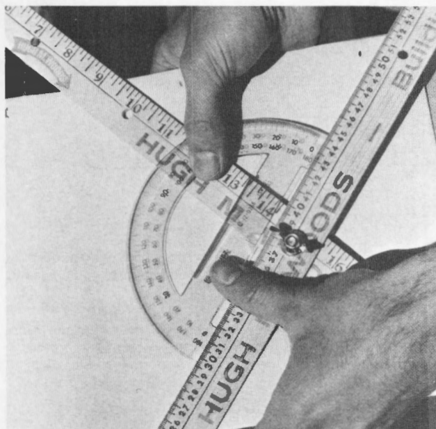
Figure 8. – Measuring the vertex angle using a protractor.
