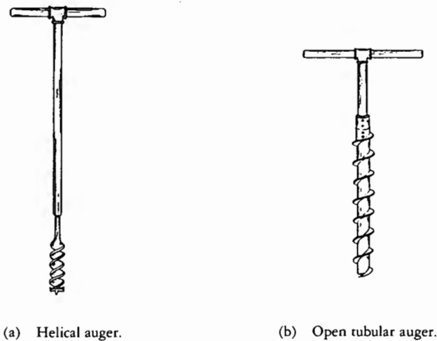
Figure 1. – Hand augers.
