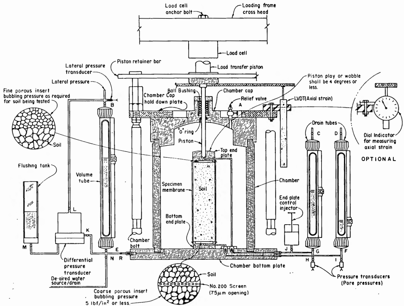
Figure 1. – Triaxial assembly for unconsolidated-undrained tests.
