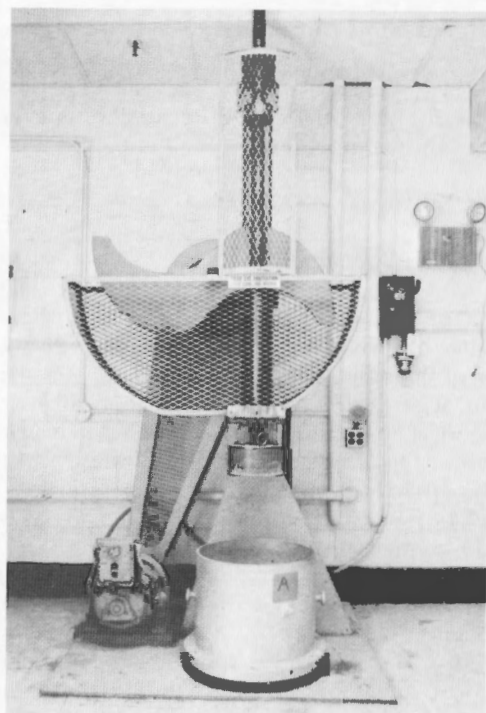
Figure 3. - Large mechanical compactor and compaction mold.
