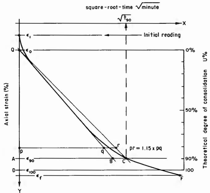
Figure X1.2.—Percent axial strain versus square root of time (square root of time method) — example.
