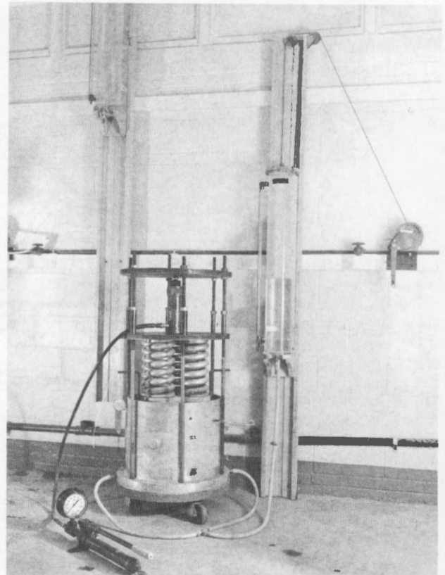
Figure 2.—19-inch permeability test being performed in the laboratory.
