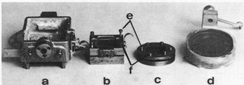
Figure 2. – Shear box bowls with associated shear boxes with gap and alignment screws installed, (a) shear box bowl, (b) shear box with removable bottom porous plate, (c) shear box, (d) shear box with bottom porous plate attached, (e) gap screws, and (f) alignment screws.
