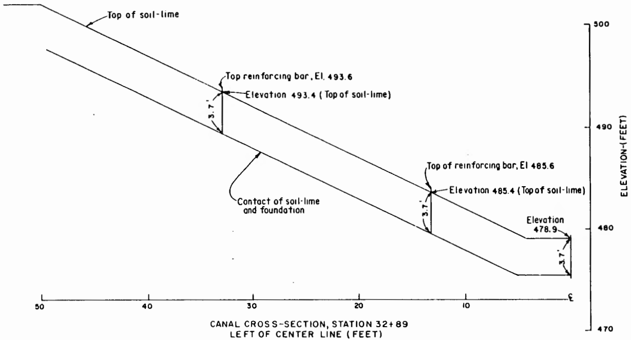
Figure 3A. - Typical soil-lime cross section (in-lb units).
