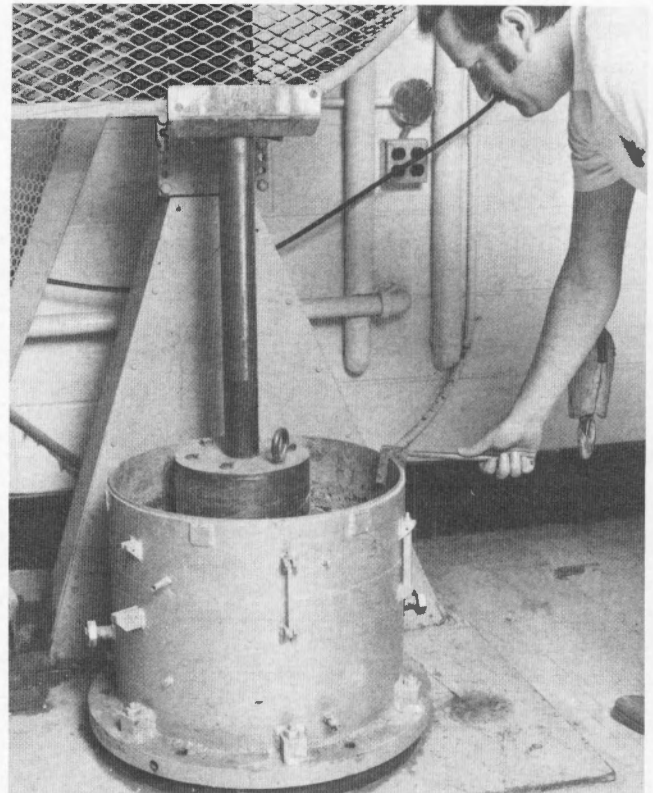
Figure 10. – Rotation of compaction mold using modified spanner wrench.
