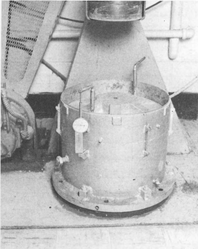
Figure 9. – Initial dial gauge measurement.
