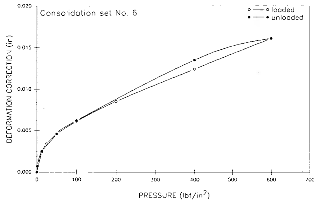
Figure 14. – Pressure versus equipment deformation correction — example.
