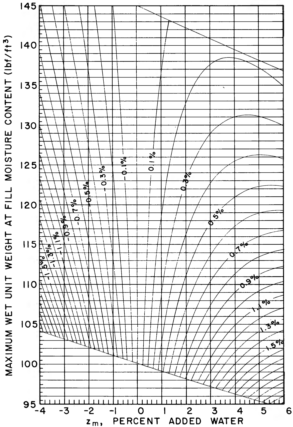
Figure 5. - Red-line correction — moisture adjustment values — w_o - w_f = z_m + \text{RLC} .
