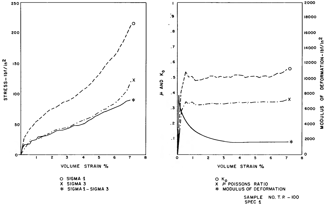
Figure 7. - K_0 - test data plots—example.
