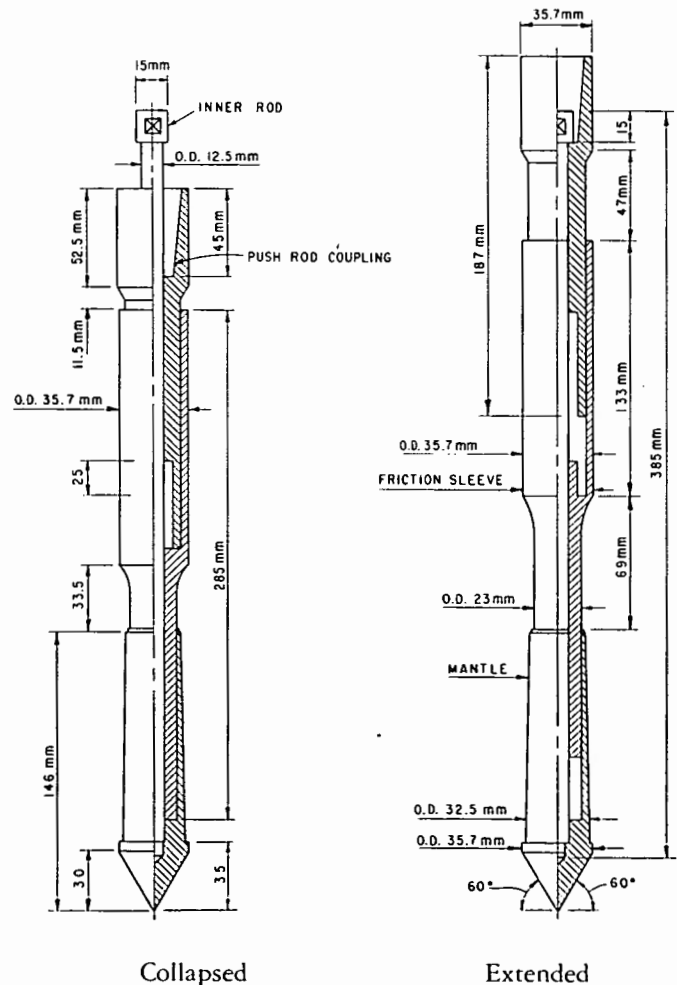
Figure 2. — Mechanical friction mantle cone penetrometer tip (Begemann friction cone).
