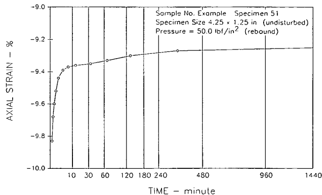
Figure 17. — Axial strain versus square root of time for specimen rebound upon unloading — example.
