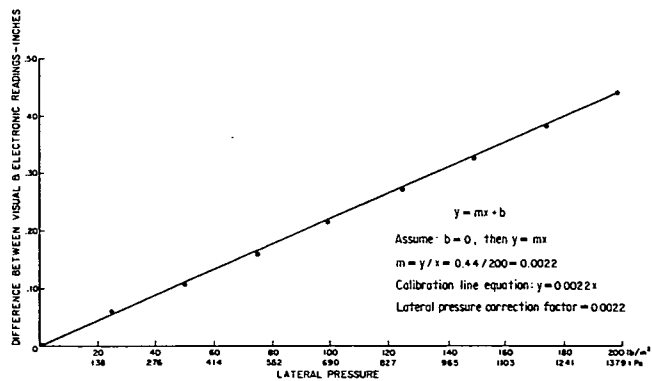
Figure 5. – Plot of lateral pressure correction factor — example.
