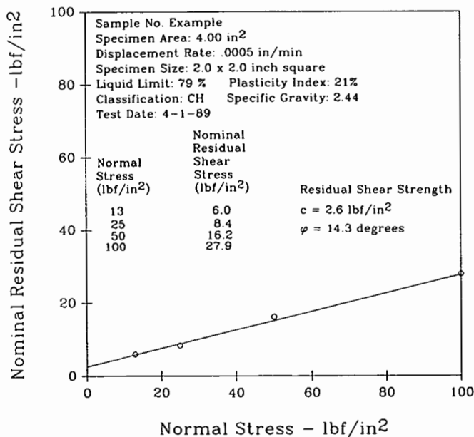
Figure 14. - Nominal residual shear stress versus normal stress plot—example.
