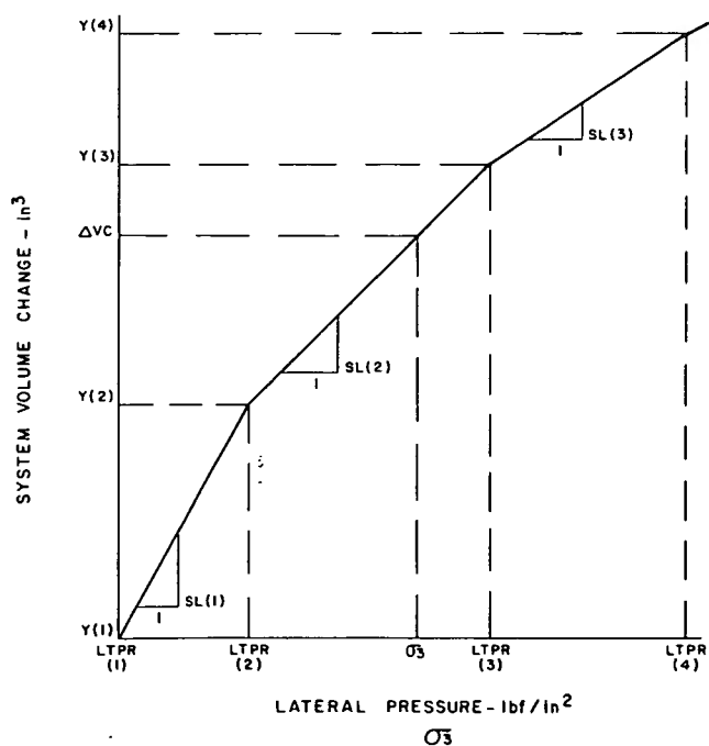
Figure 6. - Volume change of system due to applied lateral pressure.
