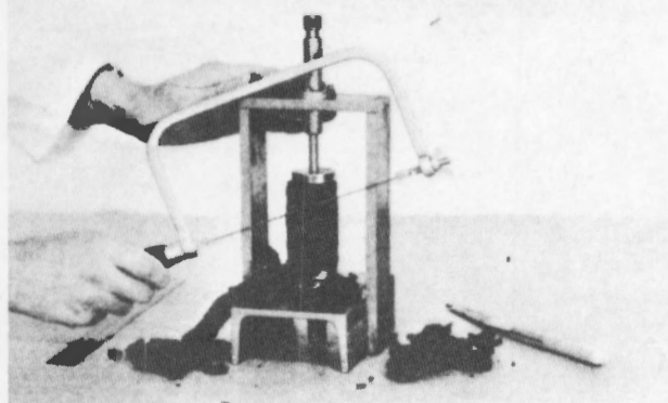
(c) Trimming to final diameter using wire saw against vertical guide plates.
