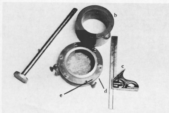
Figure 5. - 4.25-inch diameter specimen compaction equipment. (a) tamper, (b) compaction collar, (c) try square, (d) clamping ring, (e) specimen ring.
