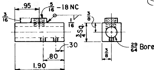
LVDT MOUNTING BLOCK CARRIER PART H TWO REQUIRED
