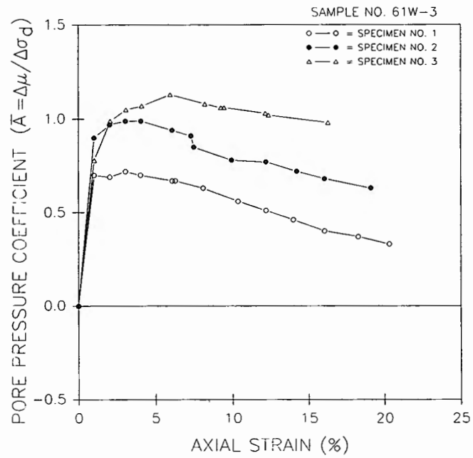
Figure 15. - Percent axial strain versus pore pressure coefficient—example.
