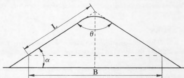
Figure 10. – Diagram for calculating the angle of repose.
