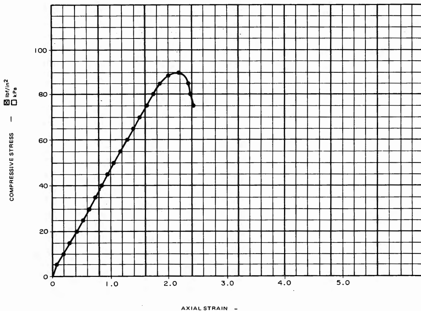
Figure 2. - Unconfined compressive strength plot — example.
