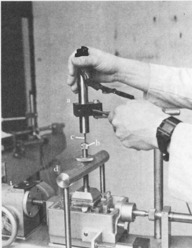
Figure 9. — Vertical displacement measurement device placement. (a) LVDT body, (b) yoke adjustment screw, (c) LVDT core and (d) loading yoke.
