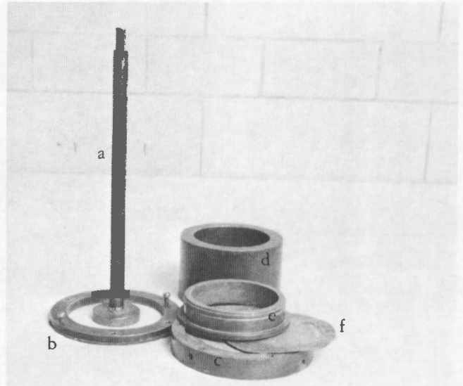
Figure 6.—One-dimensional consolidation, expansion, and uplift test specimen compaction equipment. a) tamper, b) collar and specimen ring retainer, c) compaction baseplate, d) compaction collar, e) specimen ring, and f) plastic liner.
