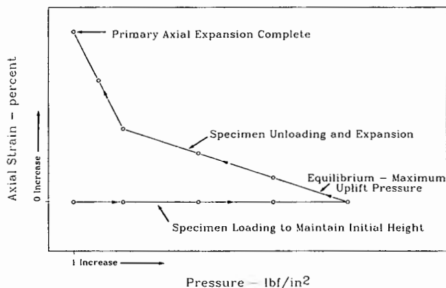
Figure 2. - Schematic of one-dimensional uplift test.
