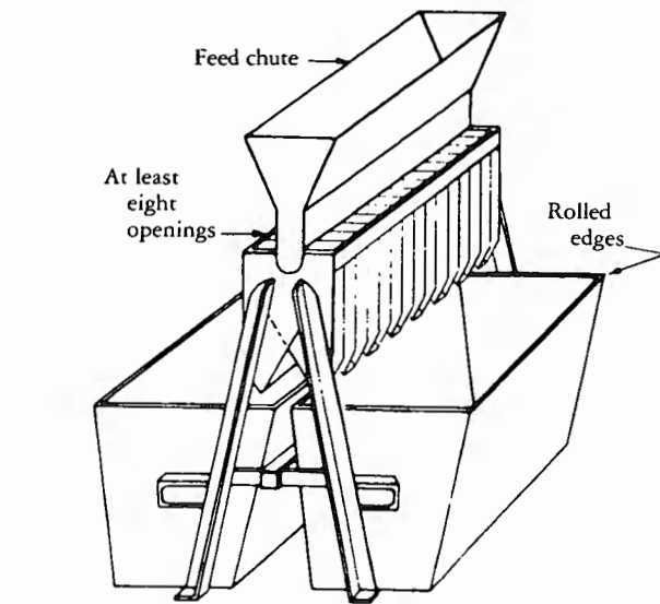
(a) Typical splitter for soils containing plus No. 4 sieve size particles.
