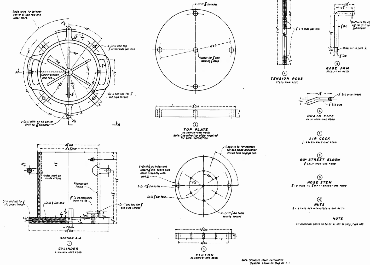
X1.2 - An 8-inch-inside-diameter aluminum permeability cylinder. 101-D-2
