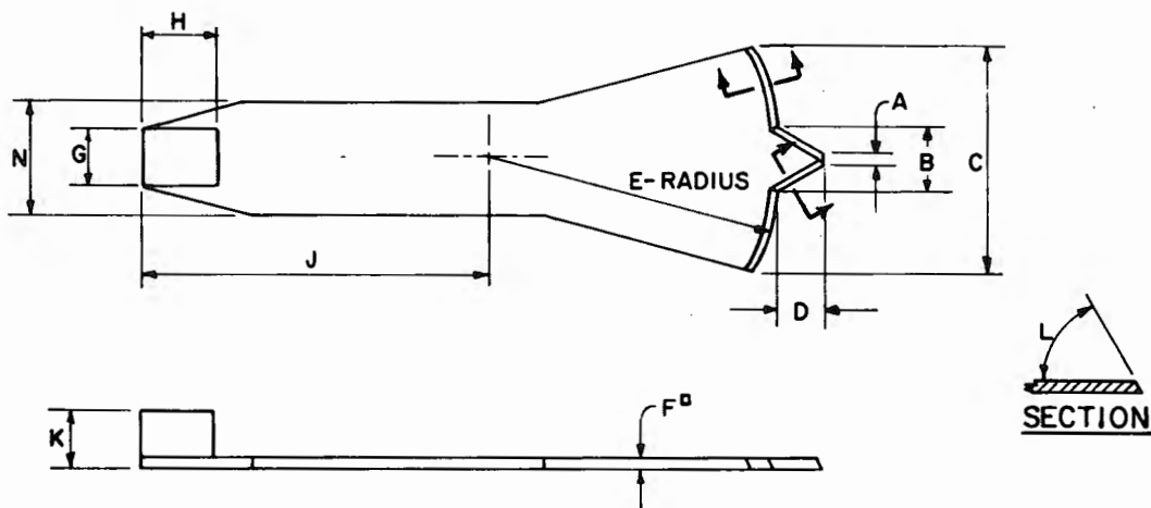
Figure 3. - Grooving tool (optional height-of-drop gauge attached) [ASTM D 4318].
