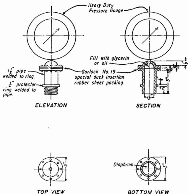
Figure 1. – Gauge saver device for protecting pressure gauge. 40-D-4287
