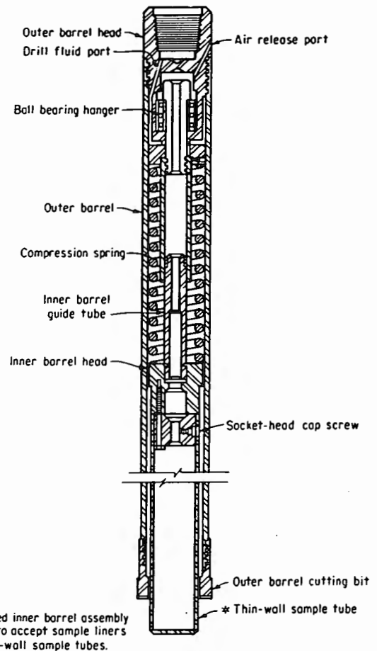
Figure 12. — Pitcher sampler (double-tube core barrel).
