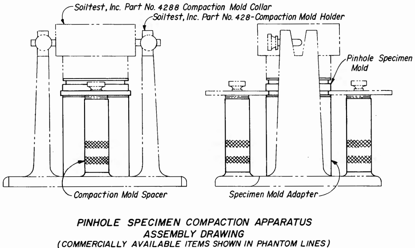
Figure 1. - USBR Pinhole test apparatus — Continued.
