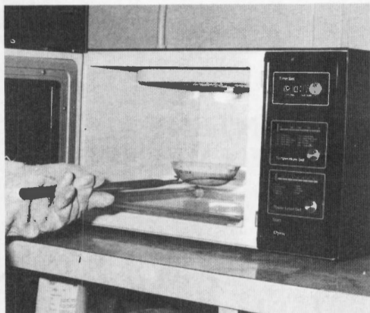
Figure 1. - Determining moisture content using microwave oven.
