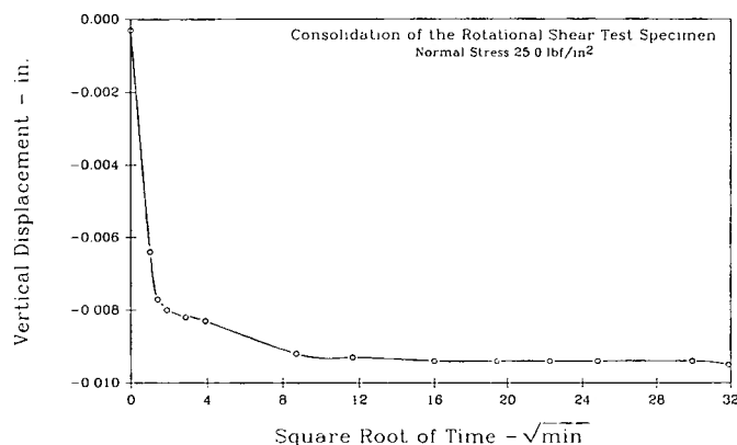
Figure 20. - Vertical displacement versus square root of time plot (normal stress = 25 lbf/in 2 ) — example.
