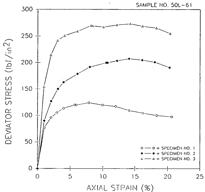
Figure 11. — Percent axial strain versus deviator stress—example.
