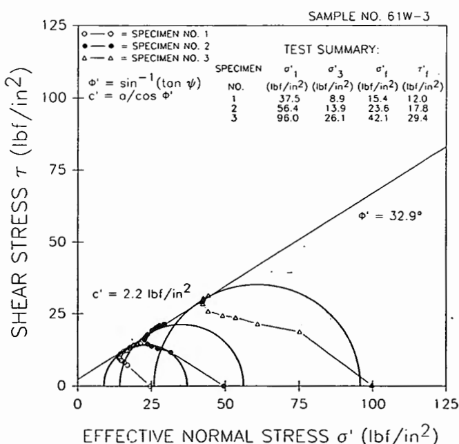
Figure 10. - Mohr's diagram—example.
