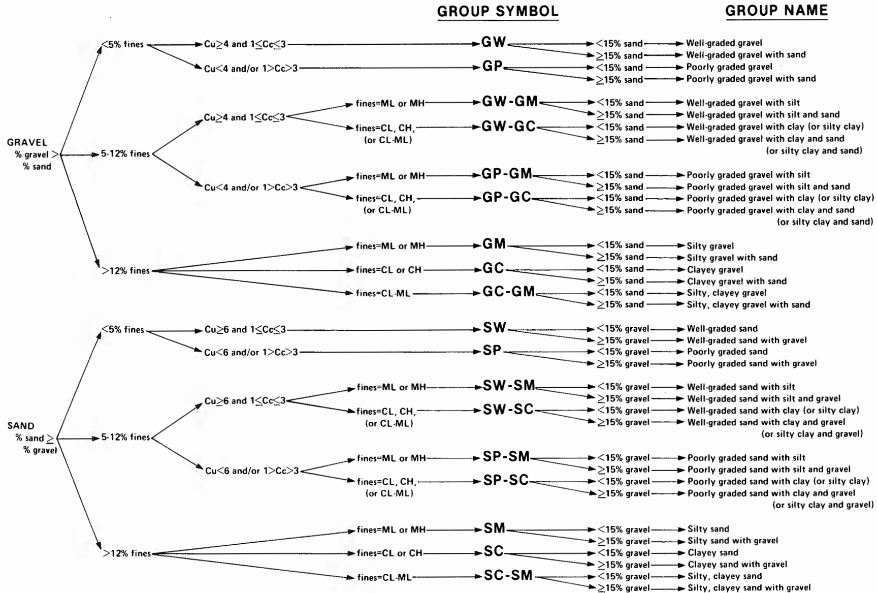
Figure 2. – Flow chart for classifying coarse-grained soils – laboratory method (more than 50% retained on No. 200 sieve).
