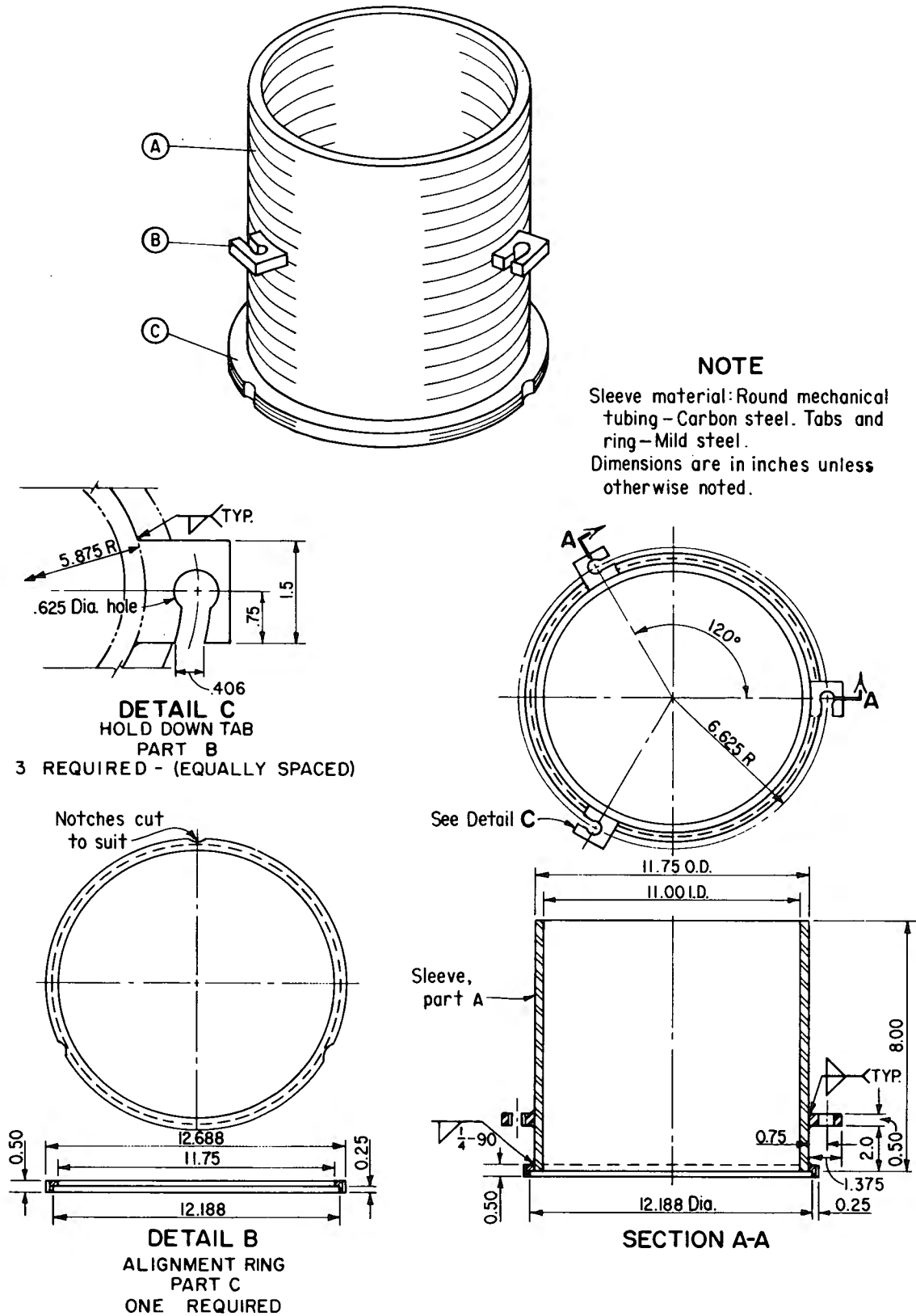
Figure 4. - Surcharge guide sleeve for 0.5 ft 3 (14 158 cm 3 ) measure.
