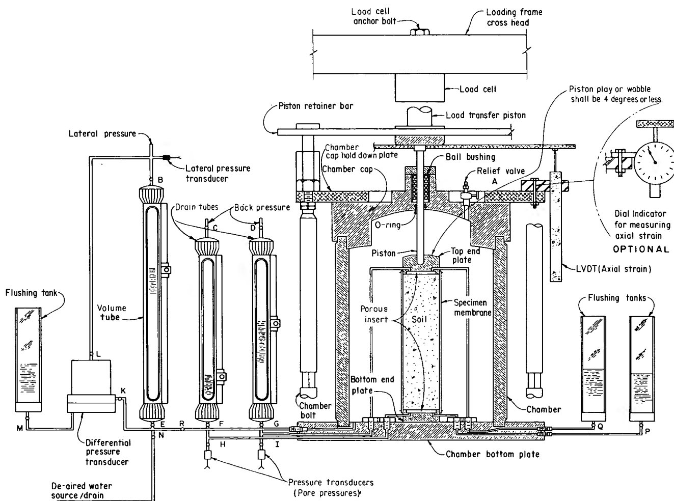
Figure 1. – Triaxial assembly for consolidated-undrained tests.
