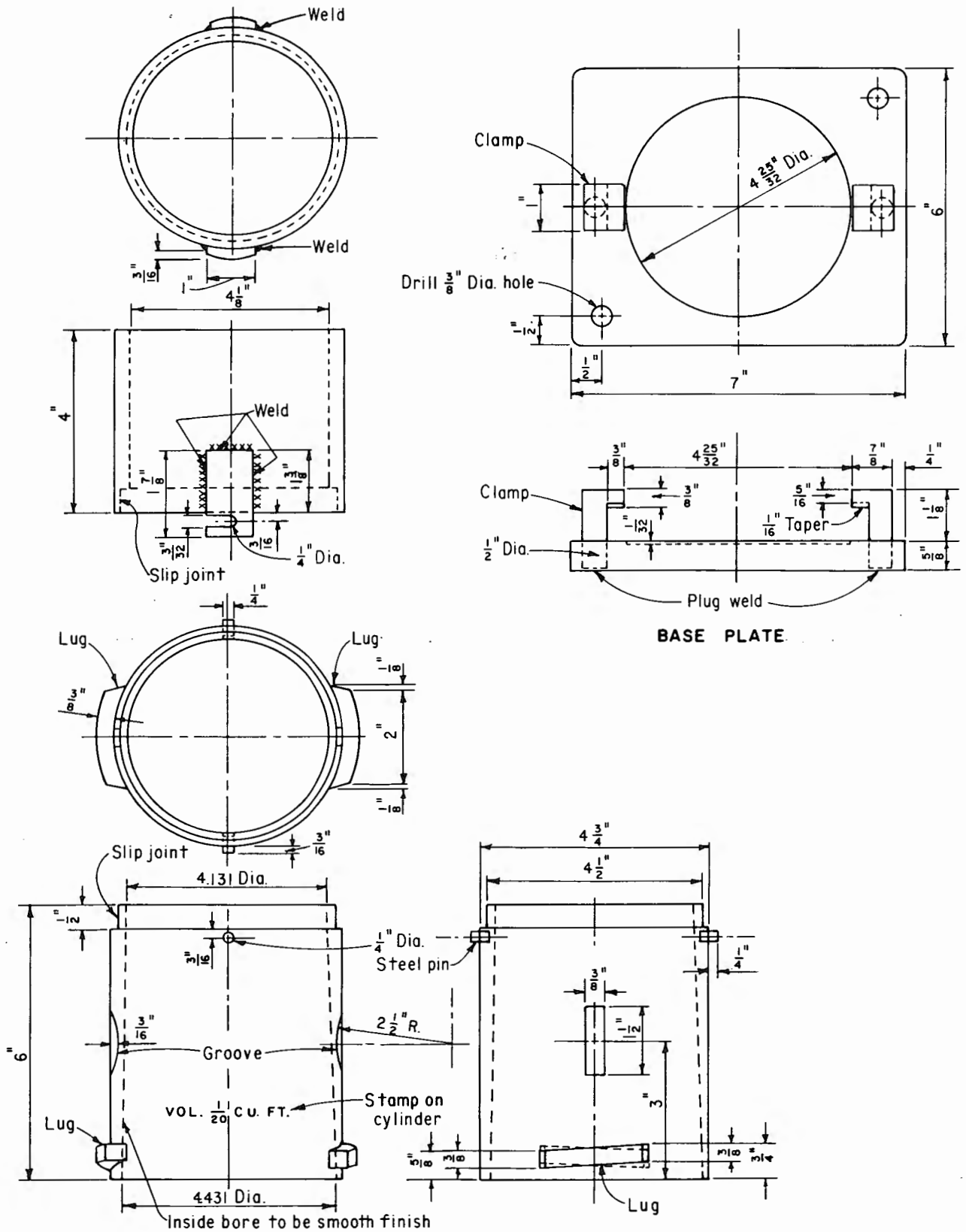
Figure 3. - Compaction mold
