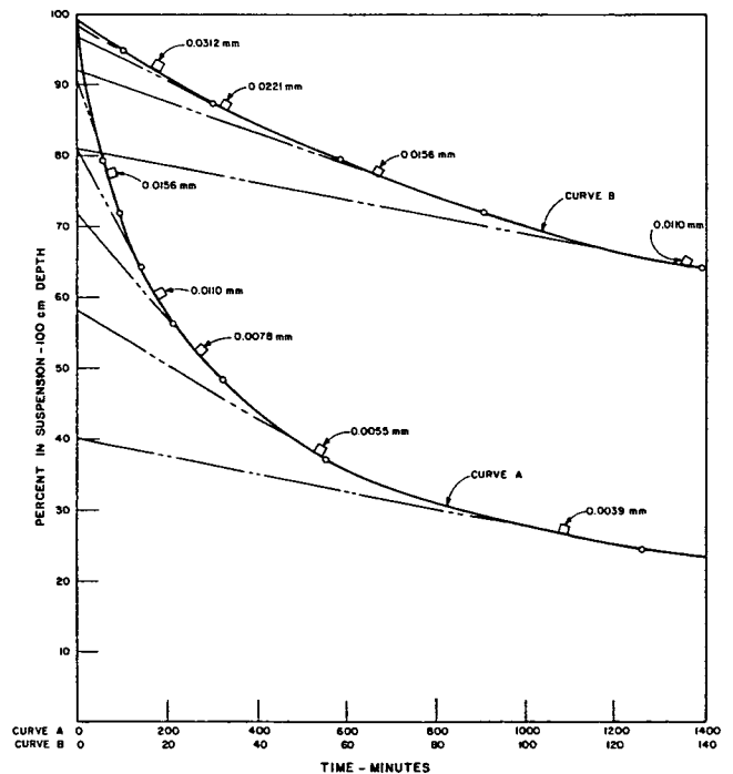
Figure X3.3 - Odén curve construction — Continued.
