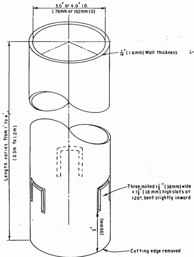
Figure 1. — Core retrieval barrels made from worn diamond studded core barrels.
