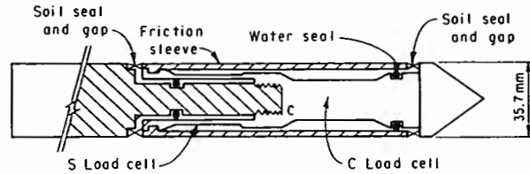
(a) Independent tension-type electric friction — cone penetrometer.
