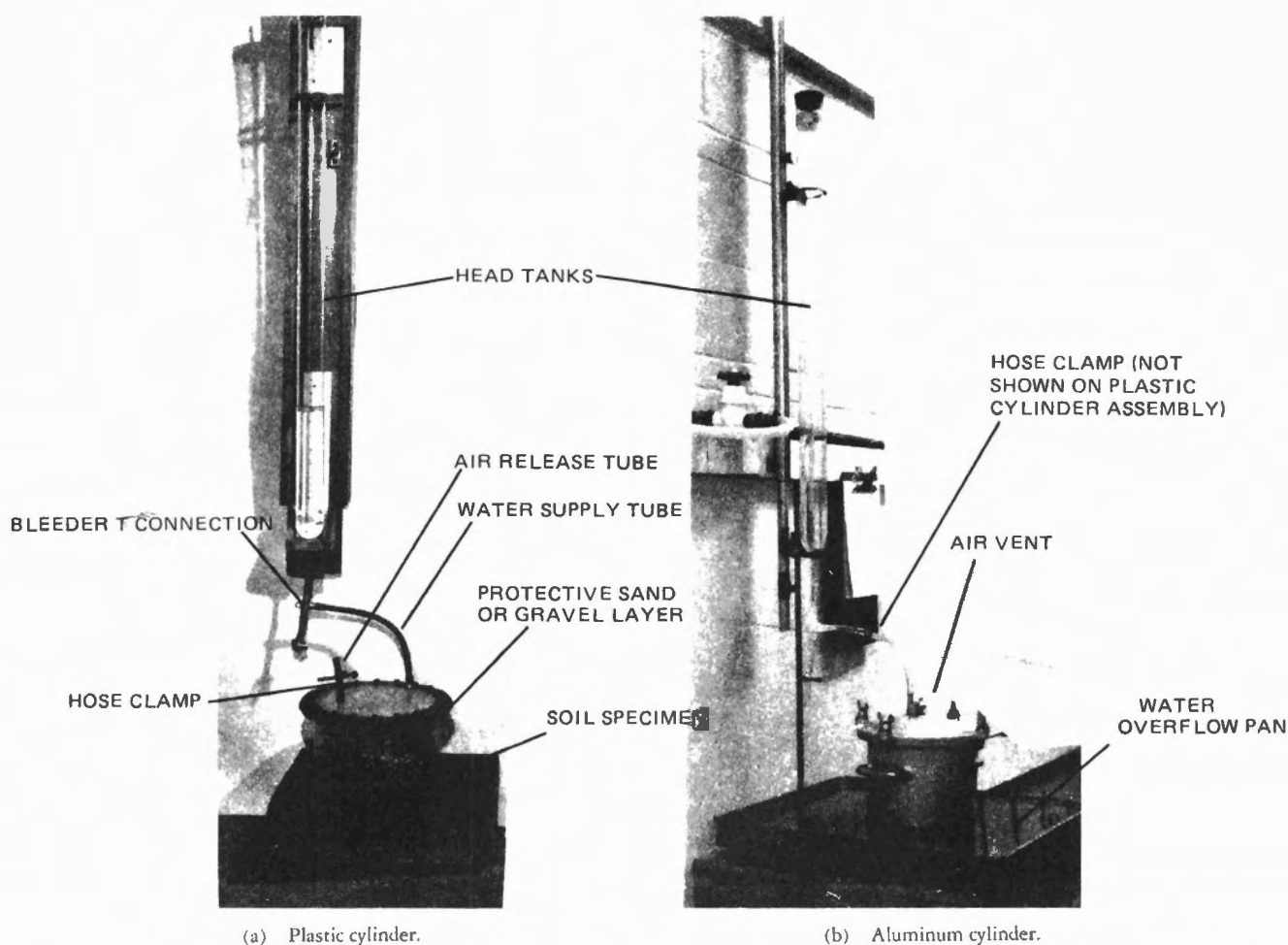
Figure 3. – Permeability cylinders with zero normal pressure.
