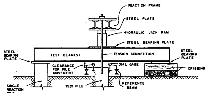
Figure 1. — Test setup using crossbeams [ASTM D 3689].
