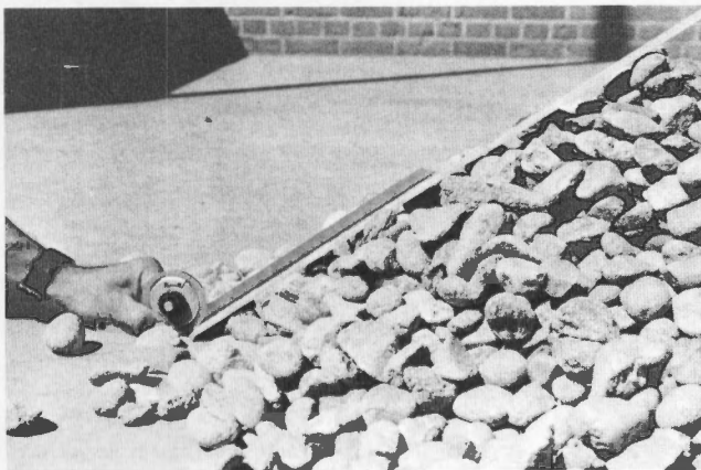
Figure 6. – Measuring the angle of repose of coarse gravel using a mechanic's vernier protractor and yardstick on the pile face.
