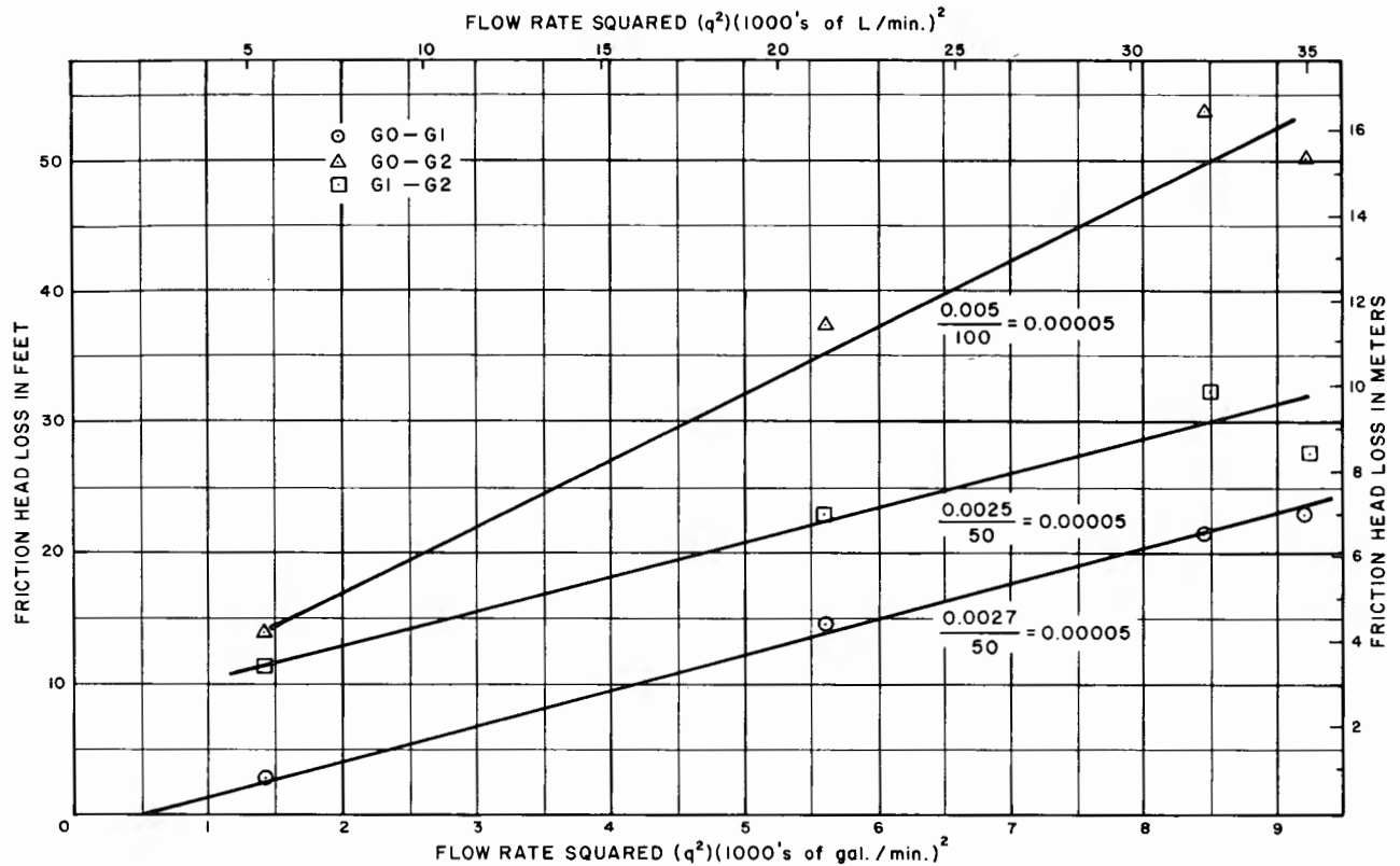
Figure 4. – Plot of feed pipe calibration data — example.
