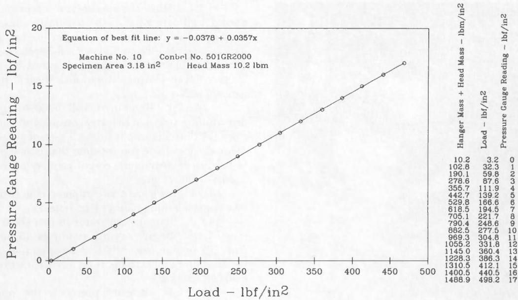
Figure 13. - Calibration of pneumatic loading device — example.
