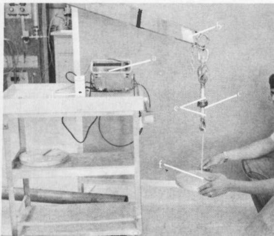
Figure 3. – Force transducer hanger assembly for tension calibration using mass standards. a) digital voltmeter, b) hoist, c) load cell, d) signal conditioner, e) load cell couplers, and f) hanger assembly.
