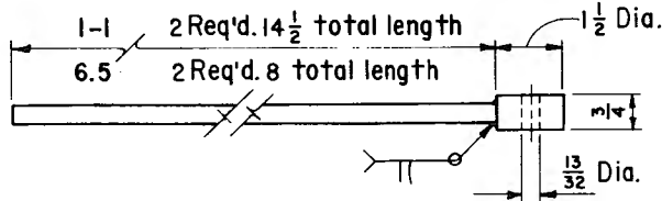
EXTENSION ARMS PART F TWO OF EACH REQUIRED
