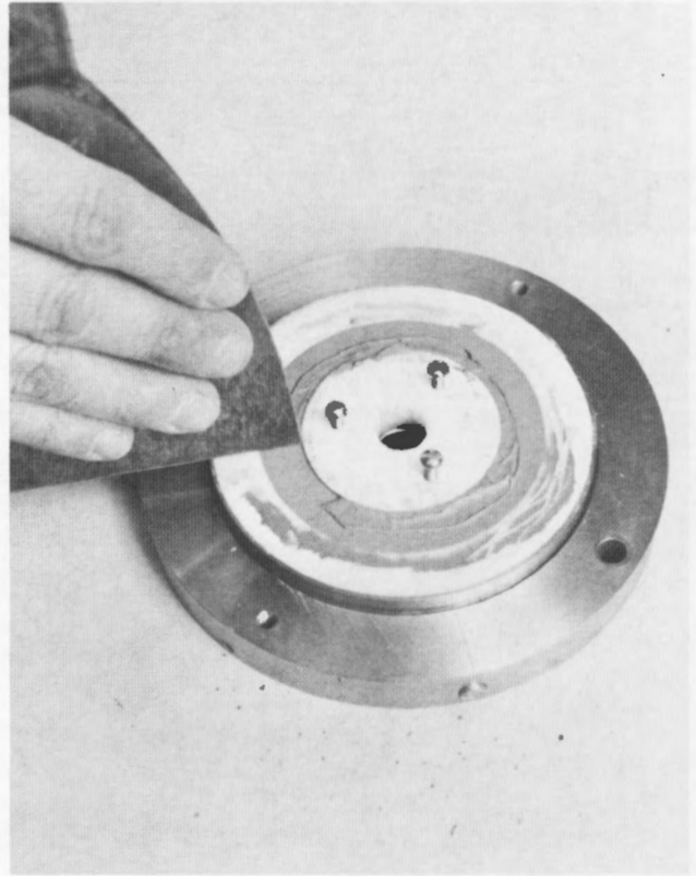
Figure 11. – A stiff straightedge (putty knife) may be used to level the surface of the specimen.
