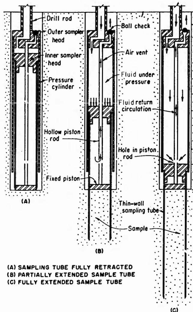
Figure 9. - Thin-wall fixed-piston sampler (Osterberg type).
