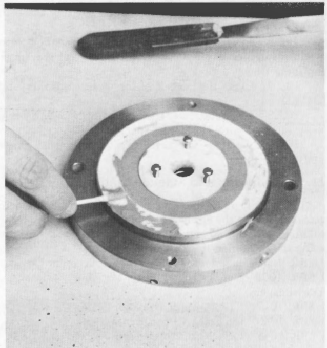
Figure 12. – The surface of the outer confining ring being cleaned with a moistened cotton swab.
