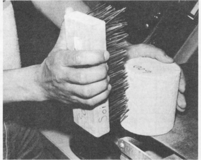
(b) Closeup view of downward vertical brushing strokes applied to the sides of a soil-cement durability test specimen.
