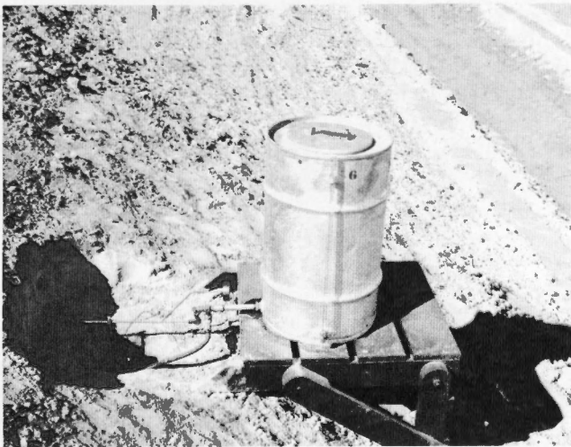
Figure 3. — Shallow-well permeameter installed in the compacted earth lining of a canal side slope.
