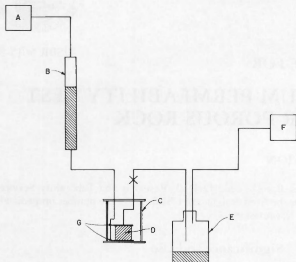
Figure 1. - Schematic of radial vacuum permeability test. A) pressure source and gauge, B) graduated volume tube, C) specimen container, D) specimen, E) graduated effluent container, F) vacuum source and gauge, G) specimen end plates, and X) valve.
