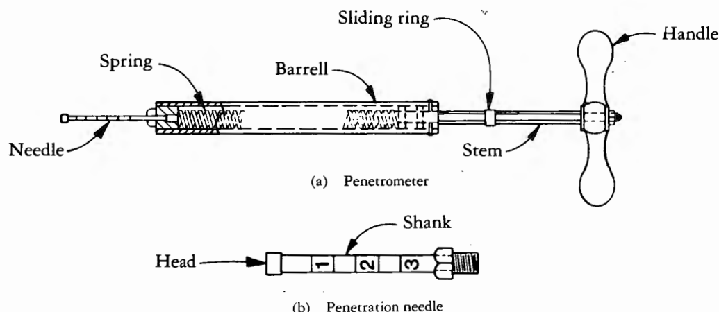
Figure 1. — Soil penetrometer.
