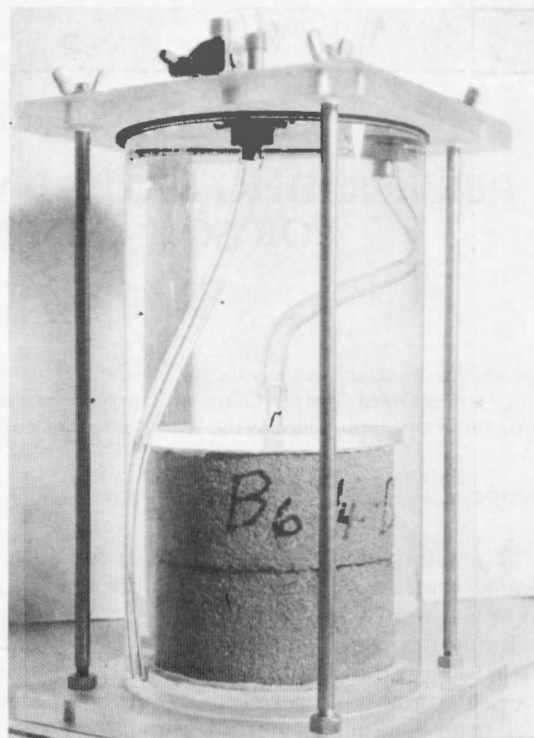
Figure 2. - Soil-cement test specimen placed in specimen container.
