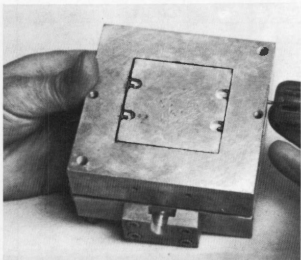
Figure 6. - Pushing in retaining pins over a correctly positioned lower plate.
