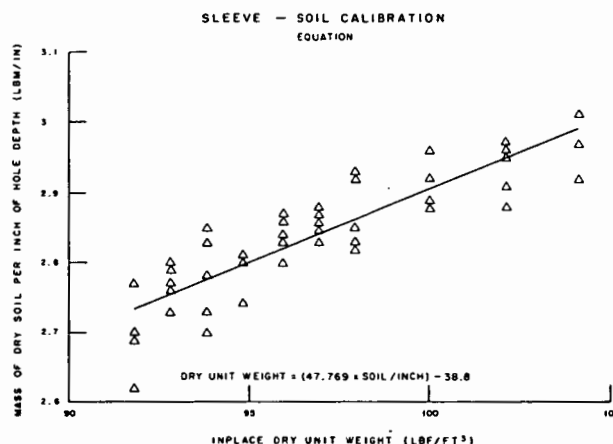
Figure X1.1 – Calibration equation for unit weight of soil in-place by the sleeve method — example.
