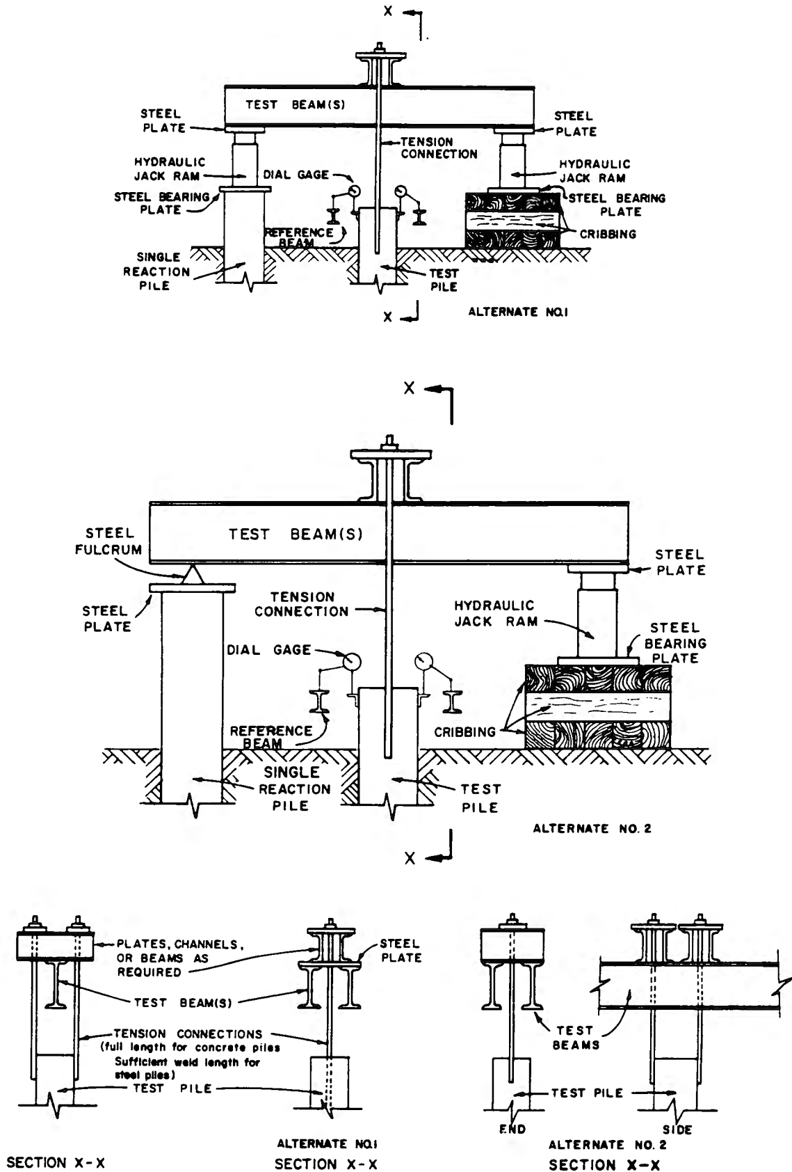
Figure 2. - Alternate methods of using crossbeams to provide reaction force [ASTM D 3689].
