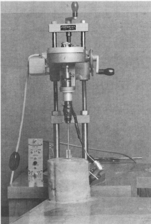
Figure 7. - Test specimen in place under vane shear device.
