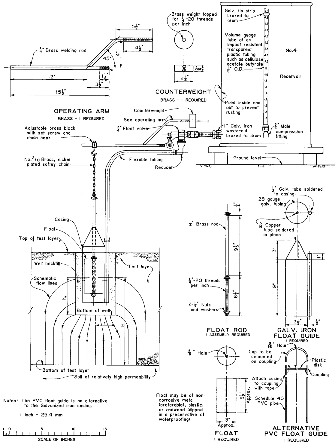
Figure 1. - Shallow-well permeameter test equipment. 101-D-352
