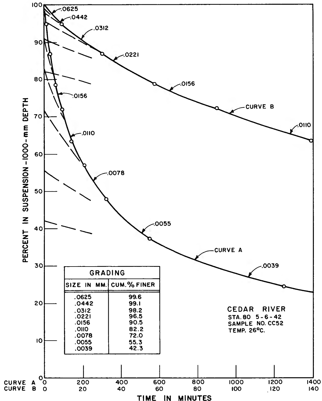
Figure 3. - Completed Odén curve.
