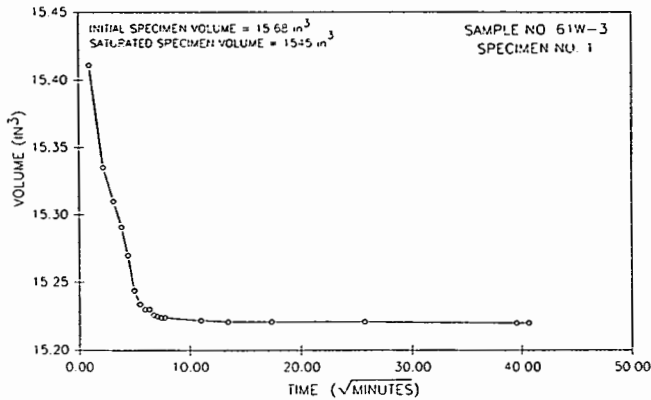
Figure 7. – Specimen volume versus square root of time—example.
