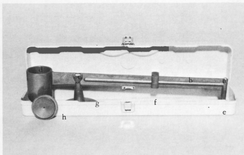
Figure 1. — Mud balance. (a) retainer screw, (b) beam (with etched scale), (c) level bubble, (d) cup, (e) counter weight, (f) rider weight, (g) support, and (h) cap.
