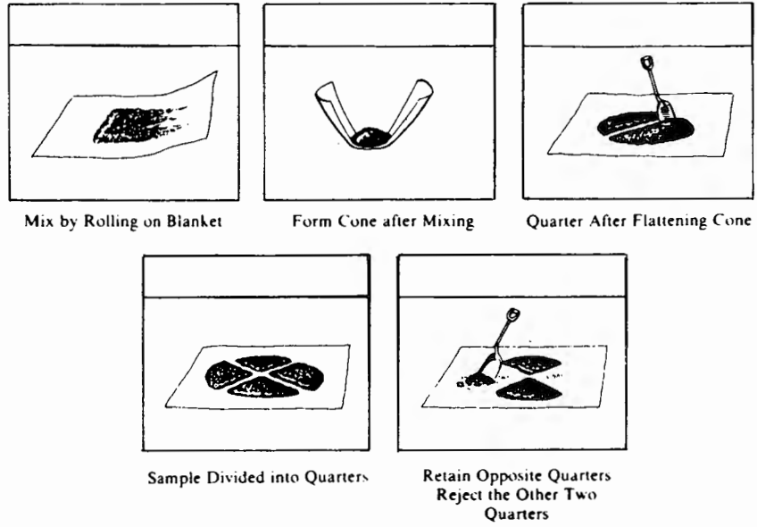
Figure 3. - Quartering using a quartering cloth [ASTM C 702].
