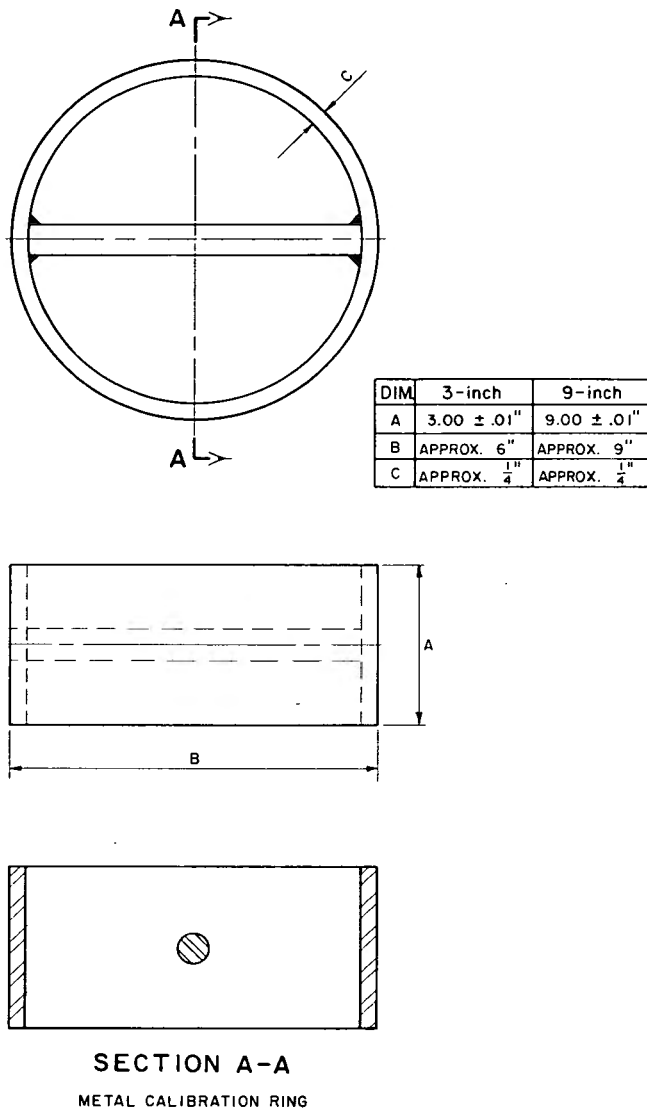
Figure 1. – Metal calibration ring.
