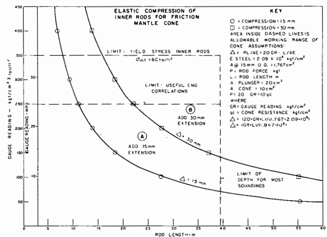
Figure X1.1. - Elastic compression of inner rods for friction mantle cone.
