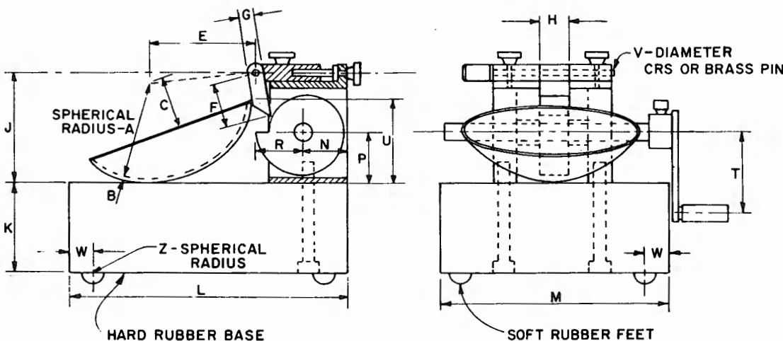
Figure 2. - Hand-operated liquid limit device [ASTM D 4318].
