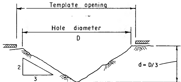
Figure X1.1. - Test pit configurations.
