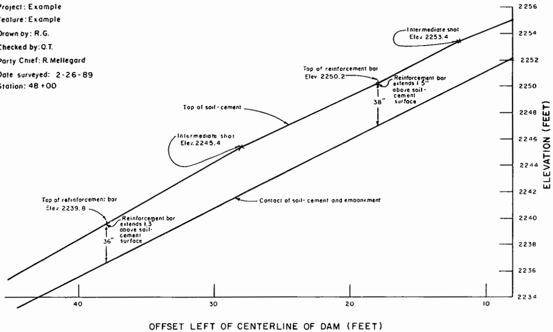
Figure 4A. - Soil-cement cross section (in-lb example).
