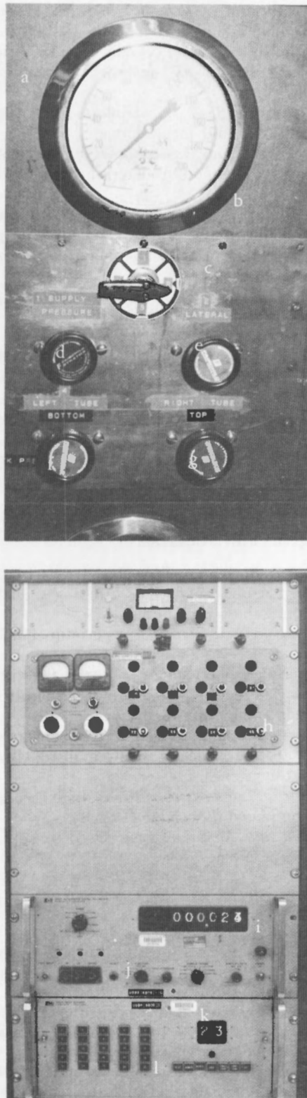
Figure 3. – Pressure control box and data acquisition system for back pressure permeability testing. a) pressure control box, b) pressure gauge, c) pressure function selector, d) supply regulator, e) lateral regulator, f) bottom regulator, g) top regulator, h) balance controls, i) voltmeter readout, j) function selector, k) period selector, and l) channel selector.
