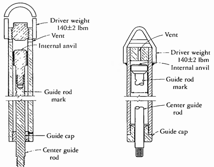
Figure 2. — Internal anvil safety hammers — typical designs.
