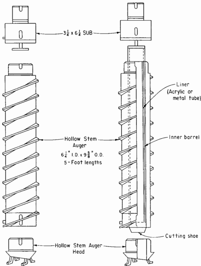
Figure 13. - Continuous hollow stem auger (not to scale).
