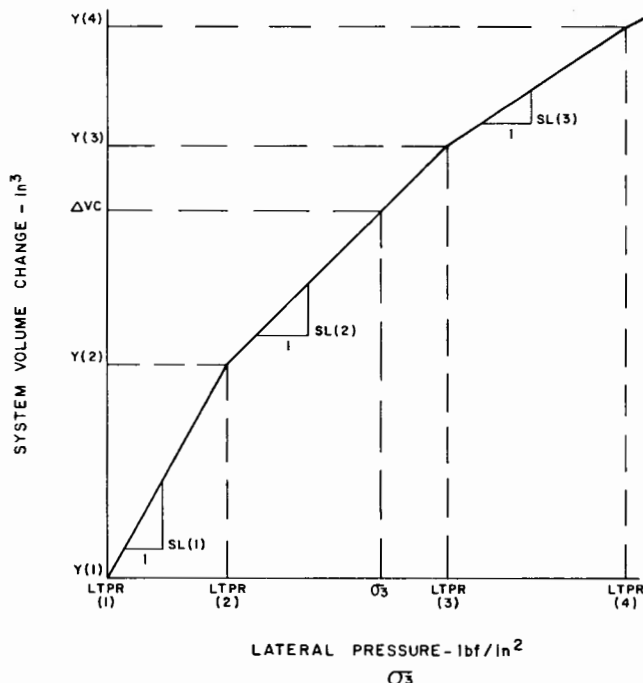
Figure 8. – Volume change of system due to applied lateral pressure.
