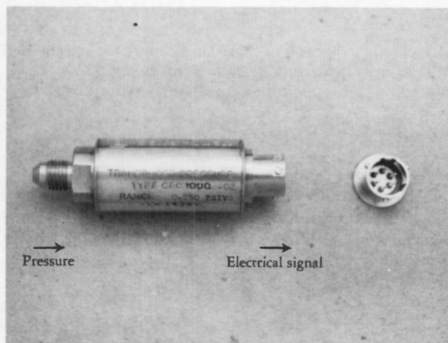
Figure 1. – Pressure transducer.
