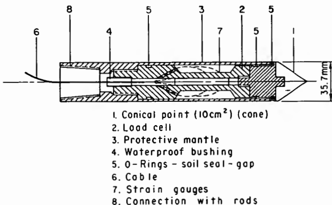
Figure 1. — Typical electric cone penetrometer tip (Robertson and Campanella, 1984 [2]).
