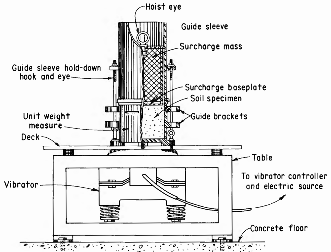
Figure 6. - Schematic of maximum index unit weight test equipment (sheet 1 of 4).
