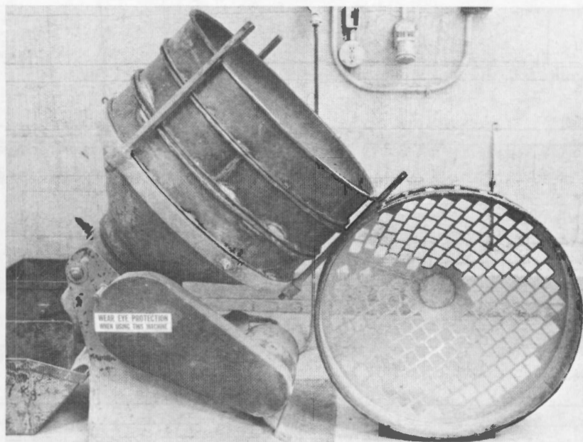
Figure 2. – Separating device.
