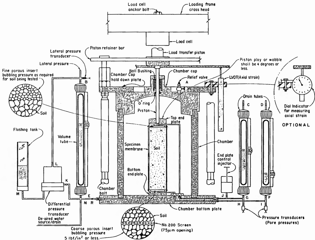
Figure 1. - Triaxial assembly for undrained tests.
