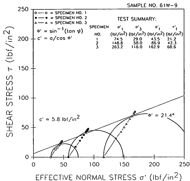
Figure 10. – Mohr's diagram — example.
