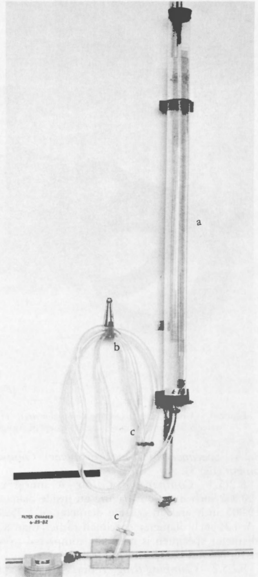
Figure 6. – Head tank apparatus for permeability testing. (a) glass head tank, (b) 1/8-inch plastic tubing, (c) hose clamps.
