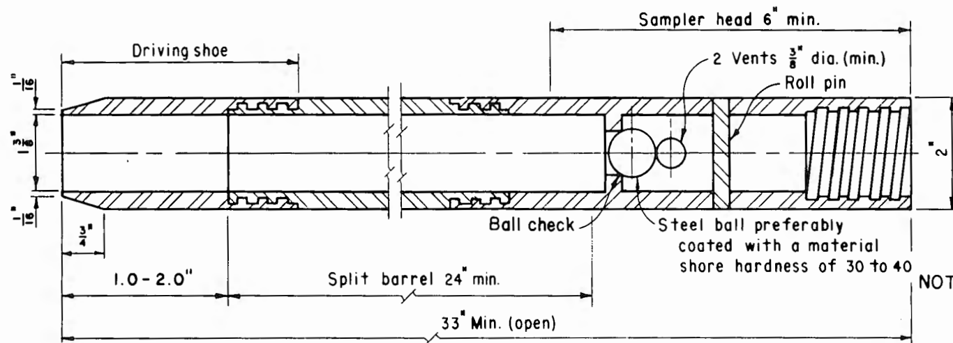
SPLIT BARREL PENETRATION RESISTANCE SAMPLER
