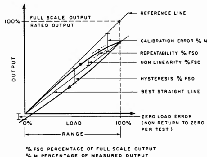
Figure A1.1. - Definition of terms related to calibration (Schaap and Zuidberg, [1] 1982).
