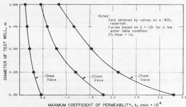
Figure 3. — Maximum permeability coefficients measurable with typical float valves commonly used on stock-watering tanks.
