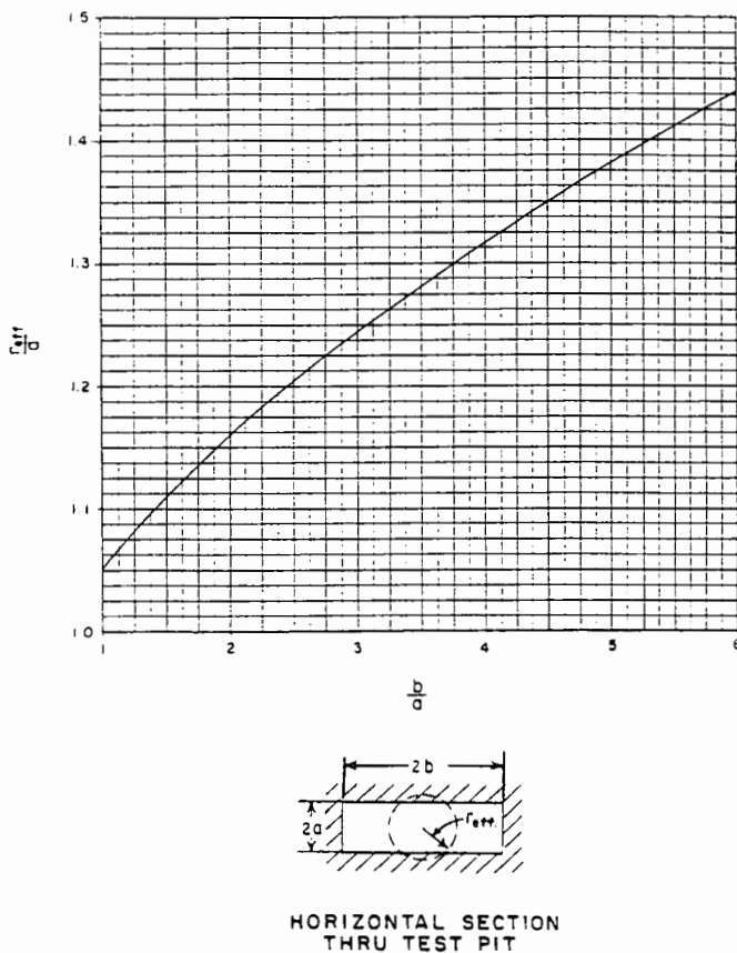
Figure 5. - Effective cylindrical radius of rectangular test pits. (fig. 44 of ref. 2)
