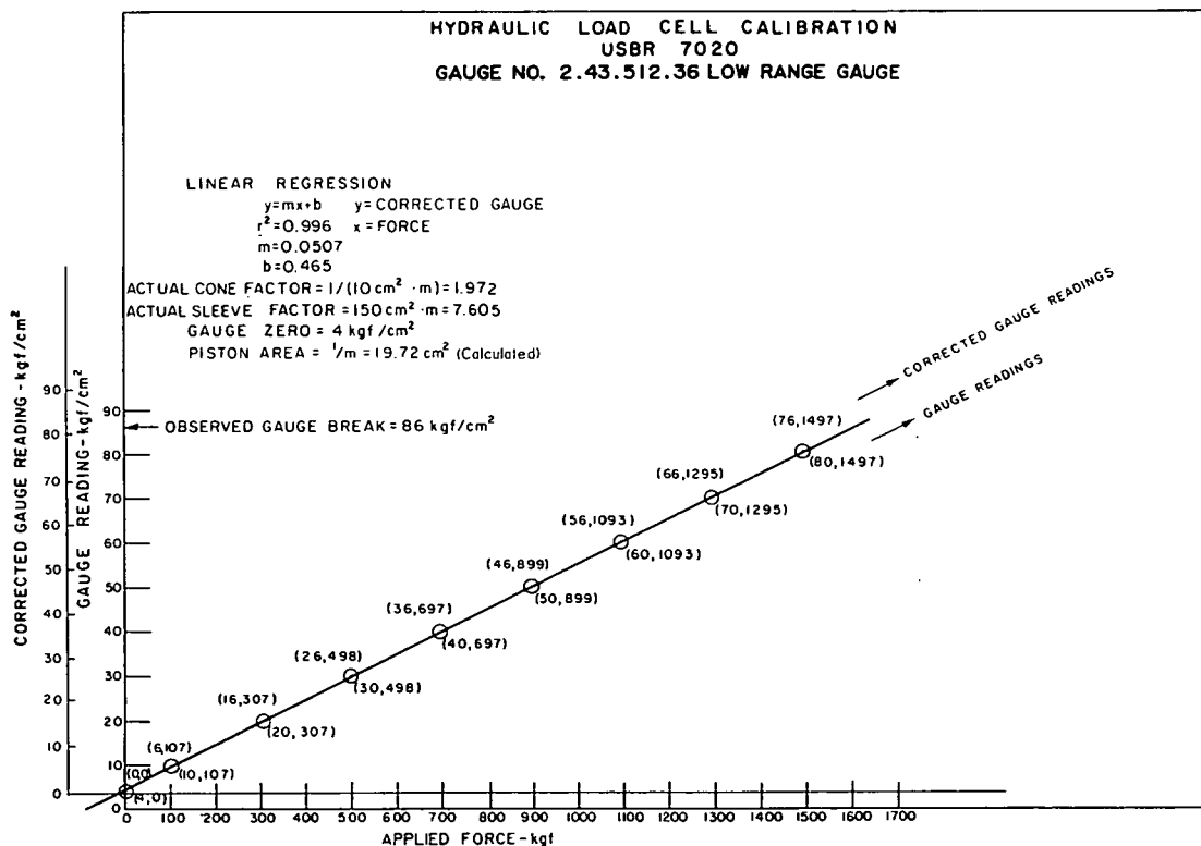
Figure A1.1. - Hydraulic load cell calibration — low range gauge example.
