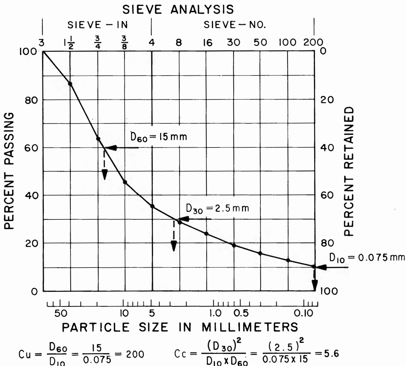
Figure 4. — Gradation plot.
