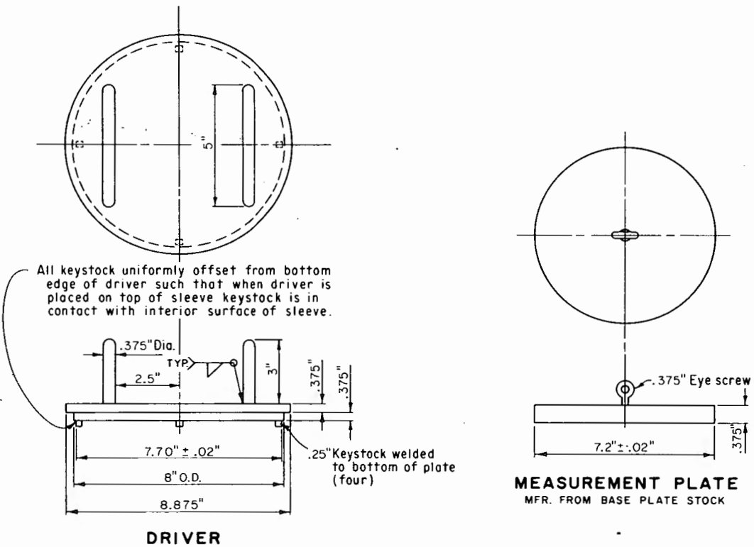
Figure 1. - In-place soil density equipment — sleeve apparatus.
