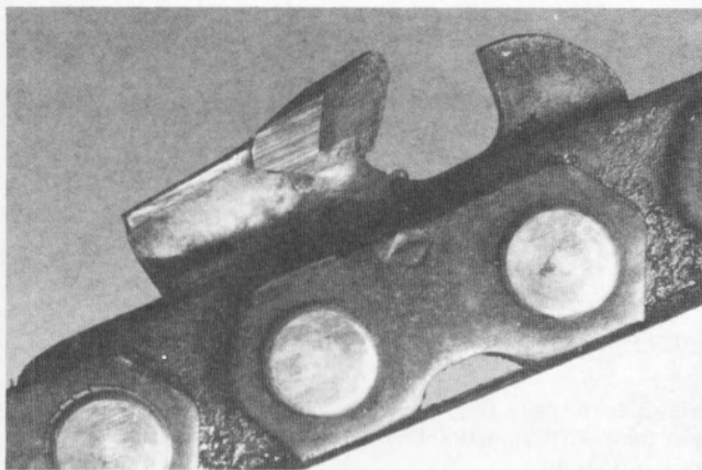
Figure 1. – Carbide-tipped cutting tooth on chain.
