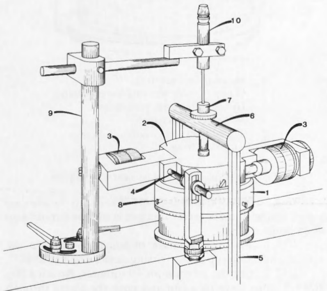
Figure 4. - Top plate placement onto the shearing unit turntable.
