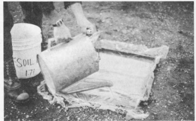
Figure 7. – Sand being poured into the template.
