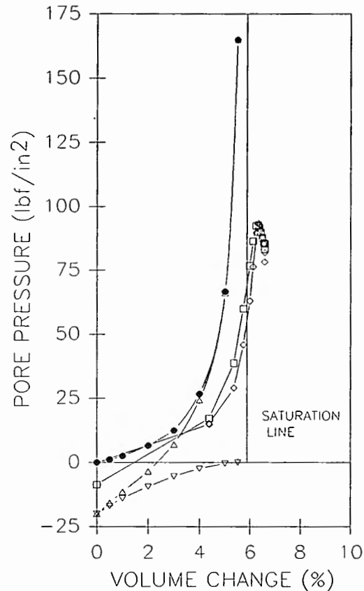
Figure 7. — Pore air and pore water pressure versus percent volume change—example.
