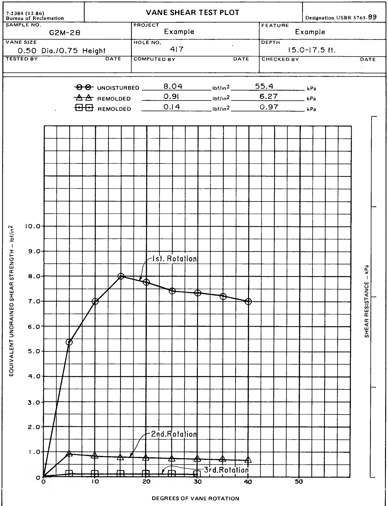
Figure 9. - Vane shear test plot — example.
