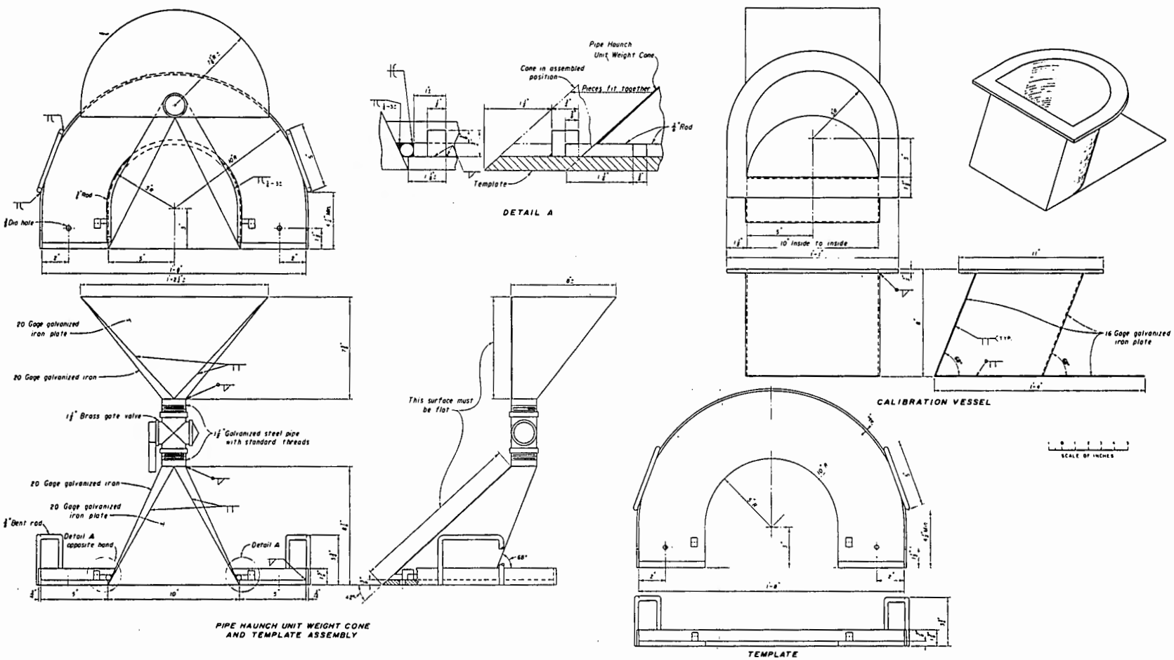
Figure 3. - Pipe haunch unit-weight cone — template, calibration vessel. 801-D-223
