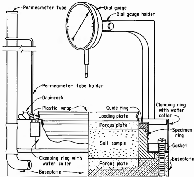
Figure 1. - Schematic of fixed-ring consolidometer.
