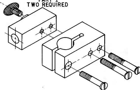
Figure X2.2. - Vibratory table calibration equipment — Continued. 101-D-649
