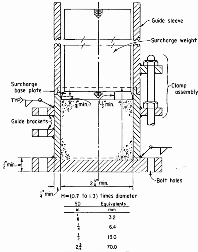
Figure 2. – Special cylindrical unit weight measure. [ASTM D 4253]
