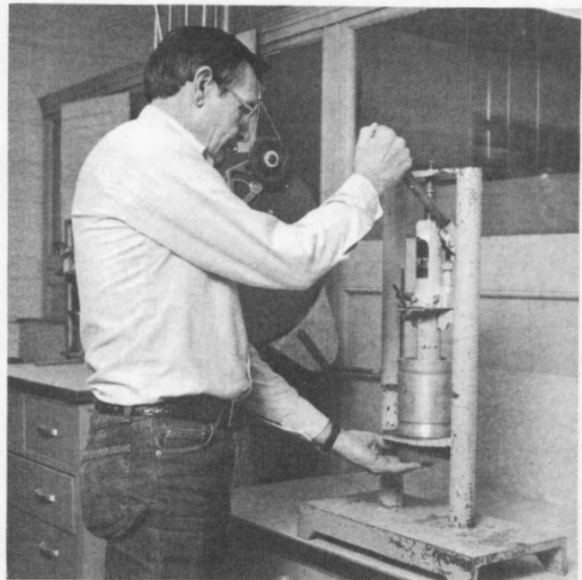
Figure 2. – Extruder for compaction specimens.
