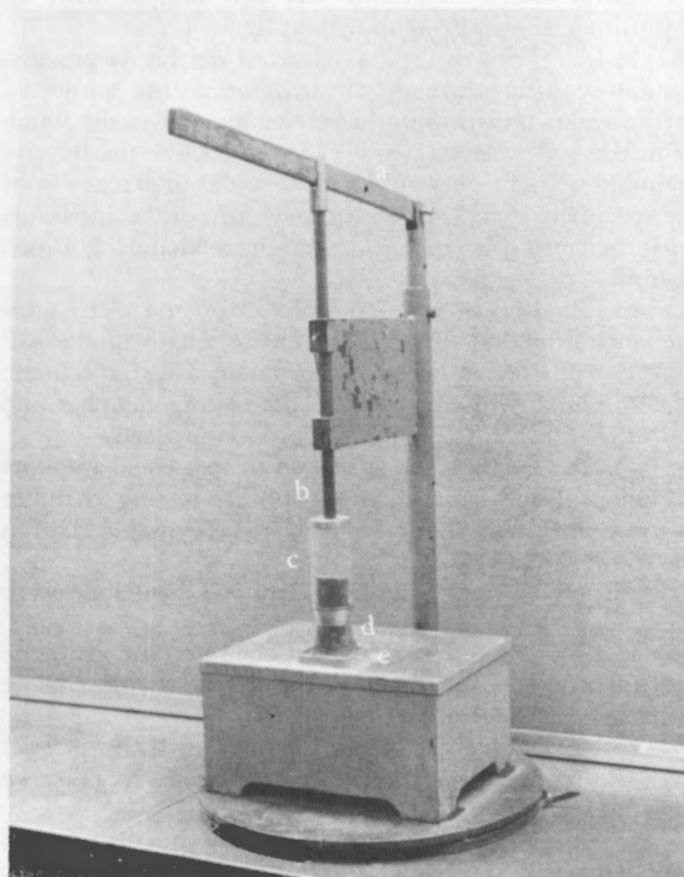
Figure 2. — Cutting an undisturbed soil specimen to be placed in a membrane. (a) lever arm, (b) guide rod, (c) spacer chamber, (d) cutting bit, and (e) wax.
