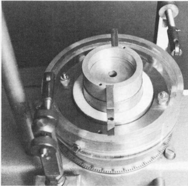
Figure 16. – Moment transfer plate parallel to horizontal restraining arms.
