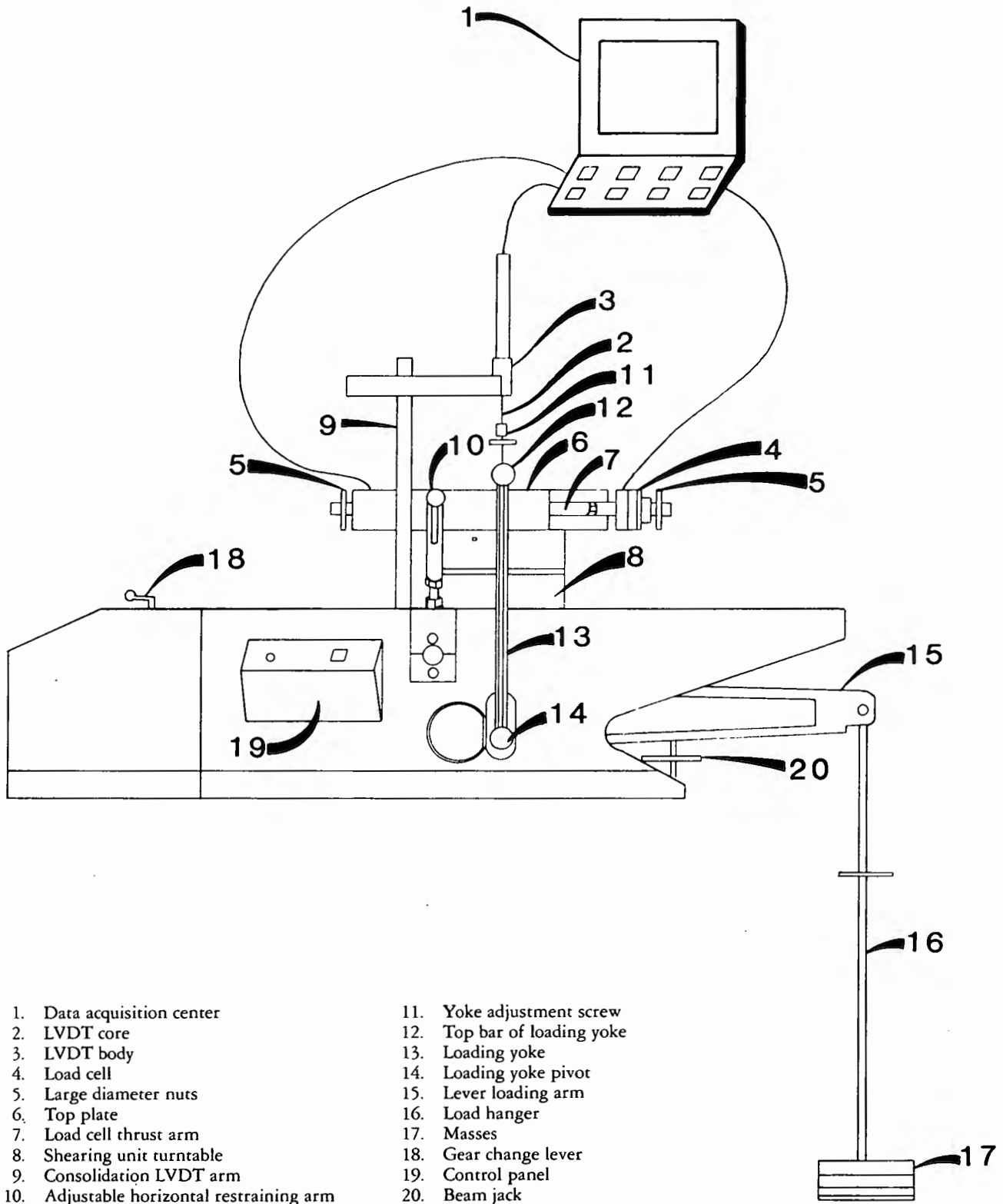
Figure 1. – Rotational shearing unit.
