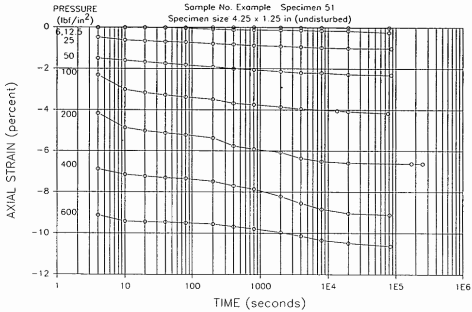
Figure 20. - Axial strain versus log-time summary — example.
