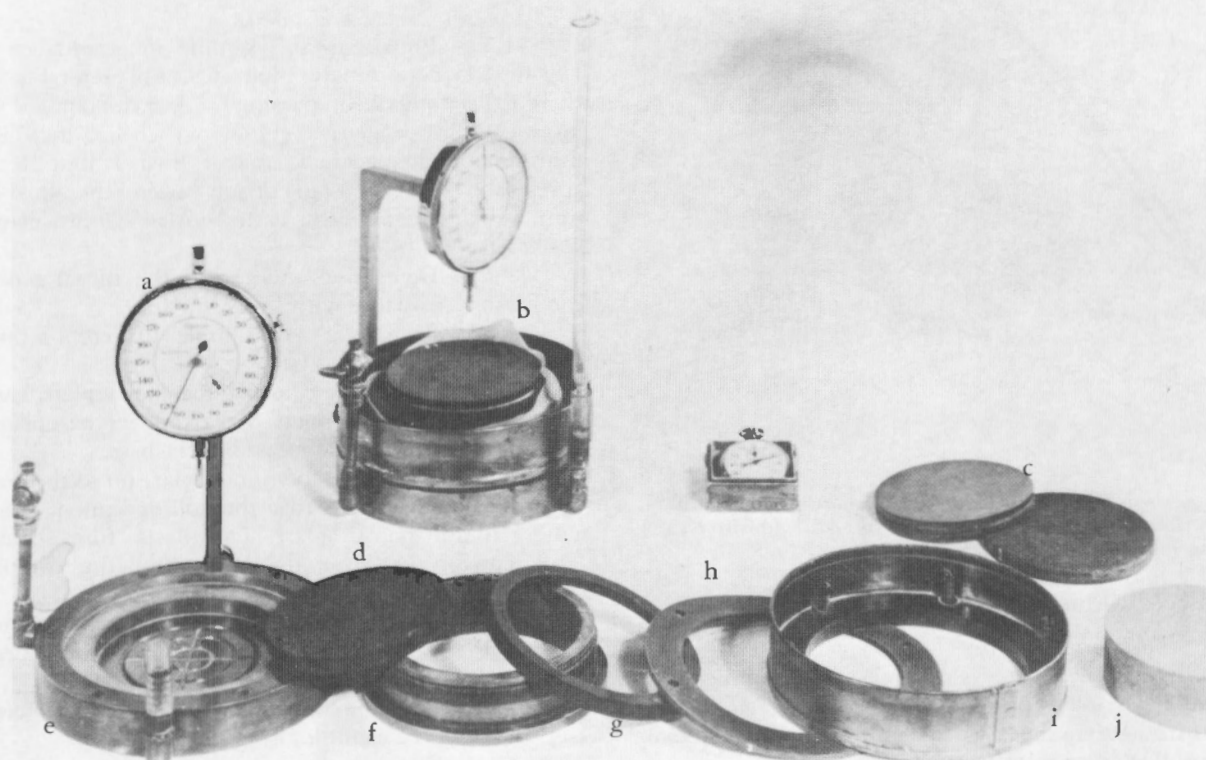
Figure 4. - Fixed-ring consolidometer. (a) dial gauge, (b) assembled consolidometer, (c) porous plates, (d) top load plate, (e) base plate, (f) specimen ring, (g) guide ring, (h) rubber gasket, (i) water collar with clamping ring, and (j) gauge block.
