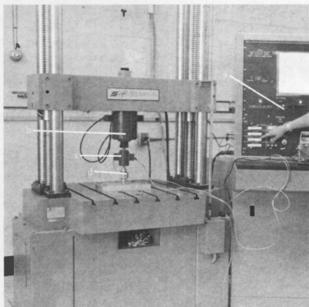
Figure 4. – Universal testing machine. a) control panel, b) universal testing machine force transducer, c) force transducer being calibrated, and d) coupler.
