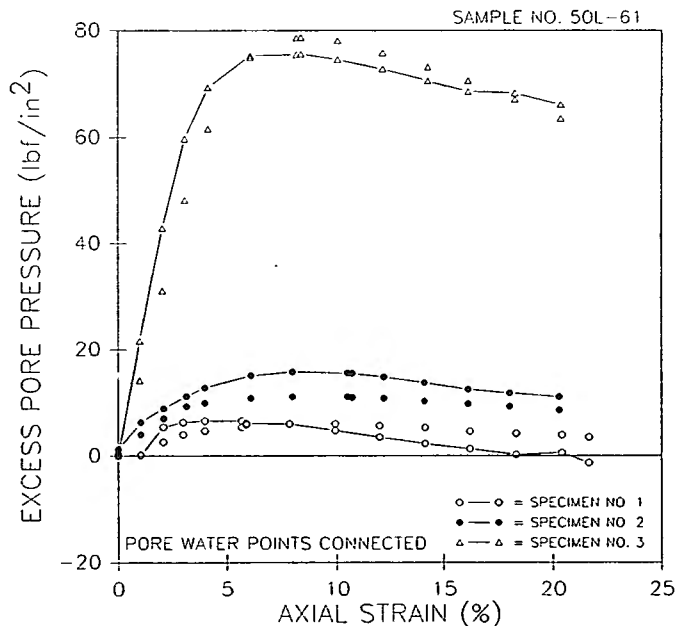
Figure 12. — Percent axial strain versus excess pore pressure—example.
