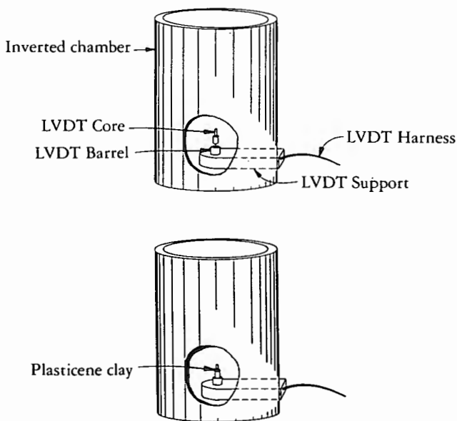
Figure 6. - LVDT placement in back pressure chamber cylinder.
