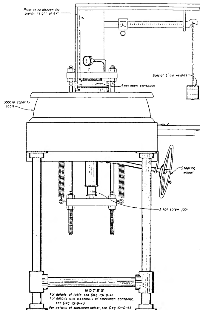
Figure 3. — Platform scale load frame with fixed-ring consolidometer in place. 101-D-40
