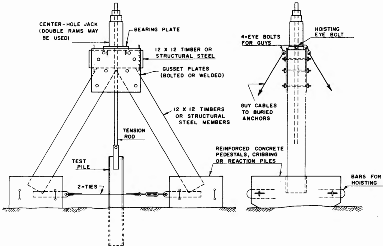
Figure 3. - Loading apparatus incorporating an A-frame. The A-frame may be guyed at various angles for testing batter piles or for special directional pull tests. Guy wires are used to stabilize the A-frame [ASTM D 3689].
