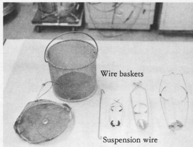
Figure 2. – Suspended mass in air and water assembly.
