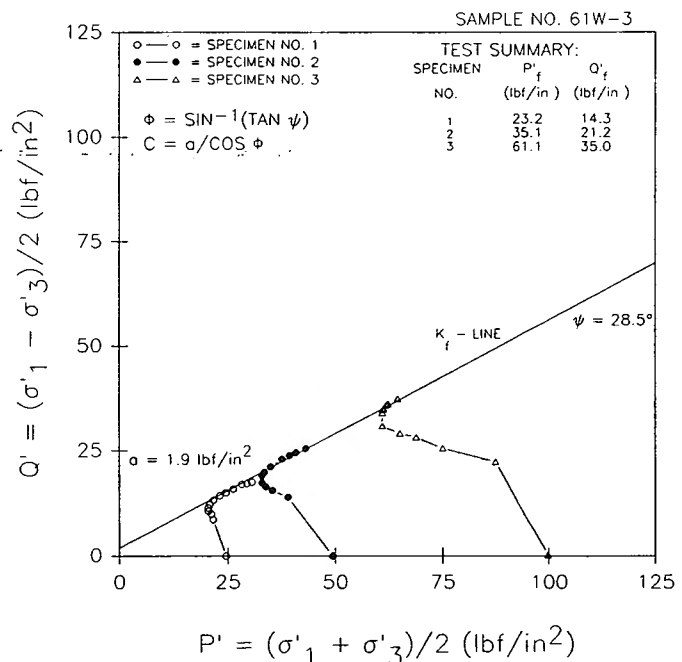
Figure 9. — p' - q' diagram—example.
