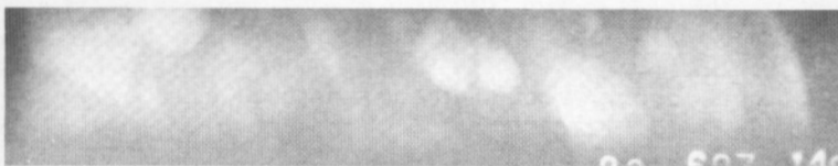
Figure 3. — X-ray radiograph showing gravel (lighter areas) in tube-type soil sample.
