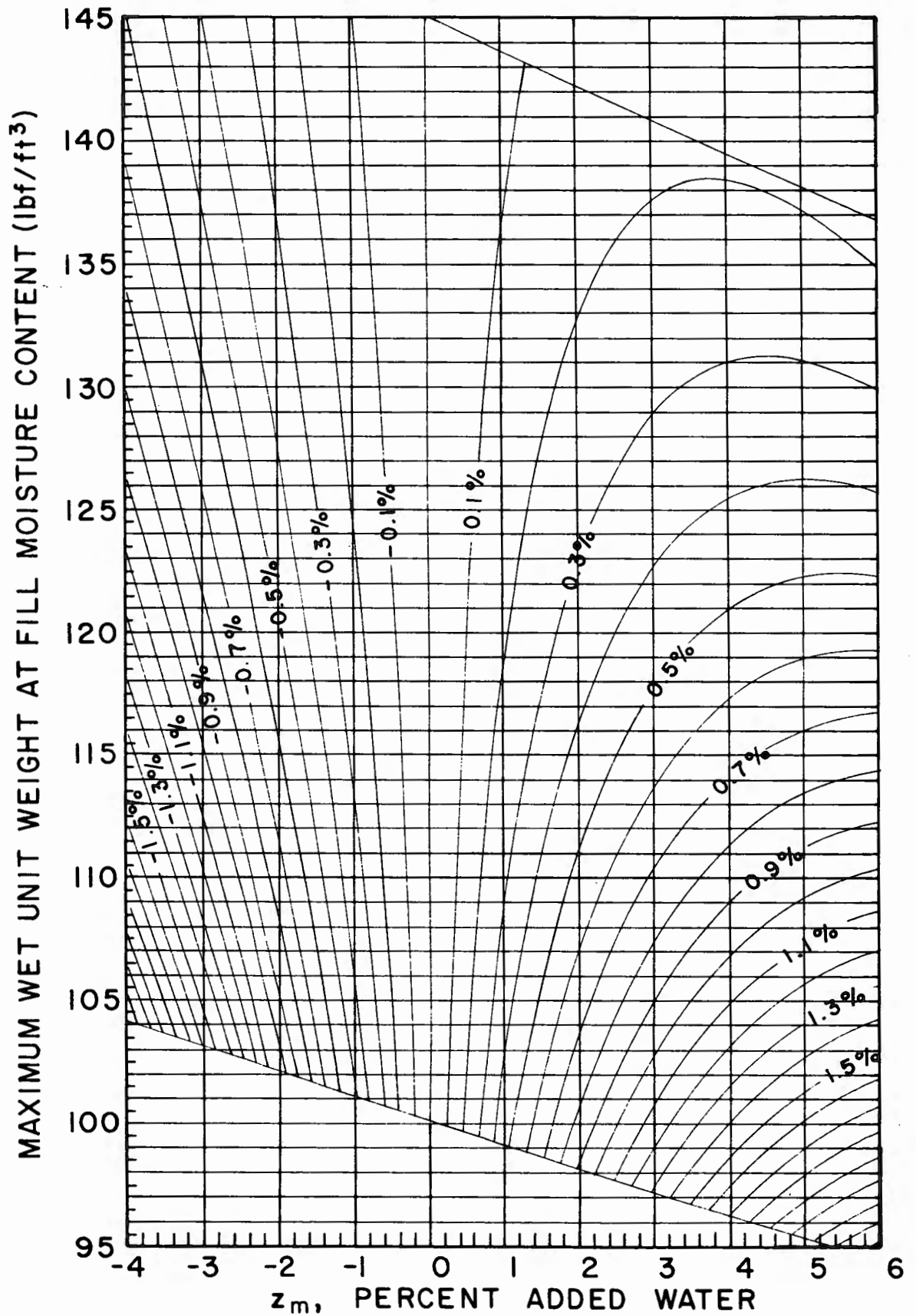
Figure X1.4. - Red-line correction — moisture adjustments values.
