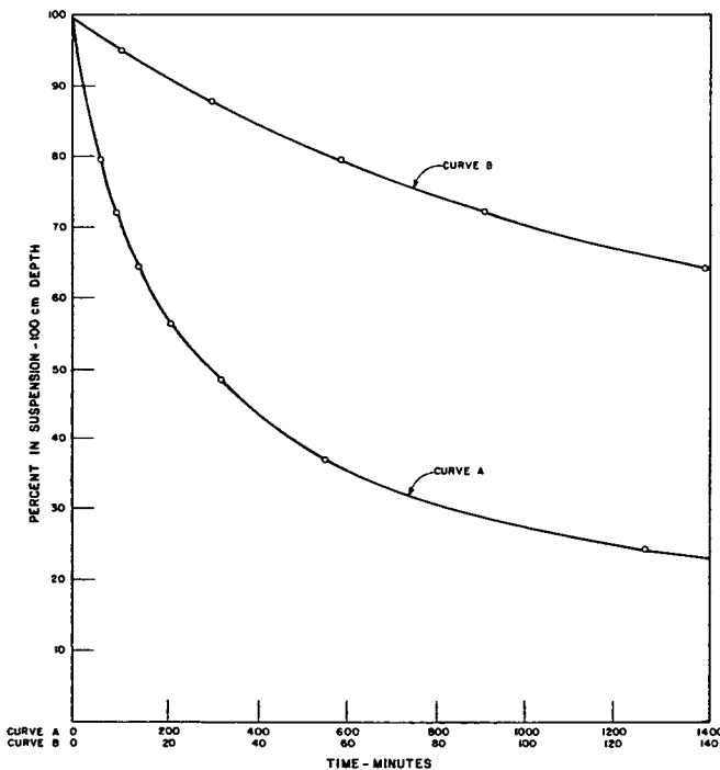
Figure X3.1 - Odén curve construction.
