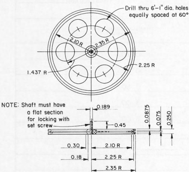
(a) Schematic of calibration wheel.
